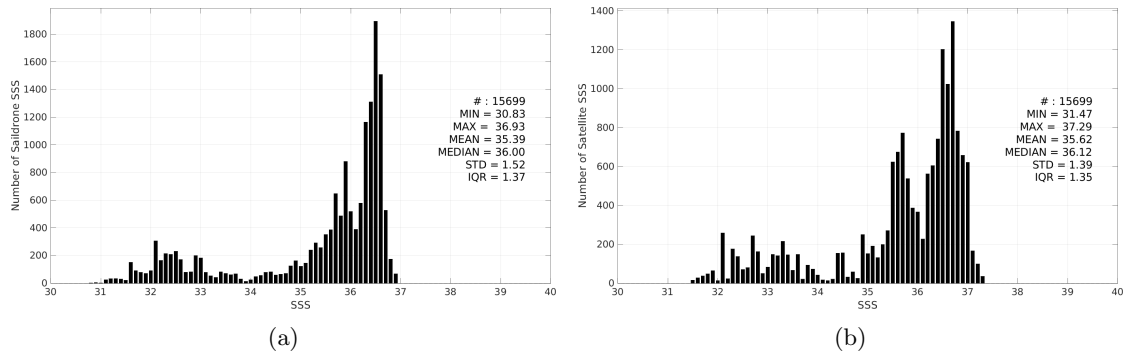
Figure 3: Histograms of SSS from Saildrone (a) and SMOS SSS L3 v335 - 10 Days - 25 km (CATDS-CPDC) (b) considering all match-up pairs per bins of 0.1 over the Gulf Stream Pi-MEP region and for the full satellite product period.
