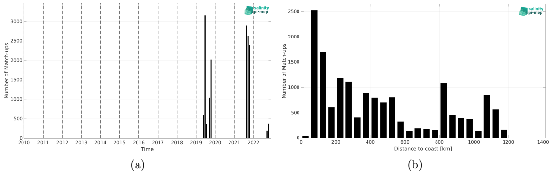
Figure 2: Number of match-ups between Saildrone and SMOS SSS L3 v335 - 10 Days - 25 km (CATDS-CPDC) SSS as a function of time (a) and as function of the distance to coast (b) over the Gulf Stream Pi-MEP region and for the full satellite product period.
