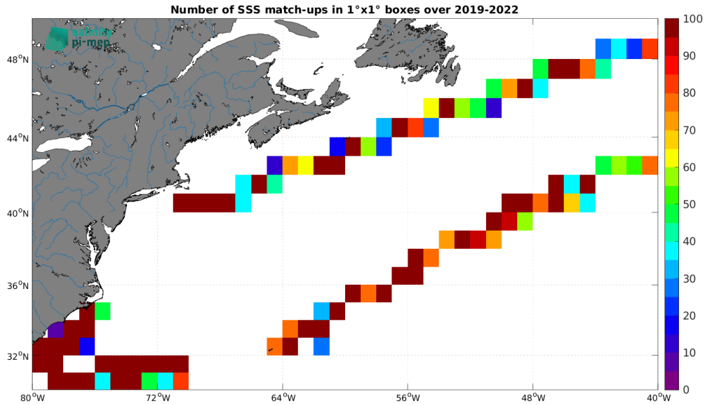
Figure 5: Number of SSS match-ups between Saildrone SSS and the SMOS SSS L3 v335 - 10 Days - 25 km (CATDS-CPDC) SSS product for the Gulf Stream Pi-MEP region over 1^\circ \times 1^\circ boxes and for the full satellite product period.
