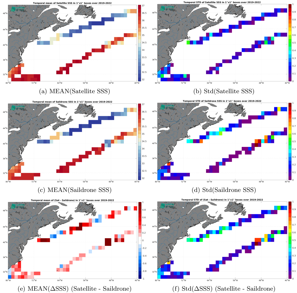
Figure 7: Temporal mean (left) and Std (right) of SSS from SMOS SSS L3 v335 - 10 Days - 25 km (CATDS-CPDC) (top), Saildrone (middle), and of \Delta SSS (Satellite - Saildrone). Only match-up pairs are used to generate these maps.
