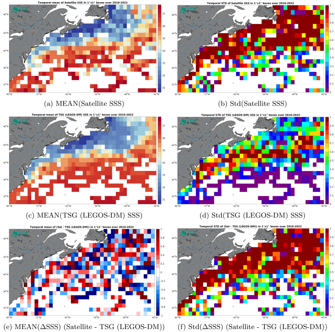
Figure 7: Temporal mean (left) and Std (right) of SSS from SMOS SSS L2Q v333 - 0.25 Deg (CATDS-CPDC) (top), TSG (LEGOS-DM) (middle), and of \Delta SSS (Satellite - TSG (LEGOS-DM)). Only match-up pairs are used to generate these maps.
