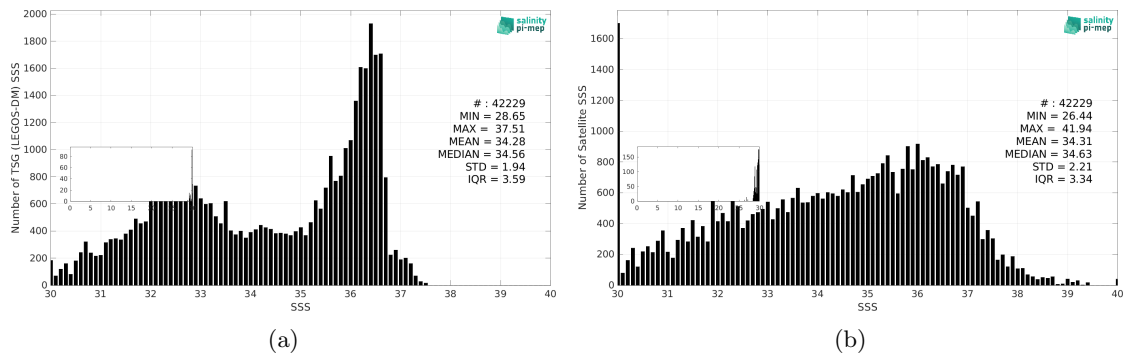
Figure 3: Histograms of SSS from TSG (LEGOS-DM) (a) and SMOS SSS L2Q v333 - 0.25 Deg (CATDS-CPDC) (b) considering all match-up pairs per bins of 0.1 over the Gulf Stream Pi-MEP region and for the full satellite product period.
