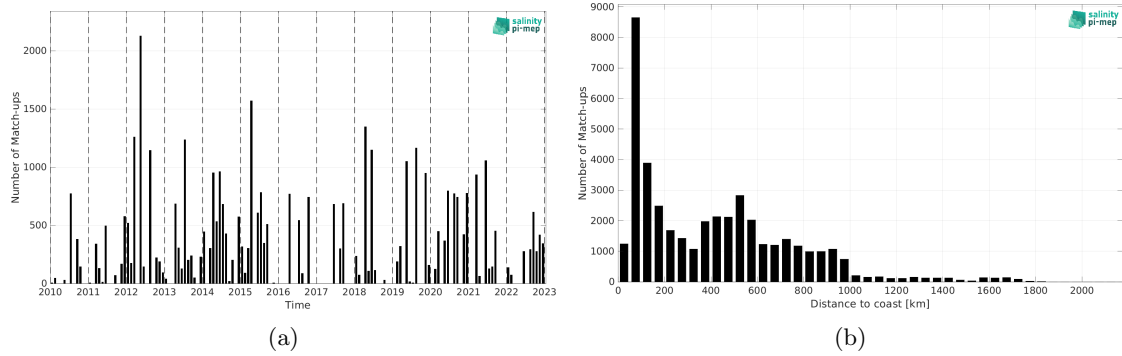
Figure 2: Number of match-ups between TSG (LEGOS-DM) and SMOS SSS L2Q v333 - 0.25 Deg (CATDS-CPDC) SSS as a function of time (a) and as function of the distance to coast (b) over the Gulf Stream Pi-MEP region and for the full satellite product period.
