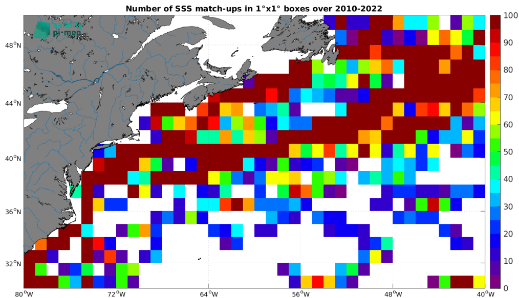
Figure 5: Number of SSS match-ups between TSG (LEGOS-DM) SSS and the SMOS SSS L2Q v333 - 0.25 Deg (CATDS-CPDC) SSS product for the Gulf Stream Pi-MEP region over 1^\circ \times 1^\circ boxes and for the full satellite product period.
