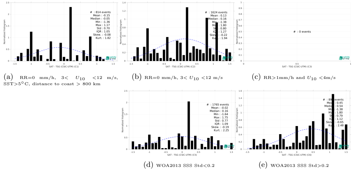
Figure 15: Normalized histogram of \Delta SSS (SMOS SSS L2Q v333 - 0.25 Deg (CATDS-CPDC) - TSG (CSIC-UTM)) for 5 different subdatasets corresponding to: RR=0 mm/h, 3 < U_{10} < 12 m/s, SST > 5°C, distance to coast > 800 km (a), RR=0 mm/h, 3 < U_{10} < 12 m/s (b), RR > 1mm/h and U_{10} < 4 m/s (c), WOA2013 SSS Std < 0.2 (d), WOA2013 SSS Std > 0.2 (e).
