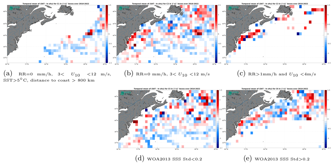
Figure 14: Temporal mean gridded over spatial boxes of size 1^\circ \times 1^\circ of \Delta SSS (SMOS SSS L3 v332 - 9 Days (CATDS-CPDC) - TSG (LEGOS-DM)) for 5 different subdatasets corresponding to: RR=0 mm/h, 3 < U_{10} < 12 m/s, SST > 5°C, distance to coast > 800 km (a), RR=0 mm/h, 3 < U_{10} < 12 m/s (b), RR > 1mm/h and U_{10} < 4 m/s (c), WOA2013 SSS Std < 0.2 (d), WOA2013 SSS Std > 0.2 (e).
