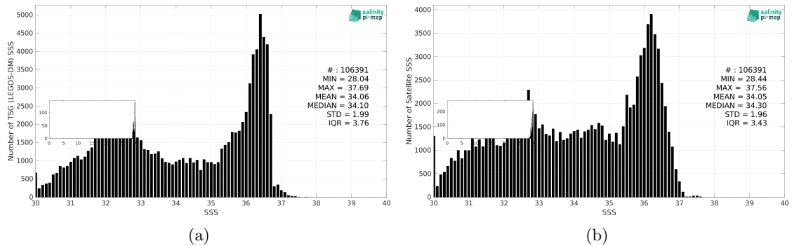
Figure 3: Histograms of SSS from TSG (LEGOS-DM) (a) and SMOS SSS L3 v332 - 9 Days (CATDS-CPDC) (b) considering all match-up pairs per bins of 0.1 over the Gulf Stream Pi-MEP region and for the full satellite product period.
