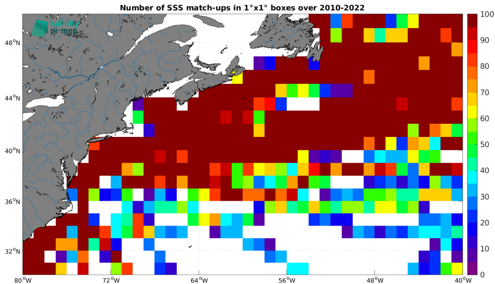
Figure 5: Number of SSS match-ups between TSG (LEGOS-DM) SSS and the SMOS SSS L3 v332 - 9 Days (CATDS-CPDC) SSS product for the Gulf Stream Pi-MEP region over 1°×1° boxes and for the full satellite product period.
