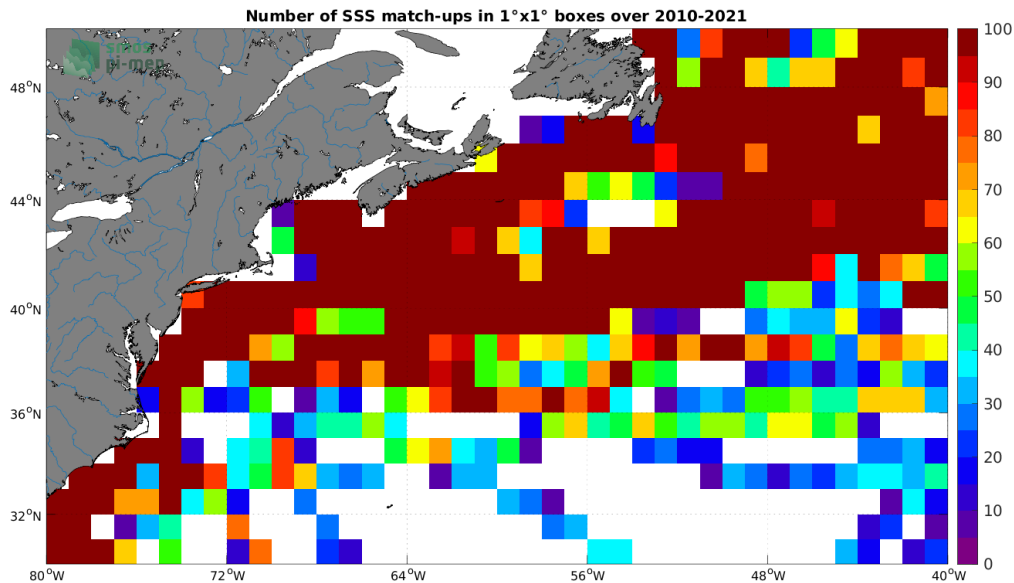
Figure 4: Number of SSS match-ups between TSG (LEGOS-DM) SSS and the SMOS SSS L3 v332 - 9 Days (CATDS-CPDC) SSS product for the Gulf Stream Pi-MEP region over 1^\circ \times 1^\circ boxes and for the full satellite product period.
