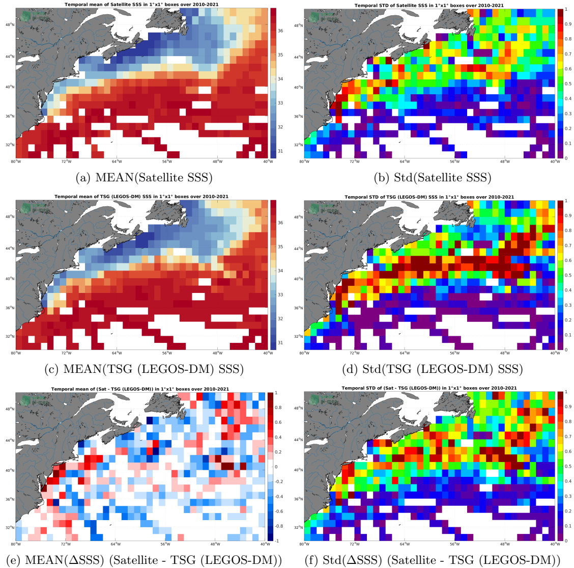
Figure 6: Temporal mean (left) and Std (right) of SSS from SMOS SSS L3 v332 - 9 Days (CATDS-CPDC) (top), TSG (LEGOS-DM) (middle), and of \Delta SSS (Satellite - TSG (LEGOS-DM)). Only match-up pairs are used to generate these maps.
