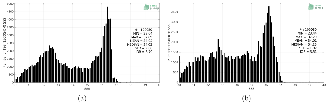
Figure 2: Histograms of SSS from TSG (LEGOS-DM) (a) and SMOS SSS L3 v332 - 9 Days (CATDS-CPDC) (b) considering all match-up pairs per bins of 0.1 over the Gulf Stream Pi-MEP region and for the full satellite product period.
