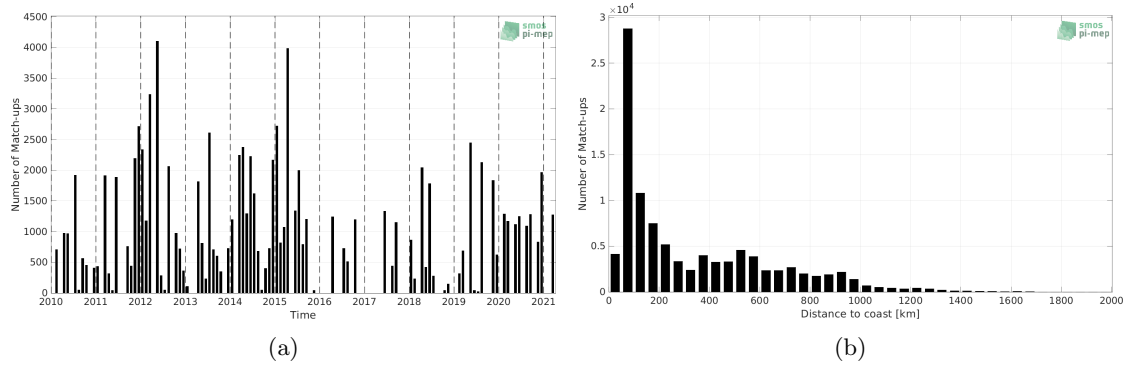
Figure 1: Number of match-ups between TSG (LEGOS-DM) and SMOS SSS L3 v332 - 9 Days (CATDS-CPDC) SSS as a function of time (a) and as function of the distance to coast (b) over the Gulf Stream Pi-MEP region and for the full satellite product period.
