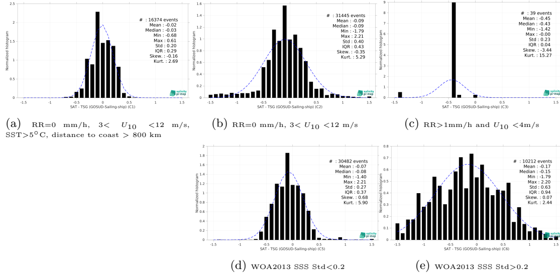
Figure 15: Normalized histogram of \Delta SSS (SMOS SSS L3 v332 - 9 Days (CATDS-CPDC) - TSG (GOSUD-Sailing-ship)) for 5 different subdatasets corresponding to: RR=0 mm/h, 3 < U_{10} < 12 m/s, SST>5°C, distance to coast > 800 km (a), RR=0 mm/h, 3 < U_{10} < 12 m/s (b), RR>1mm/h and U_{10} < 4 m/s (c), WOA2013 SSS Std<0.2 (d), WOA2013 SSS Std>0.2 (e).
