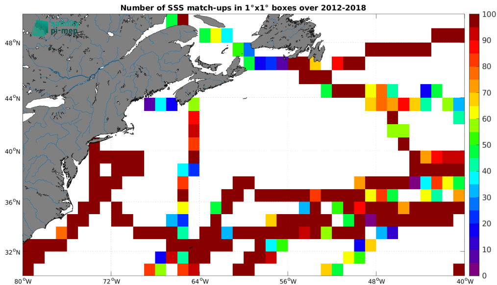
Figure 5: Number of SSS match-ups between TSG (GOSUD-Sailing-ship) SSS and the SMOS SSS L3 v332 - 9 Days (CATDS-CPDC) SSS product for the Gulf Stream Pi-MEP region over 1^\circ \times 1^\circ boxes and for the full satellite product period.
