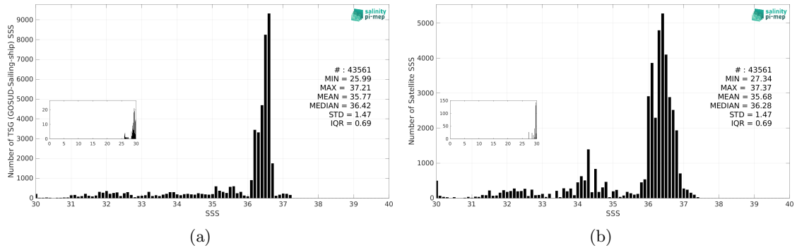
Figure 3: Histograms of SSS from TSG (GOSUD-Sailing-ship) (a) and SMOS SSS L3 v332 - 9 Days (CATDS-CPDC) (b) considering all match-up pairs per bins of 0.1 over the Gulf Stream Pi-MEP region and for the full satellite product period.
