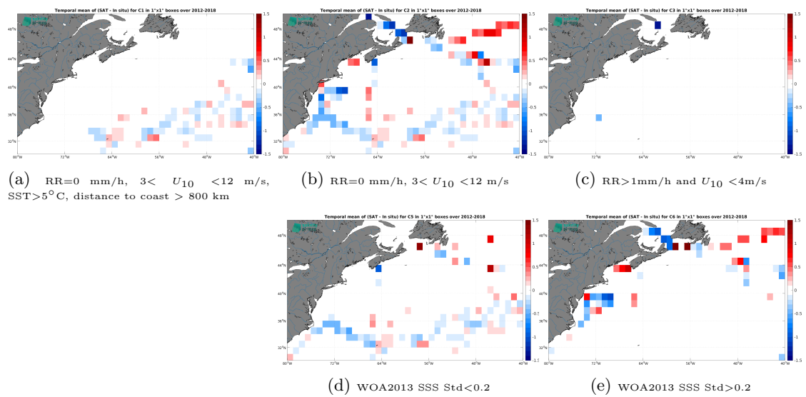
Figure 14: Temporal mean gridded over spatial boxes of size 1^\circ \times 1^\circ of \Delta SSS (SMOS SSS L3 v332 - 9 Days (CATDS-CPDC) - TSG (GOSUD-Sailing-ship)) for 5 different subdatasets corresponding to: RR=0 mm/h, 3 < U_{10} < 12 m/s, SST > 5°C, distance to coast > 800 km (a), RR=0 mm/h, 3 < U_{10} < 12 m/s (b), RR > 1mm/h and U_{10} < 4 m/s (c), WOA2013 SSS Std < 0.2 (d), WOA2013 SSS Std > 0.2 (e).
