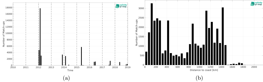
Figure 2: Number of match-ups between TSG (GOSUD-Sailing-ship) and SMOS SSS L3 v332 - 9 Days (CATDS-CPDC) SSS as a function of time (a) and as function of the distance to coast (b) over the Gulf Stream Pi-MEP region and for the full satellite product period.
