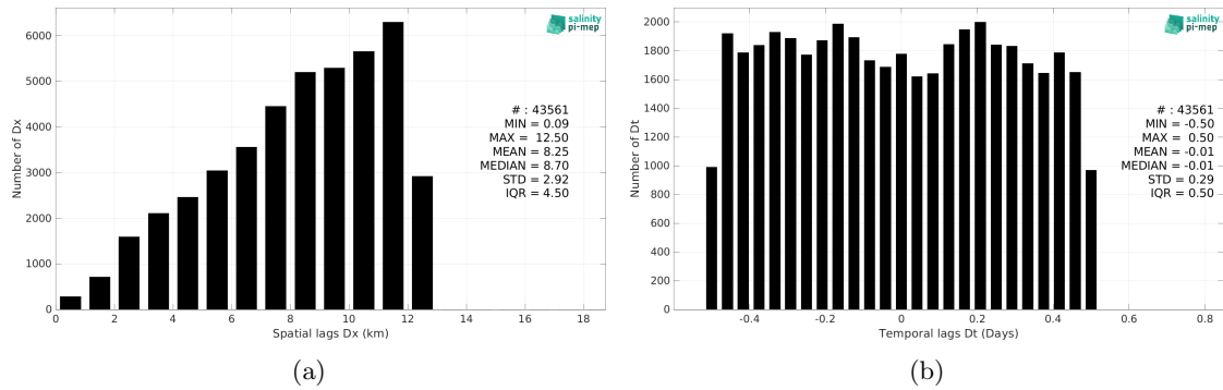
Figure 6: Histograms of the spatial (a) and temporal (b) lags between the location/time of the TSG (GOSUD-Sailing-ship) measurement and the date of the corresponding SMOS SSS L3 v332 - 9 Days (CATDS-CPDC) SSS pixel.
