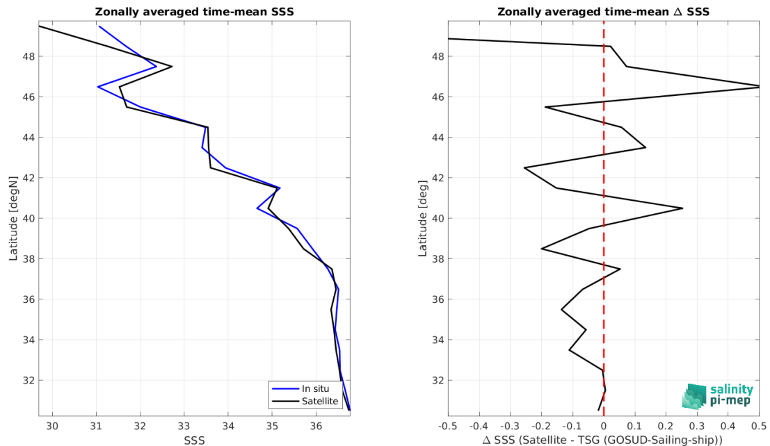
Figure 9: Left panel: Zonal mean SSS from SMOS SSS L3 v332 - 9 Days (CATDS-CPDC) satellite product (black) and from TSG (GOSUD-Sailing-ship) (blue). Right panel: Zonal mean of \Delta SSS (Satellite - TSG (GOSUD-Sailing-ship)) for all the collected Pi-MEP match-up pairs estimated over the full satellite product period.
