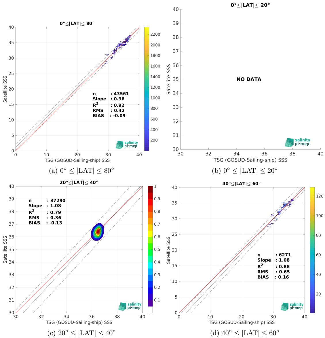
Figure 10: Contour maps of the concentration of SMOS SSS L3 v332 - 9 Days (CATDS-CPDC) SSS (y-axis) versus TSG (GOSUD-Sailing-ship) SSS (x-axis) at match-up pairs for different latitude bands. For each plot, the red line shows x=y . The black thin and dashed lines indicate a linear fit through the data cloud and the \pm 95\% confidence levels, respectively. The number match-up pairs n , the slope and R^2 coefficient of the linear fit, the root mean square (RMS) and the mean bias between satellite and in situ data are indicated for each latitude band in each plots.
