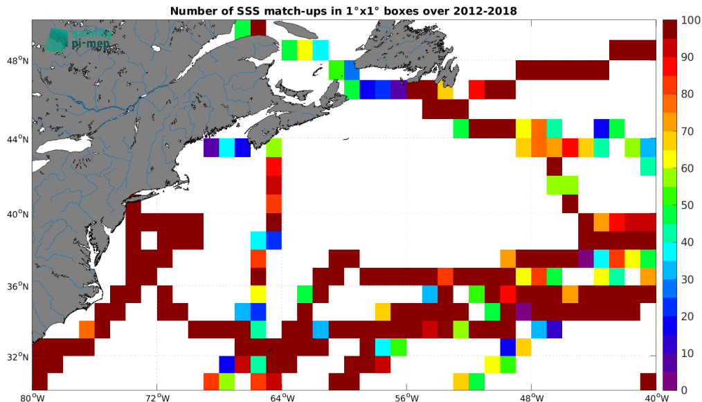
Figure 4: Number of SSS match-ups between TSG (GOSUD-Sailing-ship) SSS and the SMOS SSS L3 v332 - 9 Days (CATDS-CPDC) SSS product for the Gulf Stream Pi-MEP region over 1^\circ \times 1^\circ boxes and for the full satellite product period.
