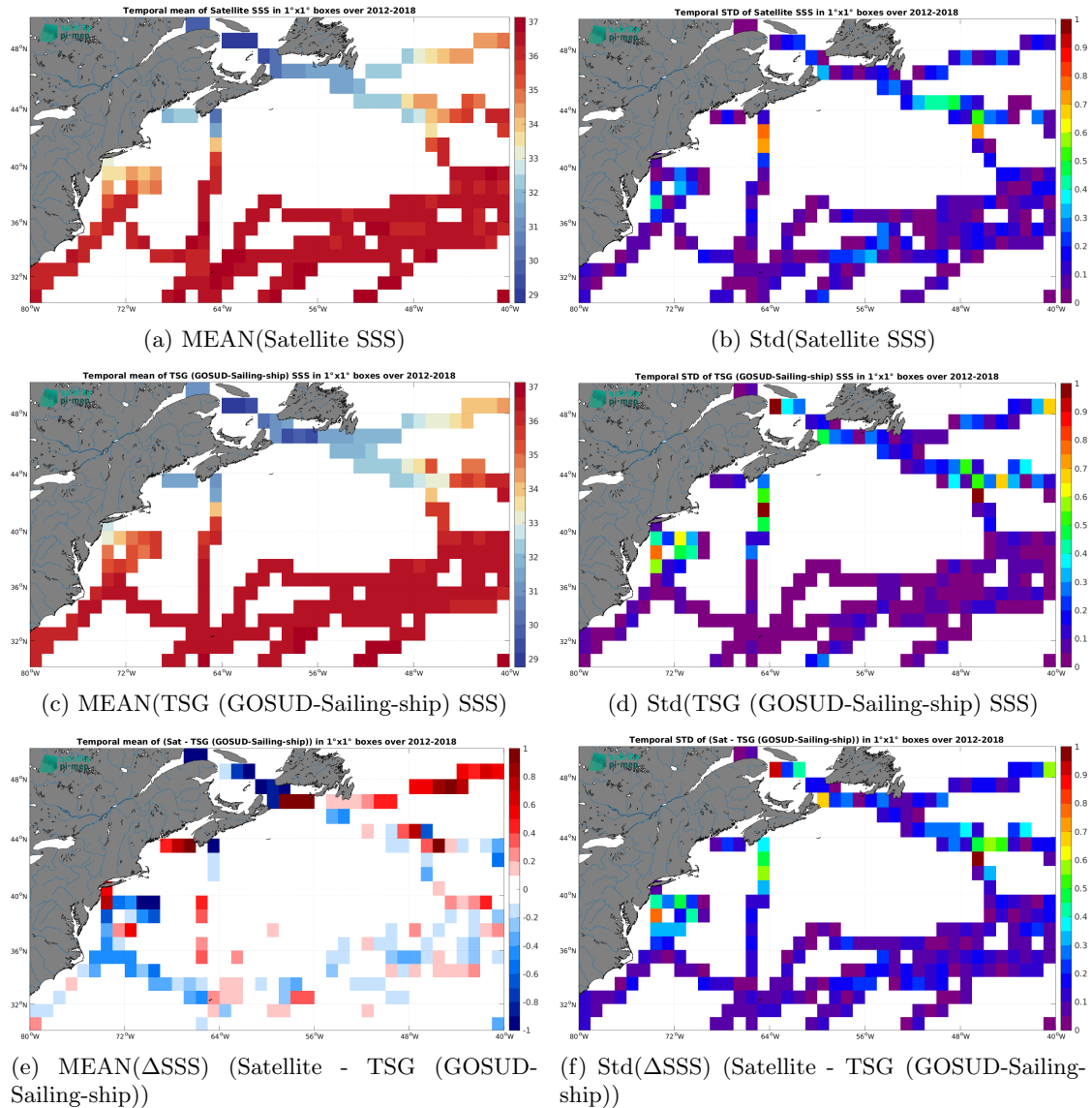
Figure 6: Temporal mean (left) and Std (right) of SSS from SMOS SSS L3 v332 - 9 Days (CATDS-CPDC) (top), TSG (GOSUD-Sailing-ship) (middle), and of \Delta SSS (Satellite - TSG (GOSUD-Sailing-ship)). Only match-up pairs are used to generate these maps.
