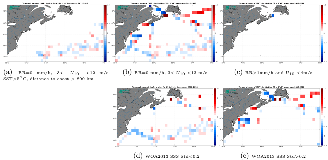
Figure 12: Temporal mean gridded over spatial boxes of size 1^{\circ}\times 1^{\circ} of \Delta SSS (SMOS SSS L3 v332 - 9 Days (CATDS-CPDC) - TSG (GOSUD-Sailing-ship)) for 5 different subdatasets corresponding to:RR=0 mm/h, 3 < U_{10} < 12 m/s, SST > 5^{\circ}\text{C} , distance to coast > 800 km (a), RR=0 mm/h, 3 < U_{10} < 12 m/s (b), RR > 1 mm/h and U_{10} < 4 m/s (c), WOA2013 SSS Std < 0.2 (d), WOA2013 SSS Std > 0.2 (e).
