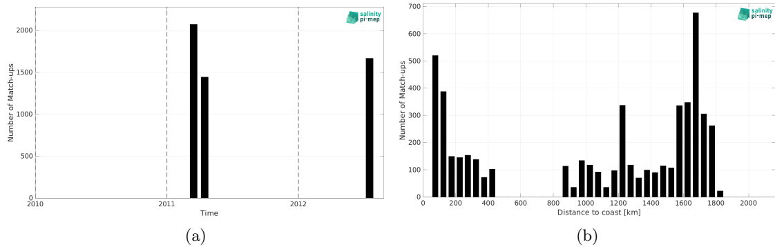
Figure 2: Number of match-ups between TSG (CSIC-UTM) and SMOS SSS L3 v332 - 9 Days (CATDS-CPDC) SSS as a function of time (a) and as function of the distance to coast (b) over the Gulf Stream Pi-MEP region and for the full satellite product period.
