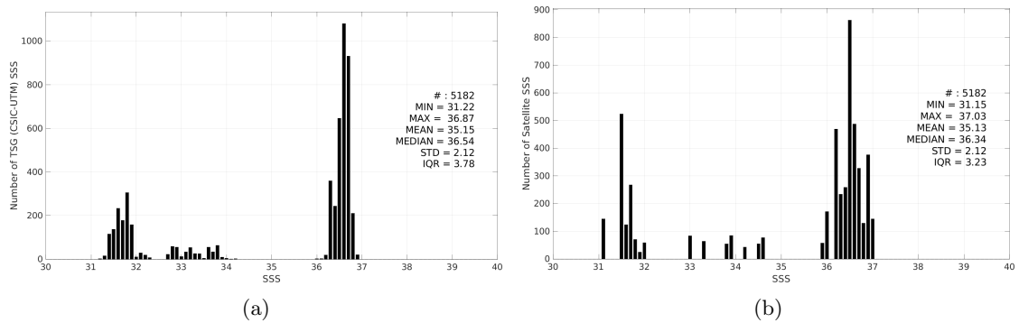
Figure 3: Histograms of SSS from TSG (CSIC-UTM) (a) and SMOS SSS L3 v332 - 9 Days (CATDS-CPDC) (b) considering all match-up pairs per bins of 0.1 over the Gulf Stream Pi-MEP region and for the full satellite product period.
