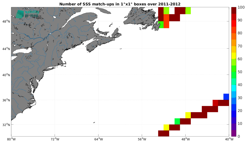
Figure 5: Number of SSS match-ups between TSG (CSIC-UTM) SSS and the SMOS SSS L3 v332 - 9 Days (CATDS-CPDC) SSS product for the Gulf Stream Pi-MEP region over 1^\circ \times 1^\circ boxes and for the full satellite product period.
