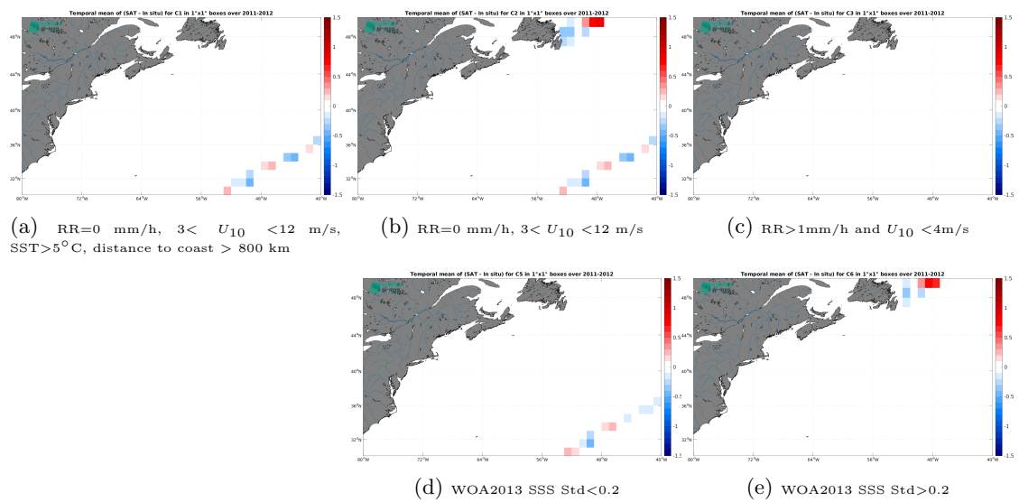
Figure 14: Temporal mean gridded over spatial boxes of size 1^\circ \times 1^\circ of \Delta SSS (SMOS SSS L3 v332 - 9 Days (CATDS-CPDC) - TSG (CSIC-UTM)) for 5 different subdatasets corresponding to: RR=0 mm/h, 3 < U_{10} < 12 m/s, SST > 5°C, distance to coast > 800 km (a), RR=0 mm/h, 3 < U_{10} < 12 m/s (b), RR > 1mm/h and U_{10} < 4 m/s (c), WOA2013 SSS Std < 0.2 (d), WOA2013 SSS Std > 0.2 (e).
