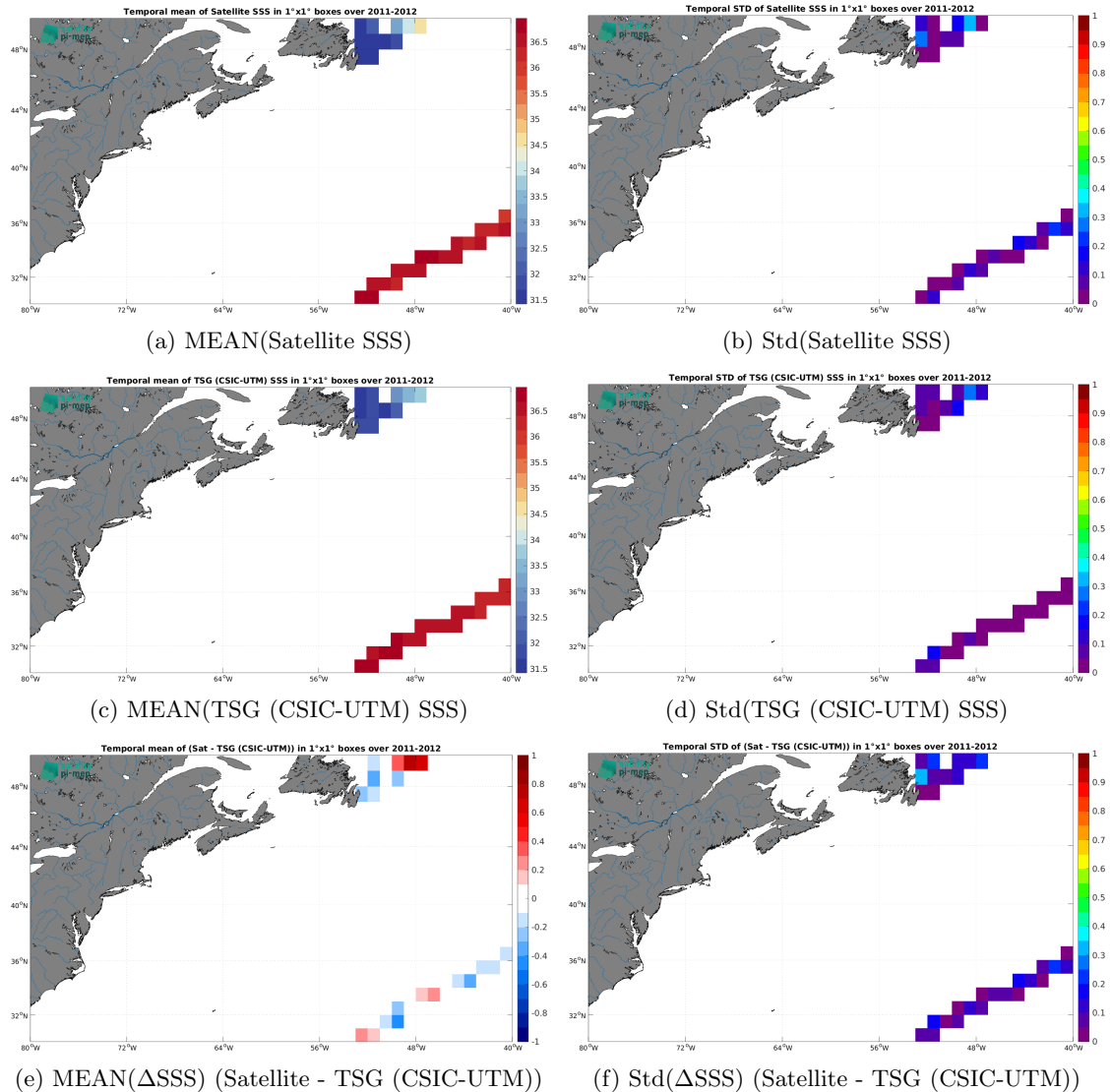
Figure 7: Temporal mean (left) and Std (right) of SSS from SMOS SSS L3 v332 - 9 Days (CATDS-CPDC) (top), TSG (CSIC-UTM) (middle), and of \Delta SSS (Satellite - TSG (CSIC-UTM)). Only match-up pairs are used to generate these maps.
