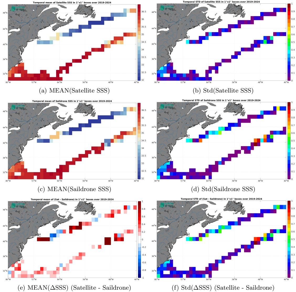
Figure 7: Temporal mean (left) and Std (right) of SSS from SMOS SSS L3 v332 - 9 Days (CATDS-CPDC) (top), Saildrone (middle), and of \Delta SSS (Satellite - Saildrone). Only match-up pairs are used to generate these maps.
