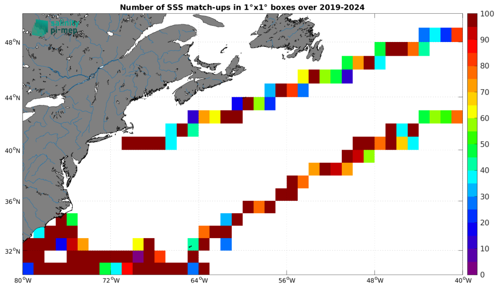
Figure 5: Number of SSS match-ups between Saildrone SSS and the SMOS SSS L3 v332 - 9 Days (CATDS-CPDC) SSS product for the Gulf Stream Pi-MEP region over 1^\circ \times 1^\circ boxes and for the full satellite product period.
