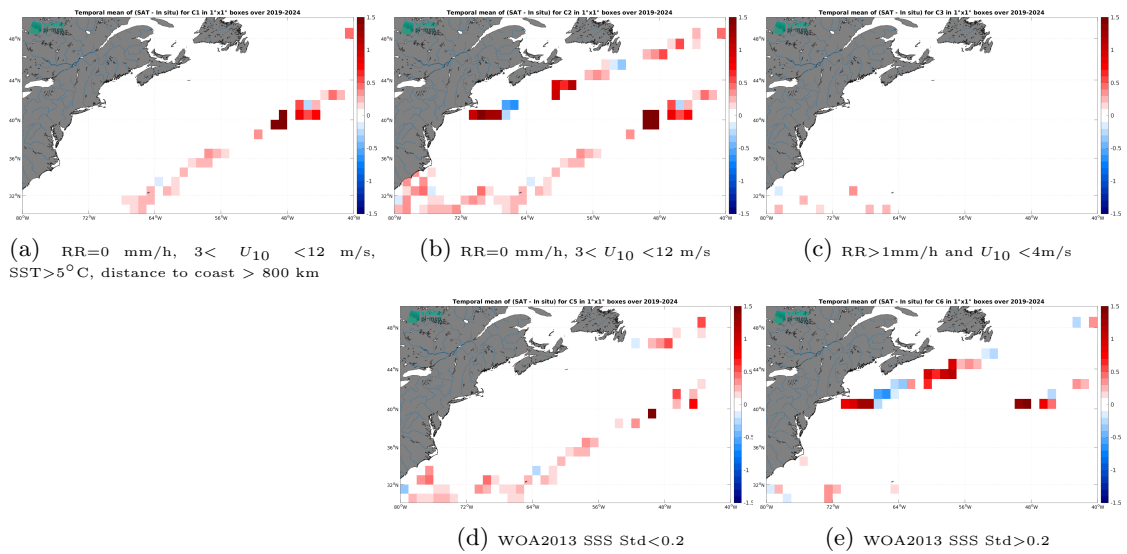
Figure 14: Temporal mean gridded over spatial boxes of size 1^\circ \times 1^\circ of \Delta SSS (SMOS SSS L3 v332 - 9 Days (CATDS-CPDC) - Sairdrone) for 5 different subdatasets corresponding to:RR=0 mm/h, 3 < U_{10} < 12 m/s, SST > 5^\circ C , distance to coast > 800 km (a), RR=0 mm/h, 3 < U_{10} < 12 m/s (b), RR>1mm/h and U_{10} < 4 m/s (c), WOA2013 SSS Std<0.2 (d), WOA2013 SSS Std>0.2 (e).
