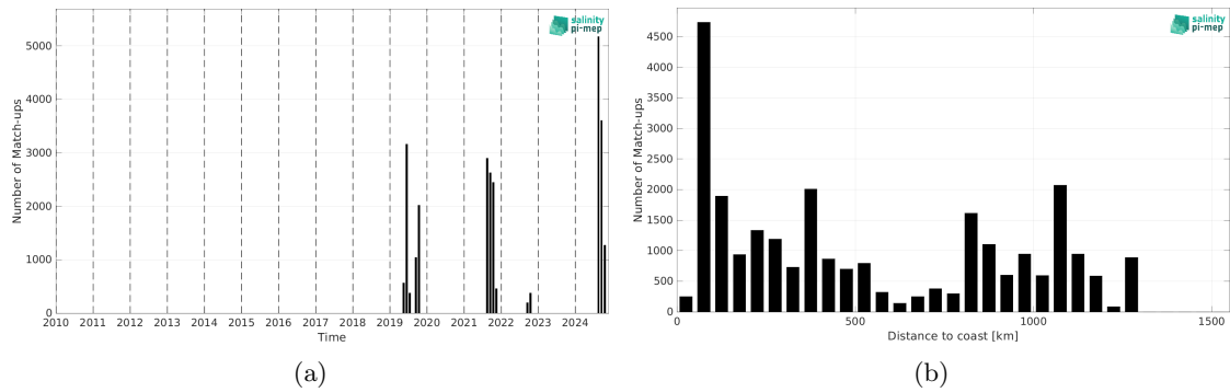
Figure 2: Number of match-ups between Saildrone and SMOS SSS L3 v332 - 9 Days (CATDS-CPDC) SSS as a function of time (a) and as function of the distance to coast (b) over the Gulf Stream Pi-MEP region and for the full satellite product period.
