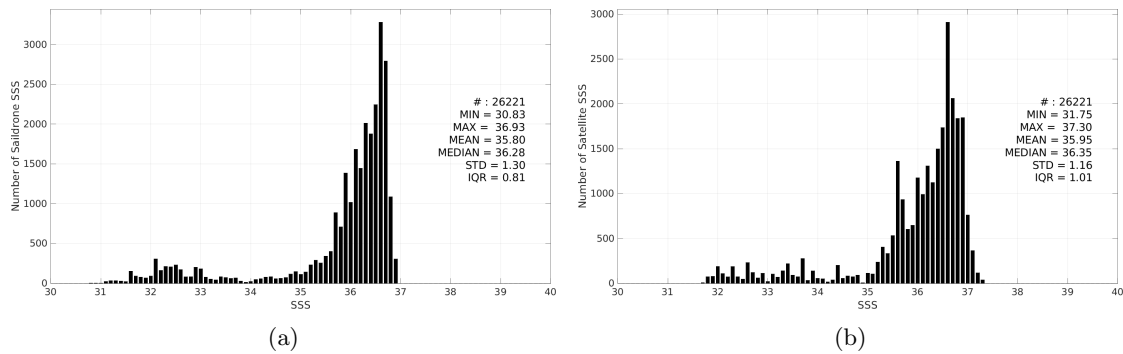
Figure 3: Histograms of SSS from Saildrone (a) and SMOS SSS L3 v332 - 9 Days (CATDS-CPDC) (b) considering all match-up pairs per bins of 0.1 over the Gulf Stream Pi-MEP region and for the full satellite product period.
