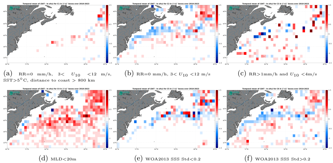
Figure 12: Temporal mean gridded over spatial boxes of size 1^\circ \times 1^\circ of \Delta SSS (SMOS SSS L3 v332 - 9 Days (CATDS-CPDC) - Argo) for 6 different subdatasets corresponding to:RR=0 mm/h, 3 < U_{10} < 12 m/s, SST > 5^\circ\text{C} , distance to coast > 800 km (a), RR=0 mm/h, 3 < U_{10} < 12 m/s (b), RR > 1 mm/h and U_{10} < 4 m/s (c),MLD < 20 m (d),WOA2013 SSS Std < 0.2 (e),WOA2013 SSS Std > 0.2 (f).
