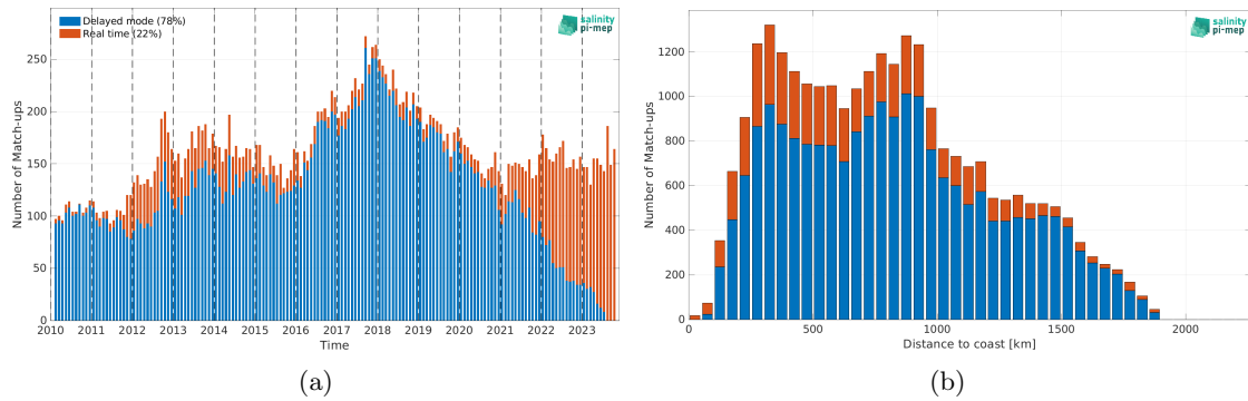
Figure 1: Number of match-ups between Argo and SMOS SSS L3 v332 - 9 Days (CATDS-CPDC) SSS as a function of time (a) and as function of the distance to coast (b) over the Gulf Stream Pi-MEP region and for the full satellite product period.
