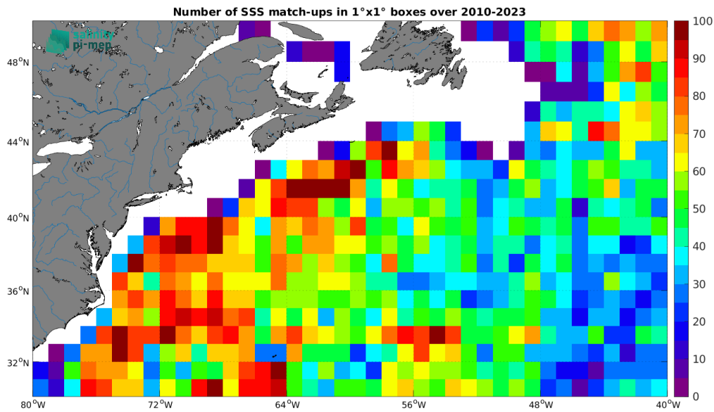
Figure 4: Number of SSS match-ups between Argo SSS and the SMOS SSS L3 v332 - 9 Days (CATDS-CPDC) SSS product for the Gulf Stream Pi-MEP region over 1^\circ \times 1^\circ boxes and for the full satellite product period.
