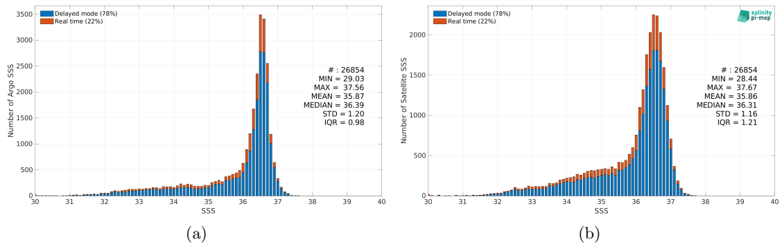
Figure 2: Histograms of SSS from Argo (a) and SMOS SSS L3 v332 - 9 Days (CATDS-CPDC) (b) considering all match-up pairs per bins of 0.1 over the Gulf Stream Pi-MEP region and for the full satellite product period.
