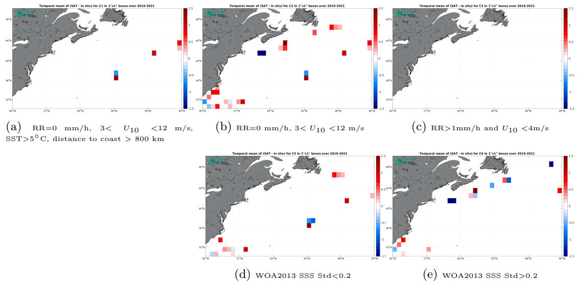
Figure 12: Temporal mean gridded over spatial boxes of size 1^\circ \times 1^\circ of \Delta SSS (SMOS SSS L2Q v331 - 0.25 Deg (CATDS-CPDC) - Sailydrone) for 5 different subdatasets corresponding to:RR=0 mm/h, 3 < U_{10} < 12 m/s, SST >5^\circ C, distance to coast > 800 km (a), RR=0 mm/h, 3 < U_{10} < 12 m/s (b), RR >1 mm/h and U_{10} < 4 m/s (c), WOA2013 SSS Std <0.2 (d), WOA2013 SSS Std >0.2 (e).
