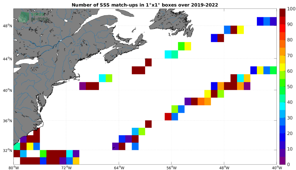
Figure 4: Number of SSS match-ups between Salldrone SSS and the SMOS SSS L2Q v331 - 0.25 Deg (CATDS-CPDC) SSS product for the Gulf Stream Pi-MEP region over 1^\circ \times 1^\circ boxes and for the full satellite product period.
