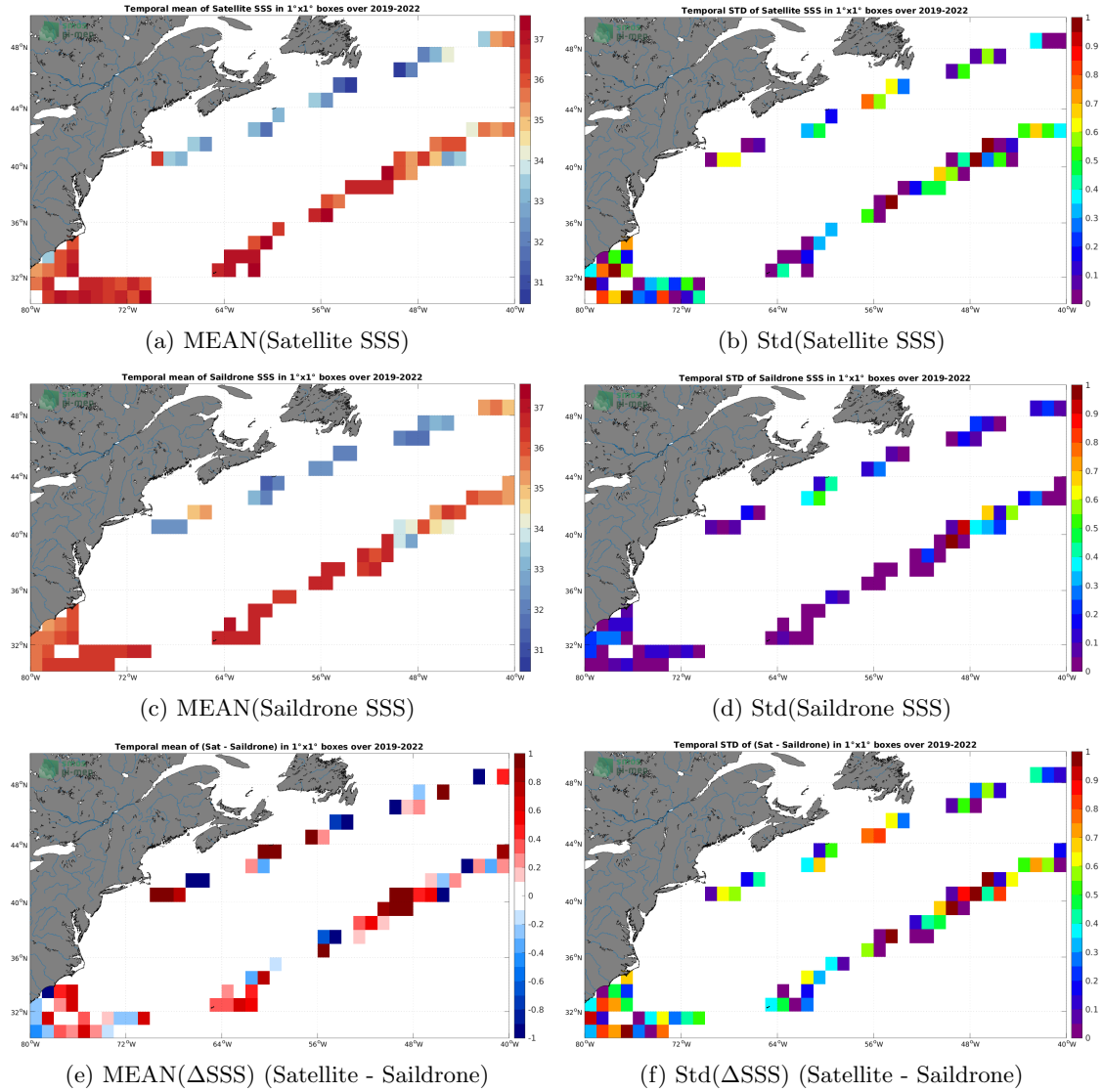
Figure 6: Temporal mean (left) and Std (right) of SSS from SMOS SSS L2Q v331 - 0.25 Deg (CATDS-CPDC) (top), Saildrone (middle), and of \Delta SSS (Satellite - Saildrone). Only match-up pairs are used to generate these maps.
