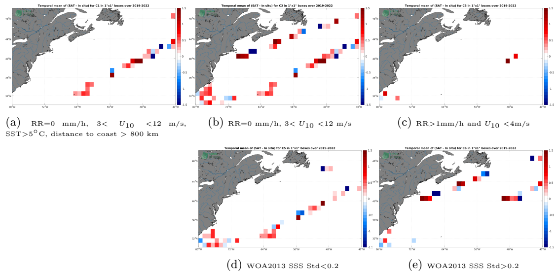
Figure 12: Temporal mean gridded over spatial boxes of size 1^\circ \times 1^\circ of \Delta SSS (SMOS SSS L2Q v331 - 0.25 Deg (CATDS-CPDC) - Saildrone) for 5 different subdatasets corresponding to:RR=0 mm/h, 3 < U_{10} < 12 m/s, SST >5^\circ C, distance to coast > 800 km (a), RR=0 mm/h, 3 < U_{10} < 12 m/s (b), RR >1 mm/h and U_{10} < 4 m/s (c), WOA2013 SSS Std <0.2 (d), WOA2013 SSS Std >0.2 (e).
