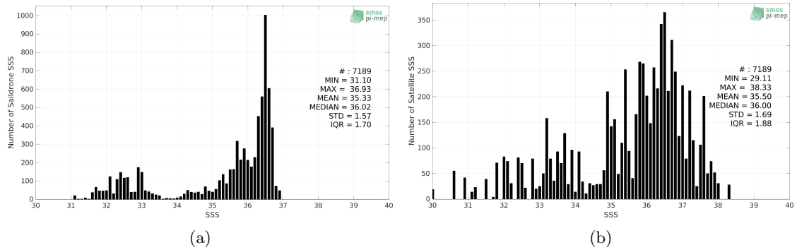
Figure 2: Histograms of SSS from Saildrone (a) and SMOS SSS L2Q v331 - 0.25 Deg (CATDS-CPDC) (b) considering all match-up pairs per bins of 0.1 over the Gulf Stream Pi-MEP region and for the full satellite product period.
