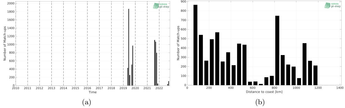
Figure 1: Number of match-ups between Saildrone and SMOS SSS L2Q v331 - 0.25 Deg (CATDS-CPDC) SSS as a function of time (a) and as function of the distance to coast (b) over the Gulf Stream Pi-MEP region and for the full satellite product period.
