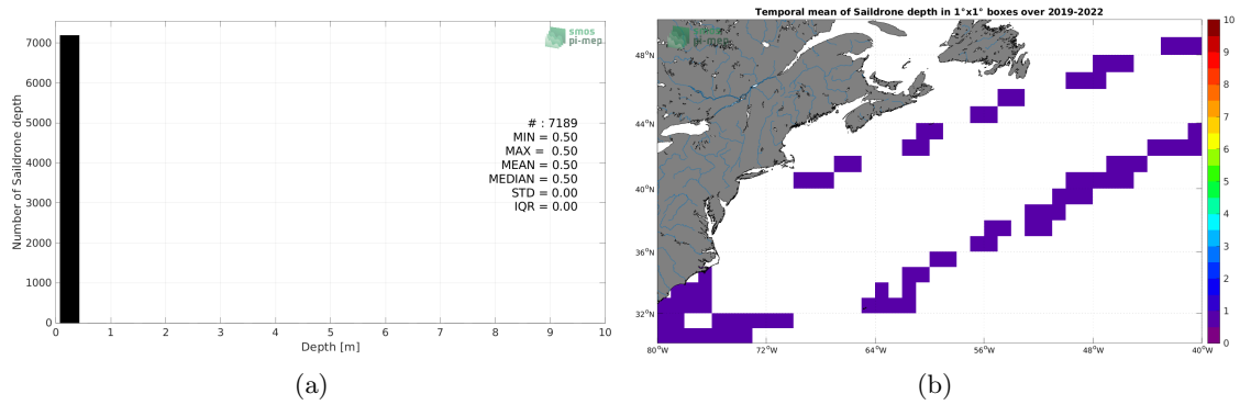
Figure 3: Histograms of the depth of the upper level SSS measurements from Salldrone in the Match-up DataBase for the Gulf Stream Pi-MEP region (a) and temporal mean spatial distribution of pressure of the in situ SSS data over 1^\circ \times 1^\circ boxes and for the full satellite product period (b).
