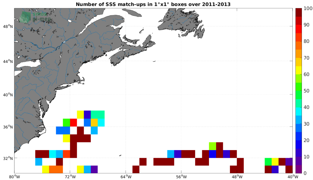
Figure 3: Number of SSS match-ups between Surface drifters SSS and the SMOS SSS L2Q v331 - 0.25 Deg (CATDS-CPDC) SSS product for the Gulf Stream Pi-MEP region over 1^\circ \times 1^\circ boxes and for the full satellite product period.
