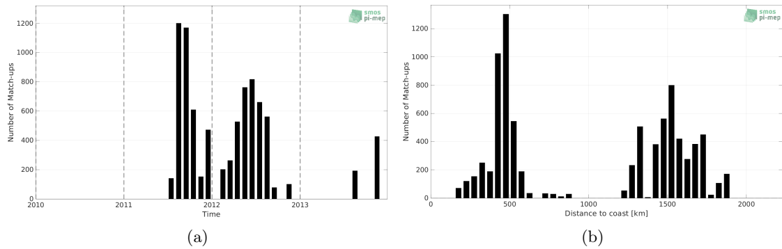
Figure 1: Number of match-ups between Surface drifters and SMOS SSS L2Q v331 - 0.25 Deg (CATDS-CPDC) SSS as a function of time (a) and as function of the distance to coast (b) over the Gulf Stream Pi-MEP region and for the full satellite product period.
