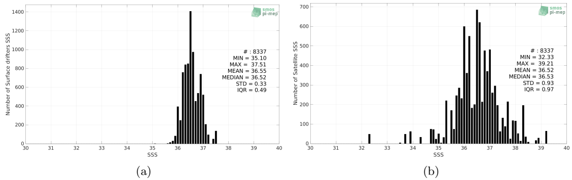
Figure 2: Histograms of SSS from Surface drifters (a) and SMOS SSS L2Q v331 - 0.25 Deg (CATDS-CPDC) (b) considering all match-up pairs per bins of 0.1 over the Gulf Stream Pi-MEP region and for the full satellite product period.
