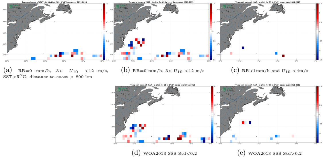
Figure 11: Temporal mean gridded over spatial boxes of size 1^{\circ}\times 1^{\circ} of \Delta\text{SSS} (SMOS SSS L2Q v331 - 0.25 Deg (CATDS-CPDC) - Surface drifters) for 5 different subdatasets corresponding to:RR=0 mm/h, 3 < U_{10} < 12 m/s, SST >5^{\circ}\text{C} , distance to coast > 800 km (a), RR=0 mm/h, 3 < U_{10} < 12 m/s (b), RR >1 mm/h and U_{10} < 4 m/s (c), WOA2013 SSS Std <0.2 (d), WOA2013 SSS Std >0.2 (e).
