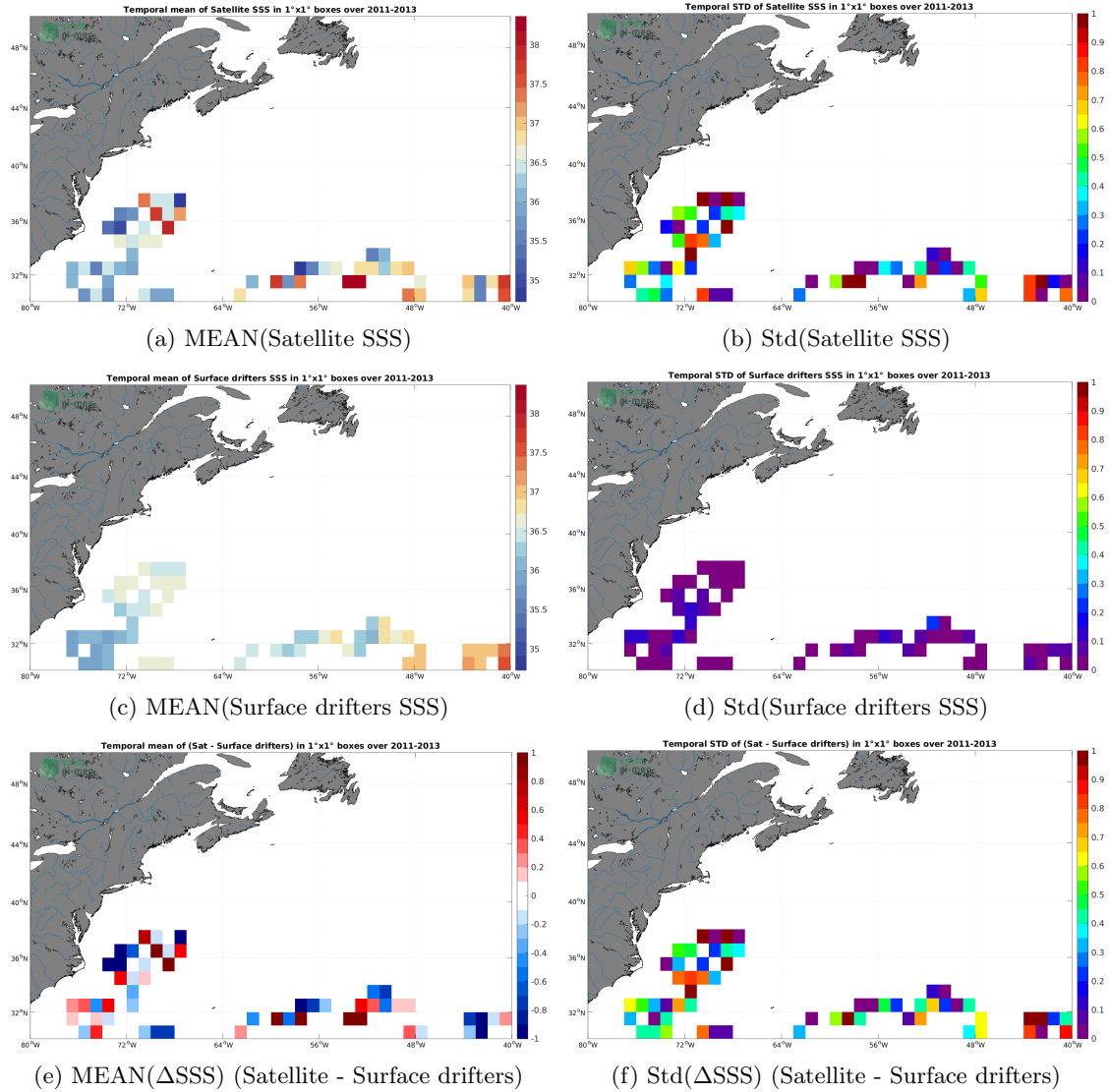
Figure 5: Temporal mean (left) and Std (right) of SSS from SMOS SSS L2Q v331 - 0.25 Deg (CATDS-CPDC) (top), Surface drifters (middle), and of \Delta SSS (Satellite - Surface drifters). Only match-up pairs are used to generate these maps.
