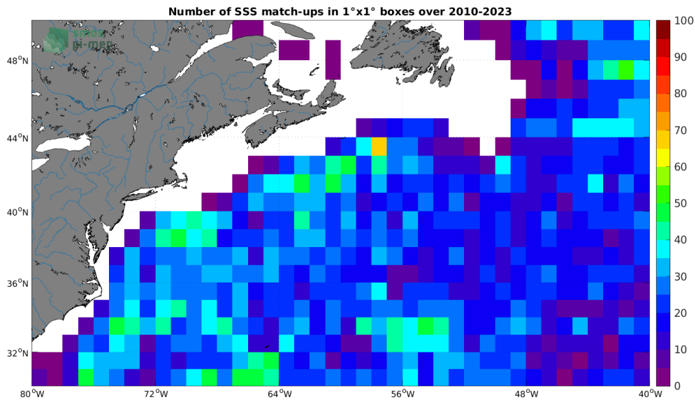
Figure 4: Number of SSS match-ups between Argo SSS and the SMOS SSS L2Q v331 - 0.25 Deg (CATDS-CPDC) SSS product for the Gulf Stream Pi-MEP region over 1^\circ \times 1^\circ boxes and for the full satellite product period.
