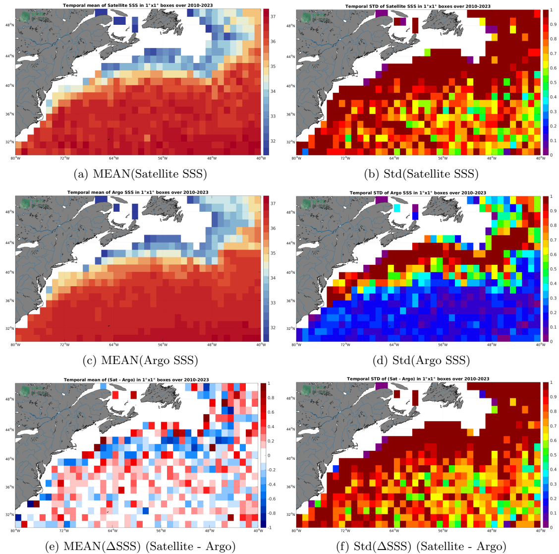
Figure 6: Temporal mean (left) and Std (right) of SSS from SMOS SSS L2Q v331 - 0.25 Deg (CATDS-CPDC) (top), Argo (middle), and of \Delta SSS (Satellite - Argo). Only match-up pairs are used to generate these maps.
