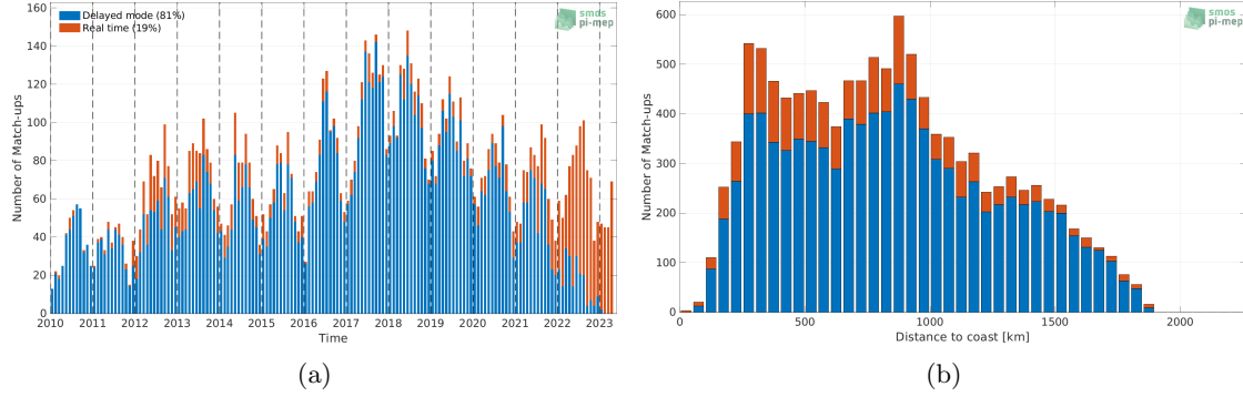
Figure 1: Number of match-ups between Argo and SMOS SSS L2Q v331 - 0.25 Deg (CATDS-CPDC) SSS as a function of time (a) and as function of the distance to coast (b) over the Gulf Stream Pi-MEP region and for the full satellite product period.
