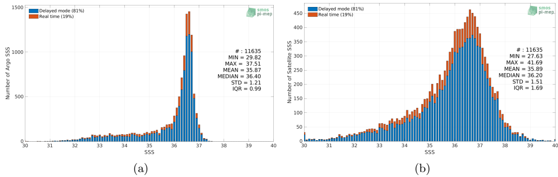
Figure 2: Histograms of SSS from Argo (a) and SMOS SSS L2Q v331 - 0.25 Deg (CATDS-CPDC) (b) considering all match-up pairs per bins of 0.1 over the Gulf Stream Pi-MEP region and for the full satellite product period.
