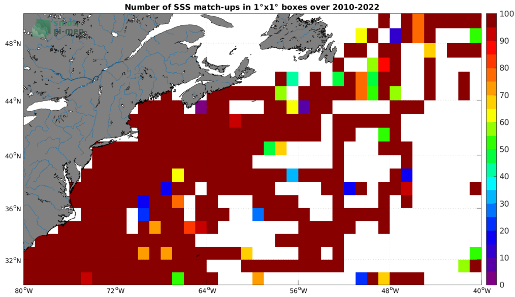
Figure 4: Number of SSS match-ups between TSG (SAMOS) SSS and the SMOS SSS L2Q v330 - 0.25 Deg (CATDS-CPDC) SSS product for the Gulf Stream Pi-MEP region over 1^\circ \times 1^\circ boxes and for the full satellite product period.
