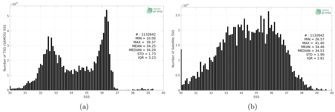
Figure 2: Histograms of SSS from TSG (SAMOS) (a) and SMOS SSS L2Q v330 - 0.25 Deg (CATDS-CPDC) (b) considering all match-up pairs per bins of 0.1 over the Gulf Stream Pi-MEP region and for the full satellite product period.
