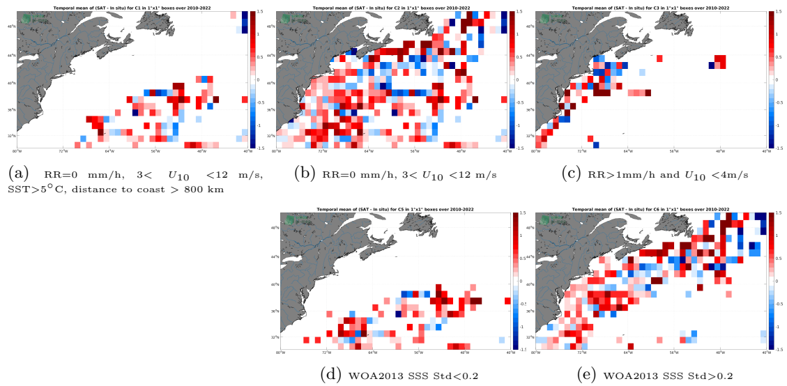
Figure 12: Temporal mean gridded over spatial boxes of size 1^\circ \times 1^\circ of \Delta SSS (SMOS SSS L2Q v330 - 0.25 Deg (CATDS-CPDC) - TSG (SAMOS)) for 5 different subdatasets corresponding to: RR=0 mm/h, 3 < U_{10} < 12 m/s, SST >5^\circ C, distance to coast > 800 km (a), RR=0 mm/h, 3 < U_{10} < 12 m/s (b), RR >1 mm/h and U_{10} < 4 m/s (c), WOA2013 SSS Std <0.2 (d), WOA2013 SSS Std >0.2 (e).
