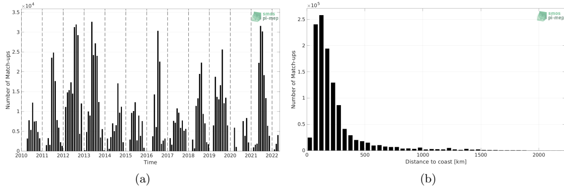
Figure 1: Number of match-ups between TSG (SAMOS) and SMOS SSS L2Q v330 - 0.25 Deg (CATDS-CPDC) SSS as a function of time (a) and as function of the distance to coast (b) over the Gulf Stream Pi-MEP region and for the full satellite product period.
