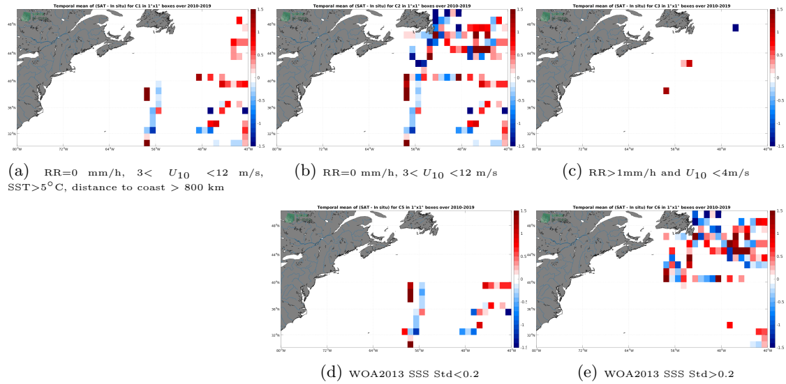
Figure 12: Temporal mean gridded over spatial boxes of size 1^{\circ}\times 1^{\circ} of \Delta SSS (SMOS SSS L2Q v330 - 0.25 Deg (CATDS-CPDC) - TSG (GOSUD-Research-vessel)) for 5 different subdatasets corresponding to:RR=0 mm/h, 3 < U_{10} < 12 m/s, SST > 5^{\circ}\text{C} , distance to coast > 800 km (a), RR=0 mm/h, 3 < U_{10} < 12 m/s (b), RR > 1 mm/h and U_{10} < 4 m/s (c), WOA2013 SSS Std < 0.2 (d), WOA2013 SSS Std > 0.2 (e).
