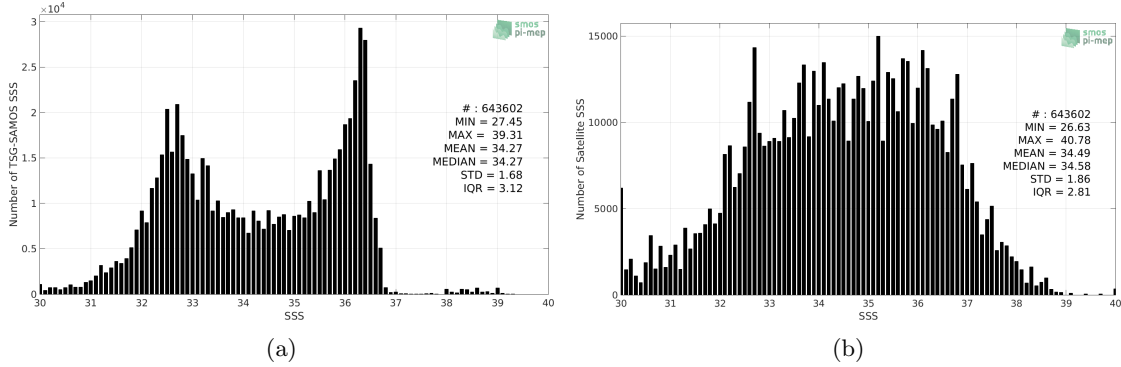
Figure 2: Histograms of SSS from TSG-SAMOS (a) and SMOS L2Q v321 - 0.25 Deg (CATDS-CPDC) (b) considering all match-up pairs per bins of 0.1 over the Gulf Stream Pi-MEP region and for the full satellite product period.
