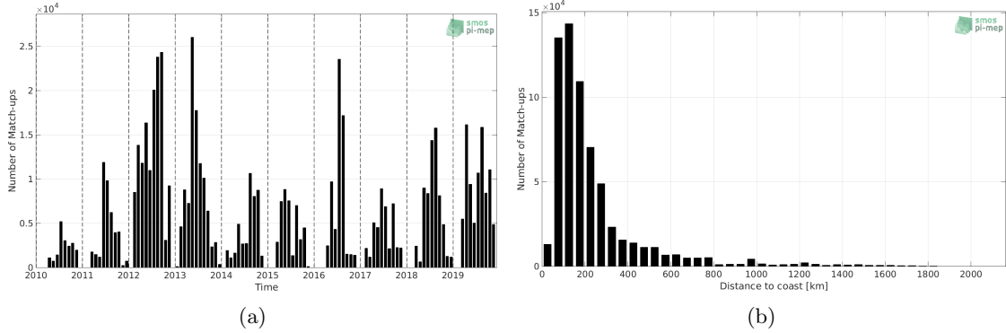
Figure 1: Number of match-ups between TSG-SAMOS and SMOS L2Q v321 - 0.25 Deg (CATDS-CPDC) SSS as a function of time (a) and as function of the distance to coast (b) over the Gulf Stream Pi-MEP region and for the full satellite product period.
