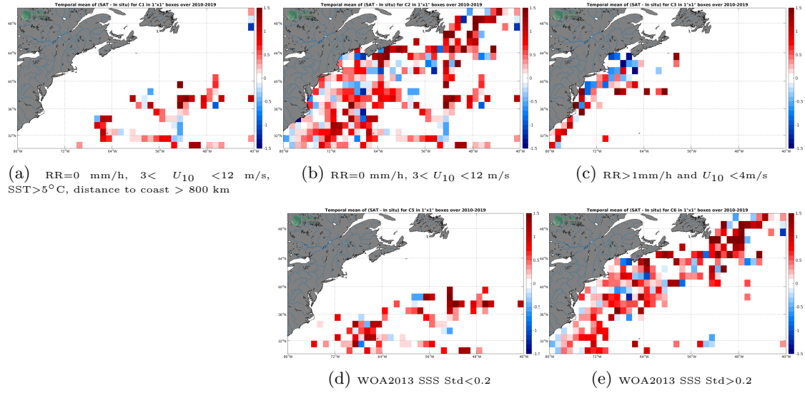
Figure 12: Temporal mean gridded over spatial boxes of size 1^\circ \times 1^\circ of \Delta SSS (SMOS L2Q v321 - 0.25 Deg (CATDS-CPDC) - TSG-SAMOS) for 5 different subdatasets corresponding to: RR=0 mm/h, 3 < U_{10} < 12 m/s, SST > 5^\circ C , distance to coast > 800 km (a), RR=0 mm/h, 3 < U_{10} < 12 m/s (b), RR > 1 mm/h and U_{10} < 4 m/s (c), WOA2013 SSS Std < 0.2 (d), WOA2013 SSS Std > 0.2 (e).
