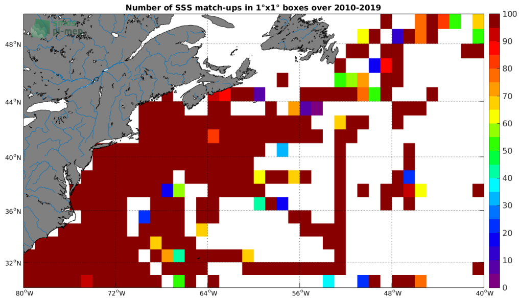
Figure 4: Number of SSS match-ups between TSG-SAMOS SSS and the SMOS L2Q v321 - 0.25 Deg (CATDS-CPDC) SSS product for the Gulf Stream Pi-MEP region over 1^\circ \times 1^\circ boxes and for the full satellite product period.
