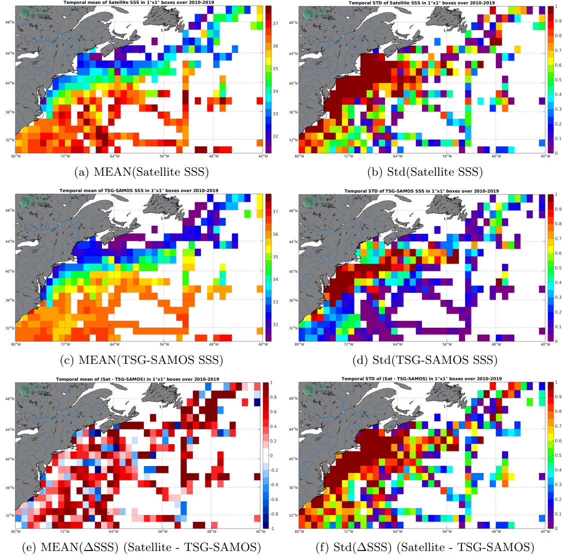
Figure 6: Temporal mean (left) and Std (right) of SSS from SMOS L2Q v321 - 0.25 Deg (CATDS-CPDC) (top), TSG-SAMOS (middle), and of \Delta SSS (Satellite - TSG-SAMOS). Only match-up pairs are used to generate these maps.
