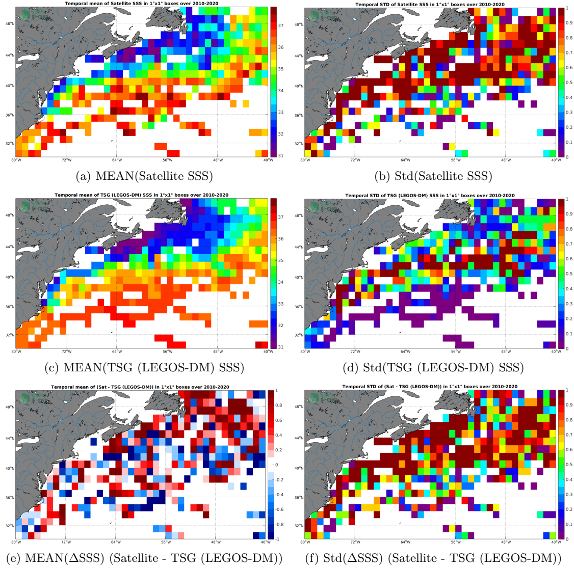
Figure 6: Temporal mean (left) and Std (right) of SSS from SMOS SSS L2Q v321 - 0.25 Deg (CATDS-CPDC) (top), TSG (LEGOS-DM) (middle), and of \Delta SSS (Satellite - TSG (LEGOS-DM)). Only match-up pairs are used to generate these maps.
