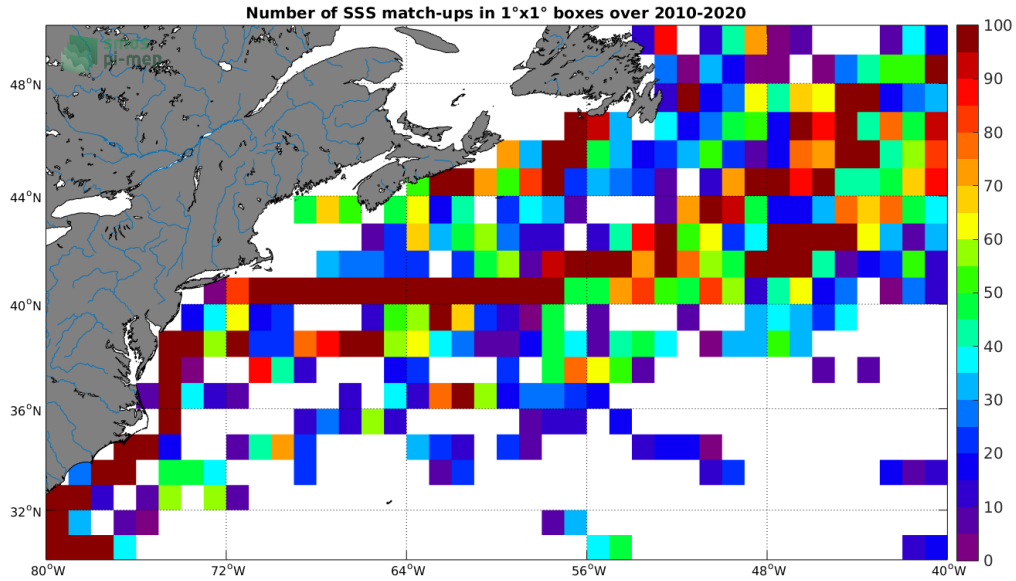
Figure 4: Number of SSS match-ups between TSG (LEGOS-DM) SSS and the SMOS SSS L2Q v321 - 0.25 Deg (CATDS-CPDC) SSS product for the Gulf Stream Pi-MEP region over 1^\circ \times 1^\circ boxes and for the full satellite product period.
