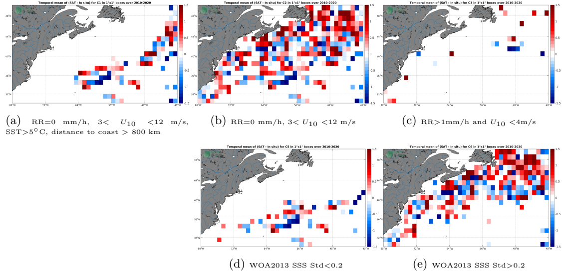
Figure 12: Temporal mean gridded over spatial boxes of size 1^{\circ}\times 1^{\circ} of \Delta\text{SSS} (SMOS SSS L2Q v321 - 0.25 Deg (CATDS-CPDC) - TSG (LEGOS-DM)) for 5 different subdatasets corresponding to: RR=0 mm/h, 3 < U_{10} < 12 m/s, SST >5^{\circ}\text{C} , distance to coast > 800 km (a), RR=0 mm/h, 3 < U_{10} < 12 m/s (b), RR >1 mm/h and U_{10} < 4 m/s (c), WOA2013 SSS Std <0.2 (d), WOA2013 SSS Std >0.2 (e).
