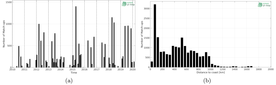
Figure 1: Number of match-ups between TSG (LEGOS-DM) and SMOS SSS L2Q v321 - 0.25 Deg (CATDS-CPDC) SSS as a function of time (a) and as function of the distance to coast (b) over the Gulf Stream Pi-MEP region and for the full satellite product period.
