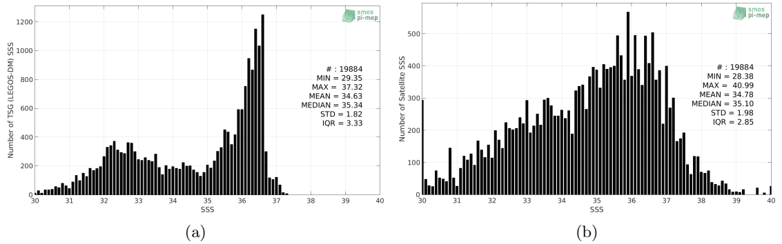
Figure 2: Histograms of SSS from TSG (LEGOS-DM) (a) and SMOS SSS L2Q v321 - 0.25 Deg (CATDS-CPDC) (b) considering all match-up pairs per bins of 0.1 over the Gulf Stream Pi-MEP region and for the full satellite product period.
