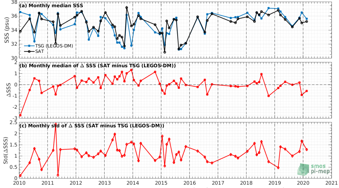
Figure 7: Time series of the monthly median SSS (top), median of \Delta\text{SSS} (Satellite - TSG (LEGOS-DM)) and Std of \Delta\text{SSS} (Satellite - TSG (LEGOS-DM)) over the Gulf Stream Pi-MEP region considering all match-ups collected by the Pi-MEP.
