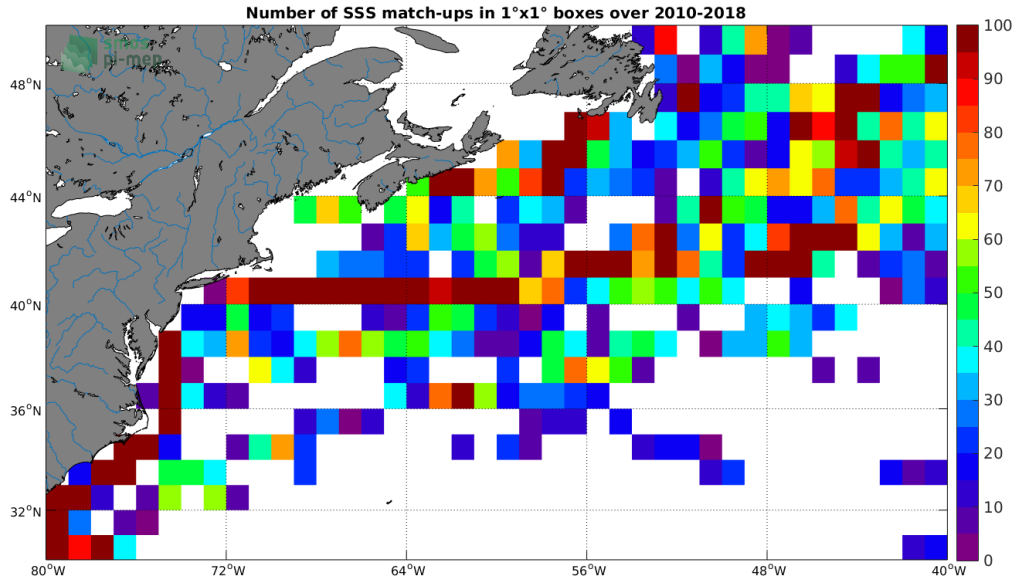
Figure 4: Number of SSS match-ups between TSG (LEGOS-DM) SSS and the SMOS SSS L2Q v321 - 0.25 Deg (CATDS-CPDC) SSS product for the Gulf Stream Pi-MEP region over 1°x1° boxes and for the full satellite product period.
