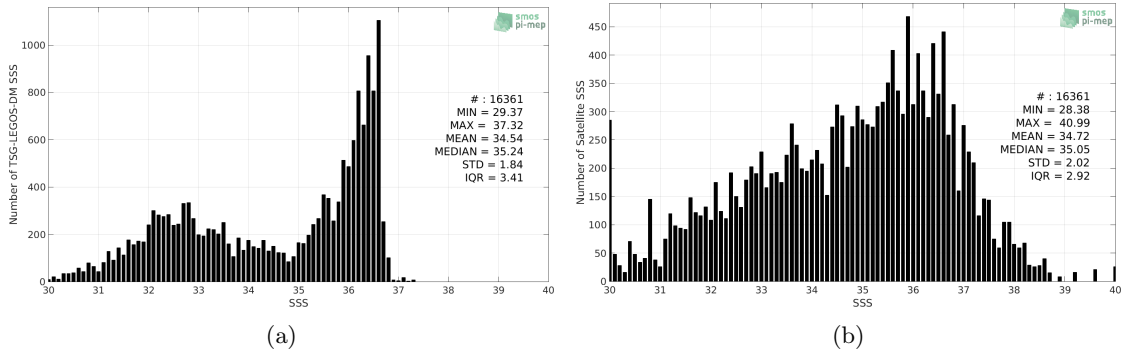
Figure 2: Histograms of SSS from TSG-LEGOS-DM (a) and SMOS L2Q v321 - 0.25 Deg (CATDS-CPDC) (b) considering all match-up pairs per bins of 0.1 over the Gulf Stream Pi-MEP region and for the full satellite product period.
