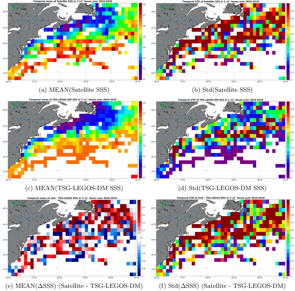
Figure 6: Temporal mean (left) and Std (right) of SSS from SMOS L2Q v321 - 0.25 Deg (CATDS-CPDC) (top), TSG-LEGOS-DM (middle), and of \Delta SSS (Satellite - TSG-LEGOS-DM). Only match-up pairs are used to generate these maps.
