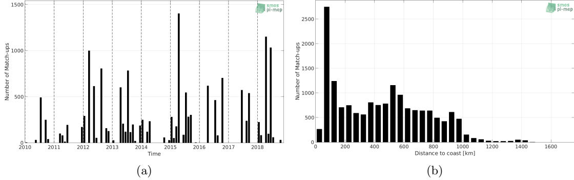
Figure 1: Number of match-ups between TSG-LEGOS-DM and SMOS L2Q v321 - 0.25 Deg (CATDS-CPDC) SSS as a function of time (a) and as function of the distance to coast (b) over the Gulf Stream Pi-MEP region and for the full satellite product period.
