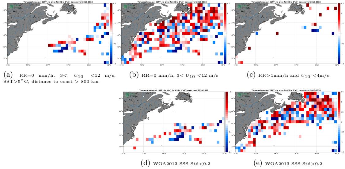
Figure 12: Temporal mean gridded over spatial boxes of size 1^\circ \times 1^\circ of \Delta SSS (SMOS L2Q v321 - 0.25 Deg (CATDS-CPDC) - TSG-LEGOS-DM) for 5 different subdatasets corresponding to: RR=0 mm/h, 3 < U_{10} < 12 m/s, SST > 5^\circ C , distance to coast > 800 km (a), RR=0 mm/h, 3 < U_{10} < 12 m/s (b), RR > 1 mm/h and U_{10} < 4 m/s (c), WOA2013 SSS Std < 0.2 (d), WOA2013 SSS Std > 0.2 (e).
