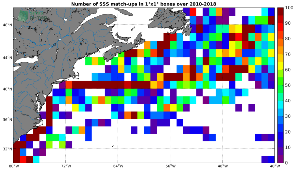
Figure 4: Number of SSS match-ups between TSG-LEGOS-DM SSS and the SMOS L2Q v321 - 0.25 Deg (CATDS-CPDC) SSS product for the Gulf Stream Pi-MEP region over 1°x1° boxes and for the full satellite product period.
