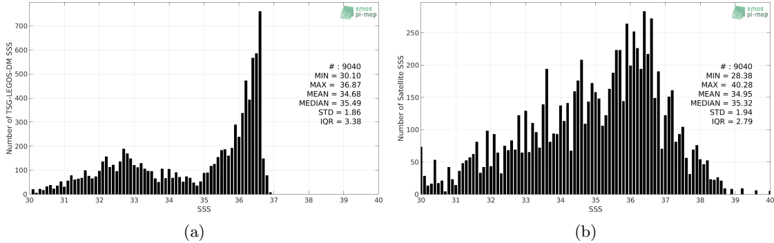
Figure 2: Histograms of SSS from TSG-LEGOS-DM (a) and SMOS-L3-CATDS-CPDC-V321-L2Q (b) considering all match-up pairs per bins of 0.1 over the Gulf Stream Pi-MEP region and for the full satellite product period.
