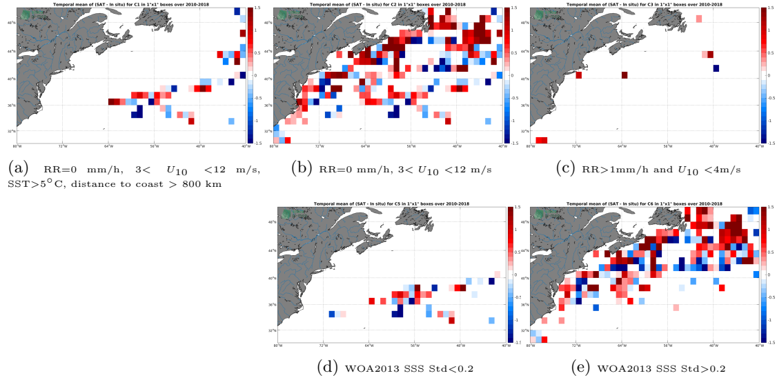
Figure 12: Temporal mean gridded over spatial boxes of size 1^\circ \times 1^\circ of \Delta SSS (SMOS-L3-CATDS-CPDC-V321-L2Q - TSG-LEGOS-DM) for 5 different subdatasets corresponding to: RR=0 mm/h, 3 < U_{10} < 12 m/s, SST > 5^\circ C , distance to coast > 800 km (a), RR=0 mm/h, 3 < U_{10} < 12 m/s (b), RR > 1 mm/h and U_{10} < 4 m/s (c), WOA2013 SSS Std < 0.2 (d), WOA2013 SSS Std > 0.2 (e).
