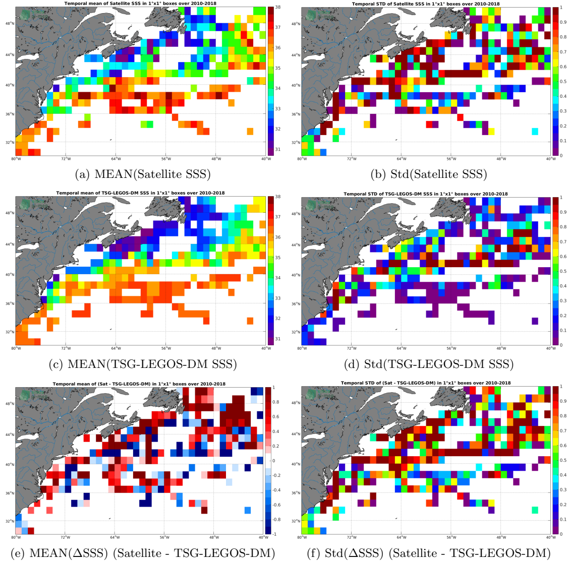
Figure 6: Temporal mean (left) and Std (right) of SSS from SMOS-L3-CATDS-CPDC-V321-L2Q (top), TSG-LEGOS-DM (middle), and of \Delta SSS (Satellite - TSG-LEGOS-DM). Only match-up pairs are used to generate these maps.
