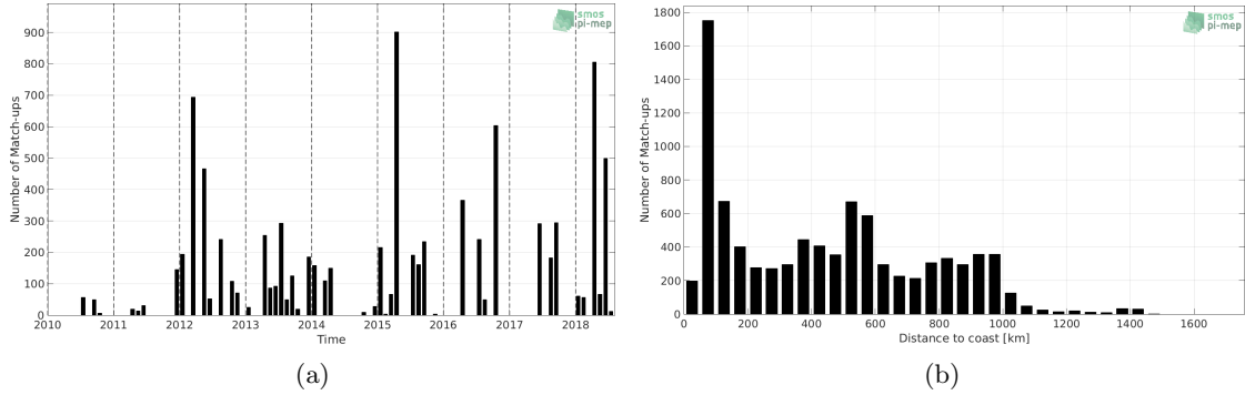
Figure 1: Number of match-ups between TSG-LEGOS-DM and SMOS-L3-CATDS-CPDC-V321-L2Q SSS as a function of time (a) and as function of the distance to coast (b) over the Gulf Stream Pi-MEP region and for the full satellite product period.
