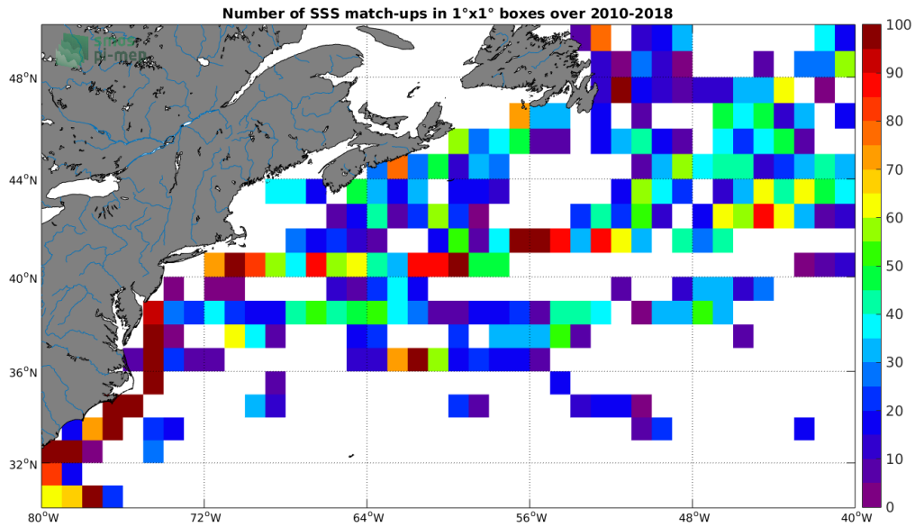
Figure 4: Number of SSS match-ups between TSG-LEGOS-DM SSS and the SMOS-L3-CATDS-CPDC-V321-L2Q SSS product for the Gulf Stream Pi-MEP region over 1^\circ \times 1^\circ boxes and for the full satellite product period.
