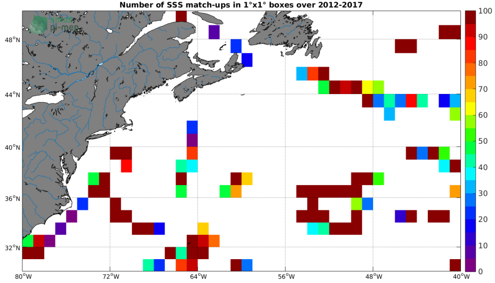
Figure 4: Number of SSS match-ups between TSG (GOSUD-Sailing-ship) SSS and the SMOS SSS L2Q v321 - 0.25 Deg (CATDS-CPDC) SSS product for the Gulf Stream Pi-MEP region over 1^\circ \times 1^\circ boxes and for the full satellite product period.
