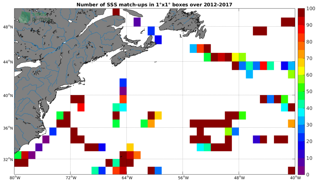
Figure 4: Number of SSS match-ups between TSG (GOSUD-Sailing-ship) SSS and the SMOS SSS L2Q v321 - 0.25 Deg (CATDS-CPDC) SSS product for the Gulf Stream Pi-MEP region over 1°x1° boxes and for the full satellite product period.
