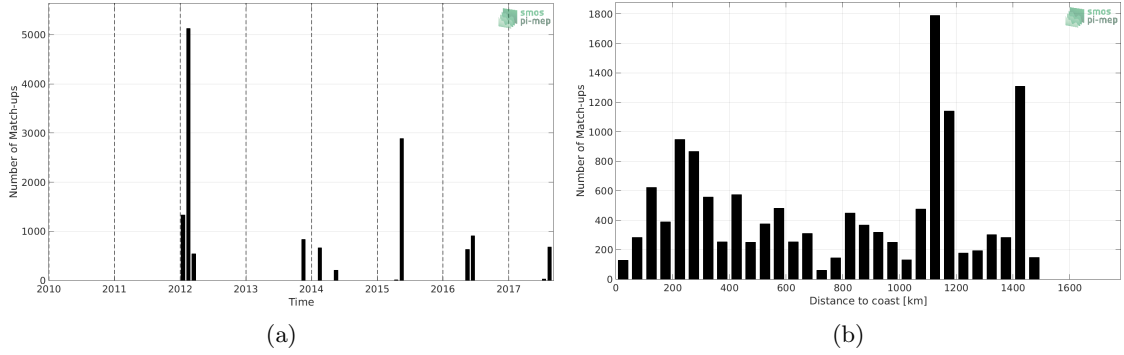
Figure 1: Number of match-ups between TSG (GOSUD-Sailing-ship) and SMOS SSS L2Q v321 - 0.25 Deg (CATDS-CPDC) SSS as a function of time (a) and as function of the distance to coast (b) over the Gulf Stream Pi-MEP region and for the full satellite product period.
