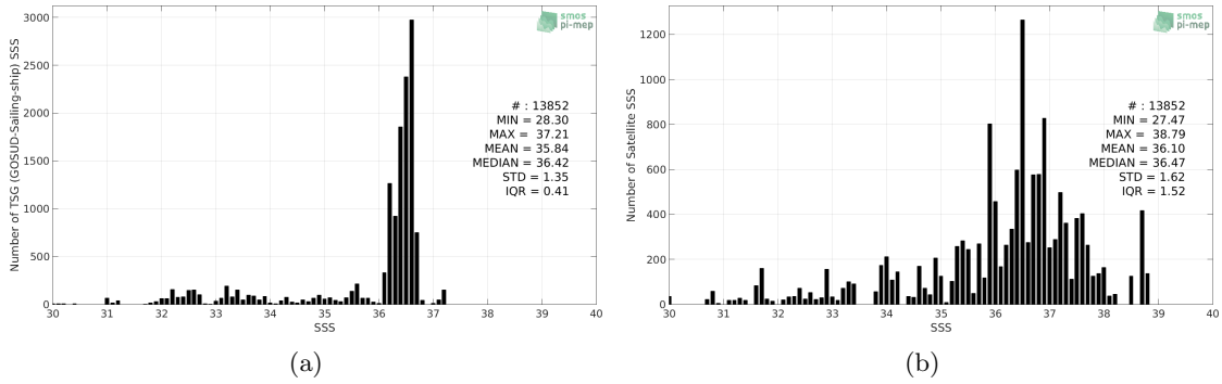
Figure 2: Histograms of SSS from TSG (GOSUD-Sailing-ship) (a) and SMOS SSS L2Q v321 - 0.25 Deg (CATDS-CPDC) (b) considering all match-up pairs per bins of 0.1 over the Gulf Stream Pi-MEP region and for the full satellite product period.
