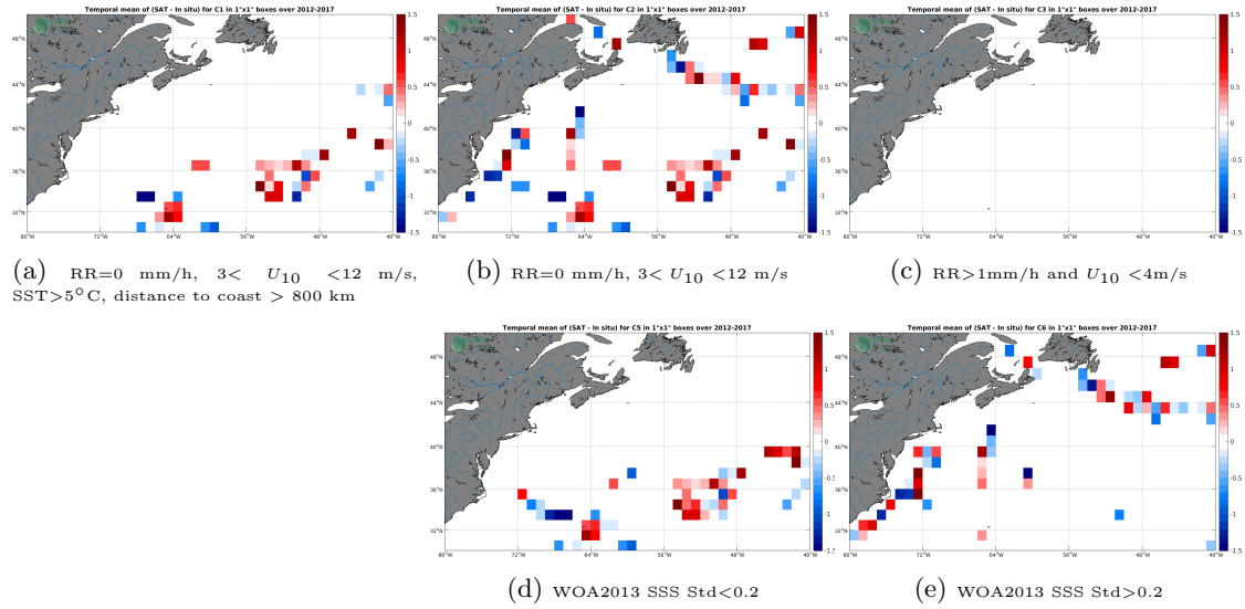
Figure 12: Temporal mean gridded over spatial boxes of size 1^\circ \times 1^\circ of \Delta SSS (SMOS SSS L2Q v321 - 0.25 Deg (CATDS-CPDC) - TSG (GOSUD-Sailing-ship)) for 5 different subdatasets corresponding to: RR=0 mm/h, 3 < U_{10} < 12 m/s, SST > 5^\circ\text{C} , distance to coast > 800 km (a), RR=0 mm/h, 3 < U_{10} < 12 m/s (b), RR > 1 mm/h and U_{10} < 4 m/s (c), WOA2013 SSS Std < 0.2 (d), WOA2013 SSS Std > 0.2 (e).
