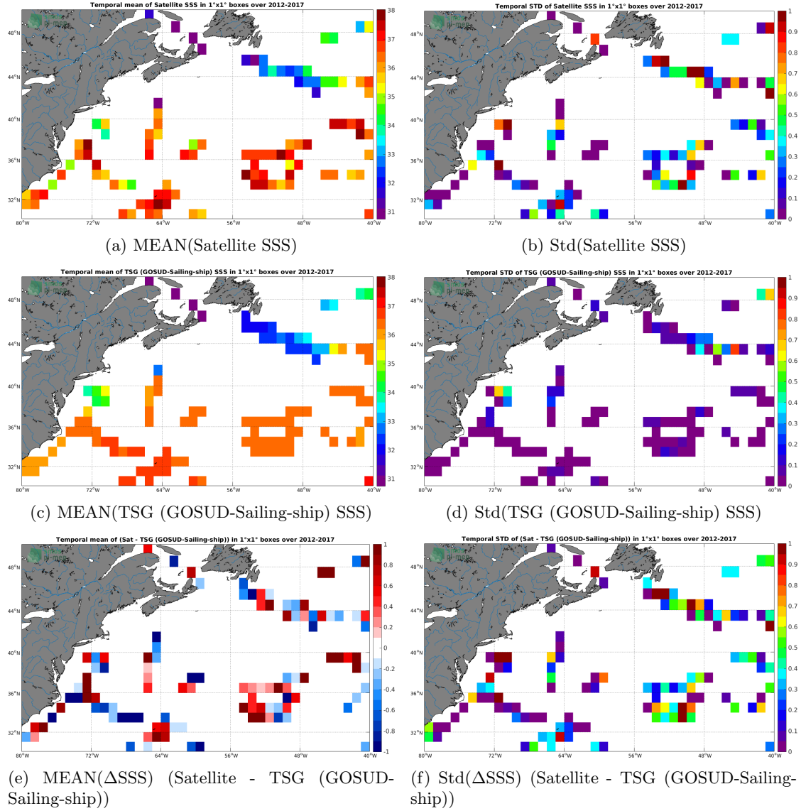
Figure 6: Temporal mean (left) and Std (right) of SSS from SMOS SSS L2Q v321 - 0.25 Deg (CATDS-CPDC) (top), TSG (GOSUD-Sailing-ship) (middle), and of \Delta SSS (Satellite - TSG (GOSUD-Sailing-ship)). Only match-up pairs are used to generate these maps.
