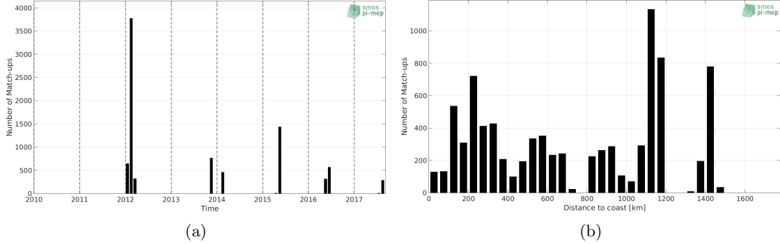
Figure 1: Number of match-ups between TSG-GOSUD-Sailing-ship and SMOS-L3-CATDS-CPDC-V321-L2Q SSS as a function of time (a) and as function of the distance to coast (b) over the Gulf Stream Pi-MEP region and for the full satellite product period.
