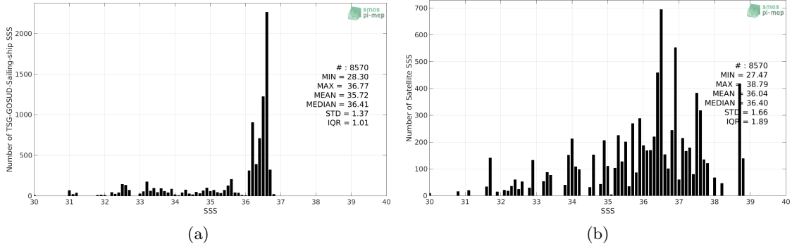
Figure 2: Histograms of SSS from TSG-GOSUD-Sailing-ship (a) and SMOS-L3-CATDS-CPDC-V321-L2Q (b) considering all match-up pairs per bins of 0.1 over the Gulf Stream Pi-MEP region and for the full satellite product period.
