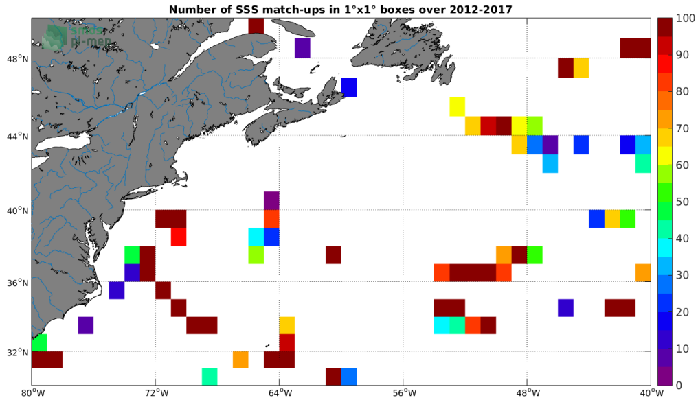
Figure 4: Number of SSS match-ups between TSG-GOSUD-Sailing-ship SSS and the SMOS-L3-CATDS-CPDC-V321-L2Q SSS product for the Gulf Stream Pi-MEP region over 1°x1° boxes and for the full satellite product period.
