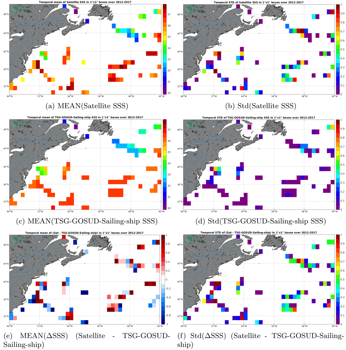
Figure 6: Temporal mean (left) and Std (right) of SSS from SMOS-L3-CATDS-CPDC-V321-L2Q (top), TSG-GOSUD-Sailing-ship (middle), and of \Delta SSS (Satellite - TSG-GOSUD-Sailing-ship). Only match-up pairs are used to generate these maps.
