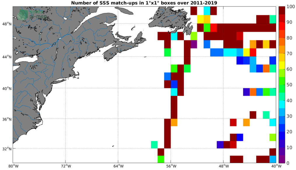
Figure 4: Number of SSS match-ups between TSG (GOSUD-Research-vessel) SSS and the SMOS SSS L2Q v321 - 0.25 Deg (CATDS-CPDC) SSS product for the Gulf Stream Pi-MEP region over 1^\circ \times 1^\circ boxes and for the full satellite product period.
