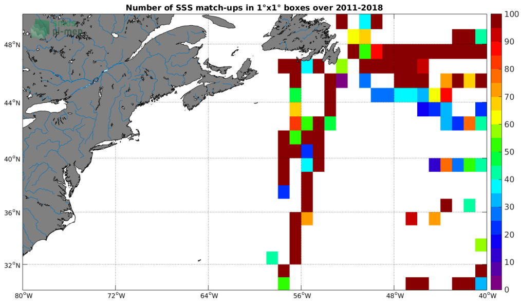
Figure 4: Number of SSS match-ups between TSG-GOSUD-Research-vessel SSS and the SMOS L2Q v321 - 0.25 Deg (CATDS-CPDC) SSS product for the Gulf Stream Pi-MEP region over 1°x1° boxes and for the full satellite product period.
