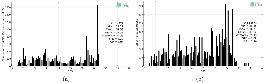
Figure 2: Histograms of SSS from TSG-GOSUD-Research-vessel (a) and SMOS L2Q v321 - 0.25 Deg (CATDS-CPDC) (b) considering all match-up pairs per bins of 0.1 over the Gulf Stream Pi-MEP region and for the full satellite product period.
