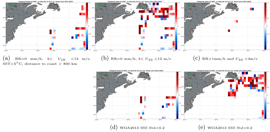
Figure 12: Temporal mean gridded over spatial boxes of size 1^{\circ}\times 1^{\circ} of \Delta SSS (SMOS L2Q v321 - 0.25 Deg (CATDS-CPDC) - TSG-GOSUD-Research-vessel) for 5 different subdatasets corresponding to:RR=0 mm/h, 3 < U_{10} < 12 m/s, SST >5^{\circ}\text{C} , distance to coast > 800 km (a), RR=0 mm/h, 3 < U_{10} < 12 m/s (b), RR >1 mm/h and U_{10} < 4 m/s (c), WOA2013 SSS Std <0.2 (d), WOA2013 SSS Std >0.2 (e).
