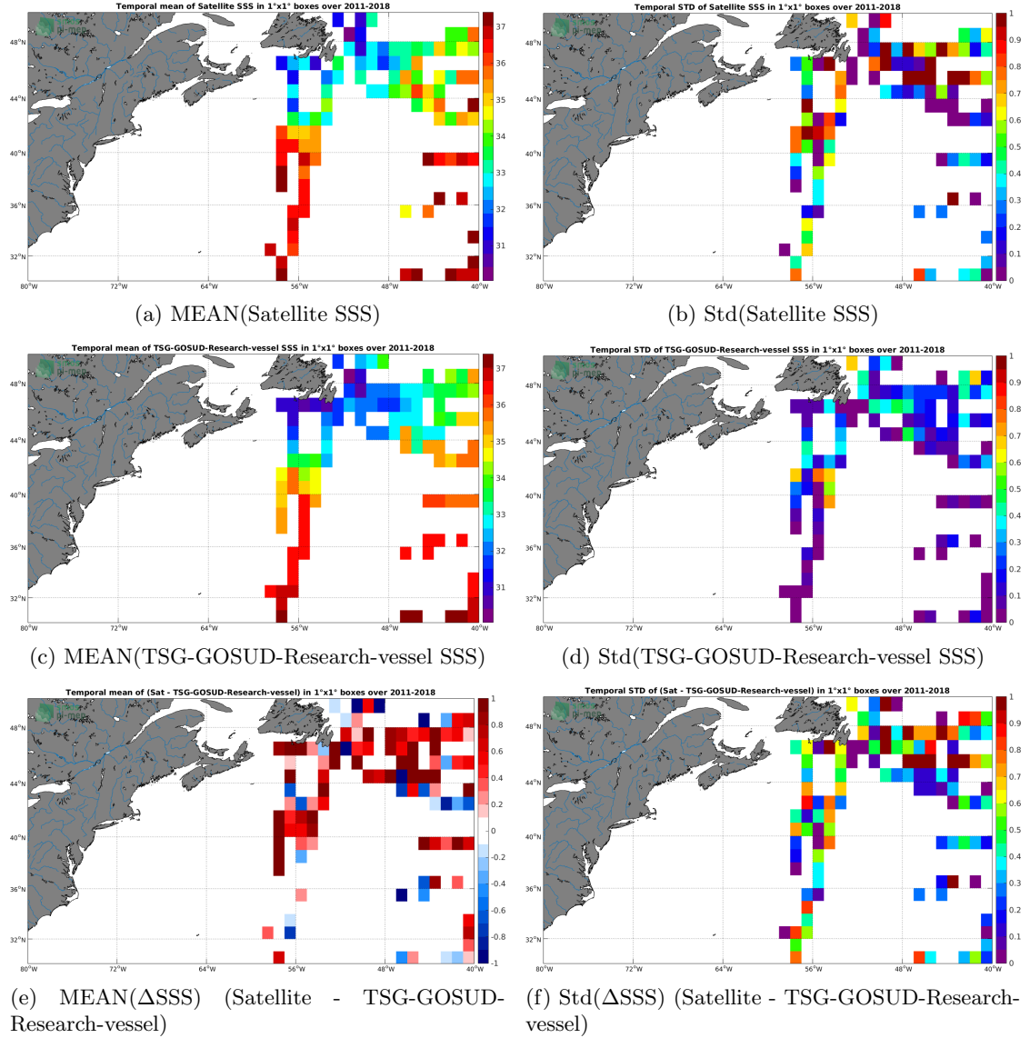
Figure 6: Temporal mean (left) and Std (right) of SSS from SMOS L2Q v321 - 0.25 Deg (CATDS-CPDC) (top), TSG-GOSUD-Research-vessel (middle), and of \Delta SSS (Satellite - TSG-GOSUD-Research-vessel). Only match-up pairs are used to generate these maps.
