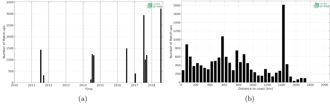
Figure 1: Number of match-ups between TSG-GOSUD-Research-vessel and SMOS L2Q v321 - 0.25 Deg (CATDS-CPDC) SSS as a function of time (a) and as function of the distance to coast (b) over the Gulf Stream Pi-MEP region and for the full satellite product period.
