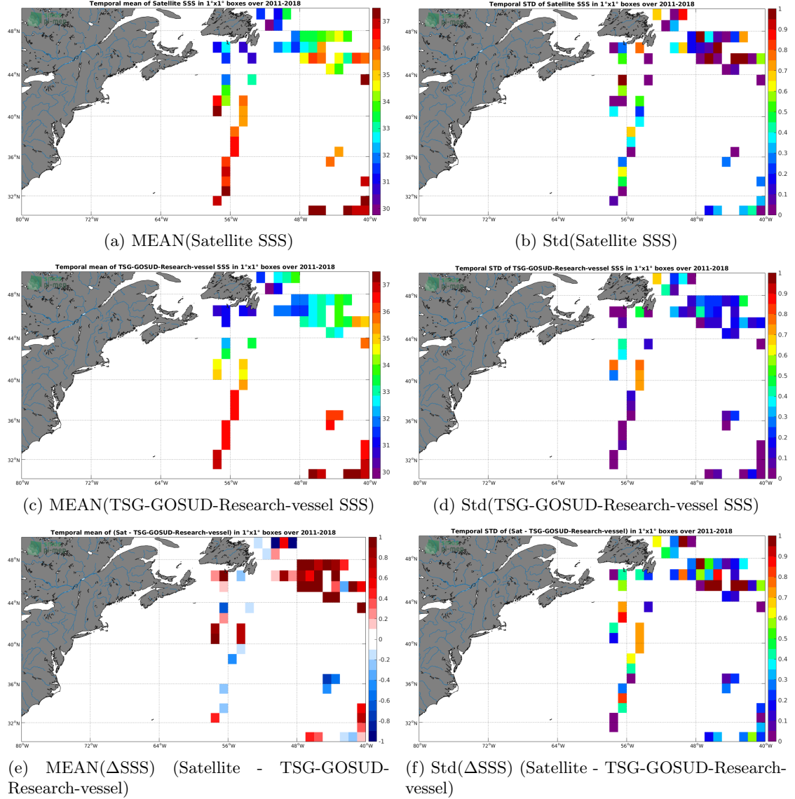
Figure 6: Temporal mean (left) and Std (right) of SSS from SMOS-L3-CATDS-CPDC-V321-L2Q (top), TSG-GOSUD-Research-vessel (middle), and of \Delta SSS (Satellite - TSG-GOSUD-Research-vessel). Only match-up pairs are used to generate these maps.
