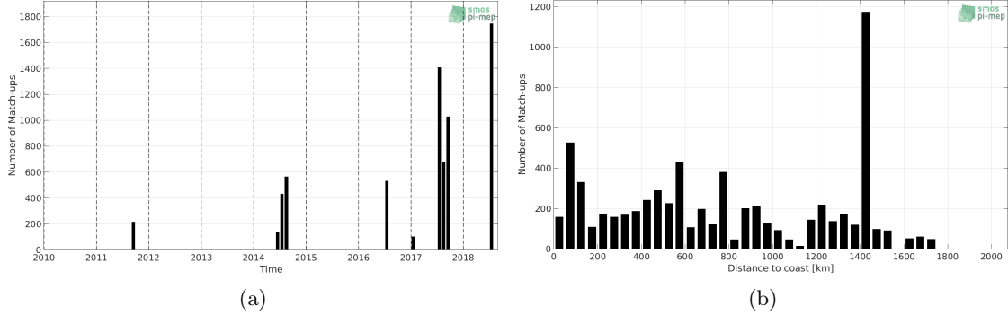
Figure 1: Number of match-ups between TSG-GOSUD-Research-vessel and SMOS-L3-CATDS-CPDC-V321-L2Q SSS as a function of time (a) and as function of the distance to coast (b) over the Gulf Stream Pi-MEP region and for the full satellite product period.
