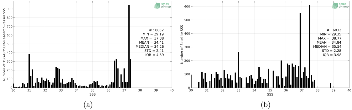
Figure 2: Histograms of SSS from TSG-GOSUD-Research-vessel (a) and SMOS-L3-CATDS-CPDC-V321-L2Q (b) considering all match-up pairs per bins of 0.1 over the Gulf Stream Pi-MEP region and for the full satellite product period.
