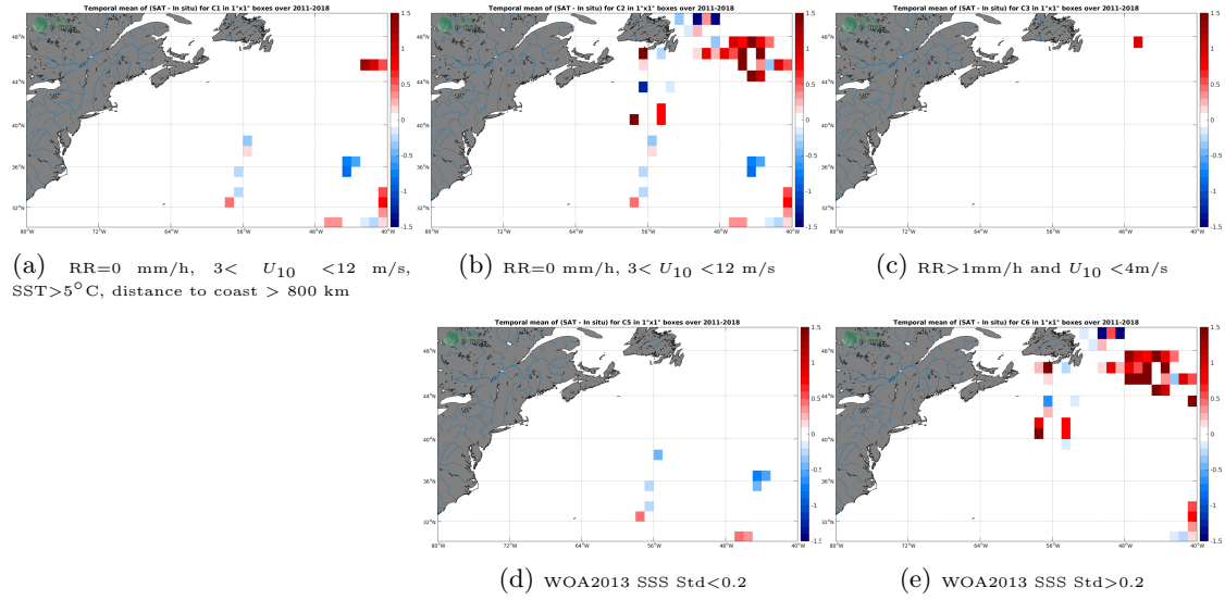
Figure 12: Temporal mean gridded over spatial boxes of size 1^\circ \times 1^\circ of \Delta SSS (SMOS-L3-CATDS-CPDC-V321-L2Q - TSG-GOSUD-Research-vessel) for 5 different subdatasets corresponding to: RR=0 mm/h, 3 < U_{10} < 12 m/s, SST > 5^\circ C , distance to coast > 800 km (a), RR=0 mm/h, 3 < U_{10} < 12 m/s (b), RR > 1 mm/h and U_{10} < 4 m/s (c), WOA2013 SSS Std < 0.2 (d), WOA2013 SSS Std > 0.2 (e).
