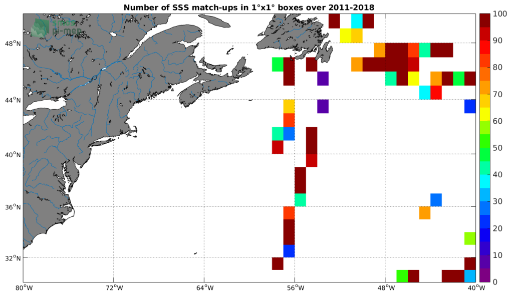
Figure 4: Number of SSS match-ups between TSG-GOSUD-Research-vessel SSS and the SMOS-L3-CATDS-CPDC-V321-L2Q SSS product for the Gulf Stream Pi-MEP region over 1°x1° boxes and for the full satellite product period.
