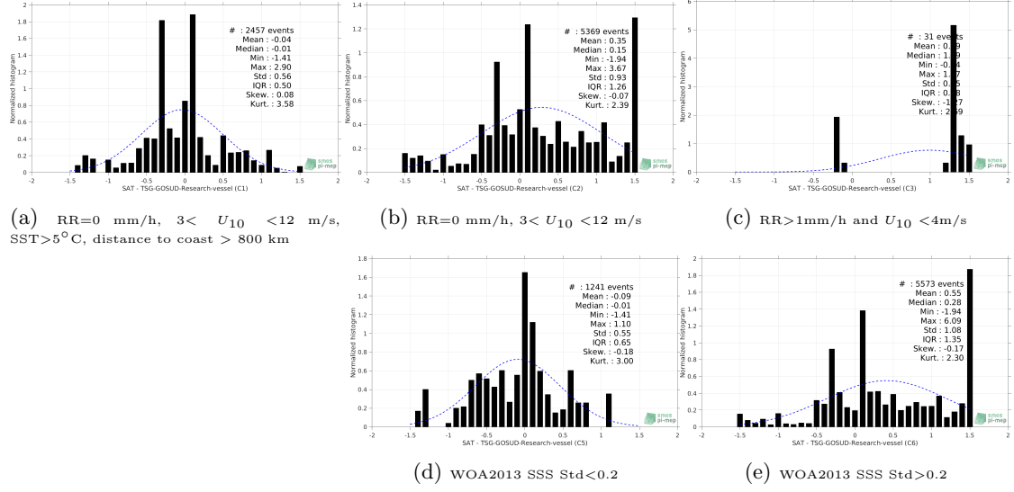
Figure 13: Normalized histogram of \Delta SSS (SMOS-L3-CATDS-CPDC-V321-L2Q - TSG-GOSUD-Research-vessel) for 5 different subdatasets corresponding to: RR=0 mm/h, 3 < U_{10} < 12 m/s, SST>5°C, distance to coast > 800 km (a), RR=0 mm/h, 3 < U_{10} < 12 m/s (b), RR>1 mm/h and U_{10} < 4 m/s (c), WOA2013 SSS Std<0.2 (d), WOA2013 SSS Std>0.2 (e).
