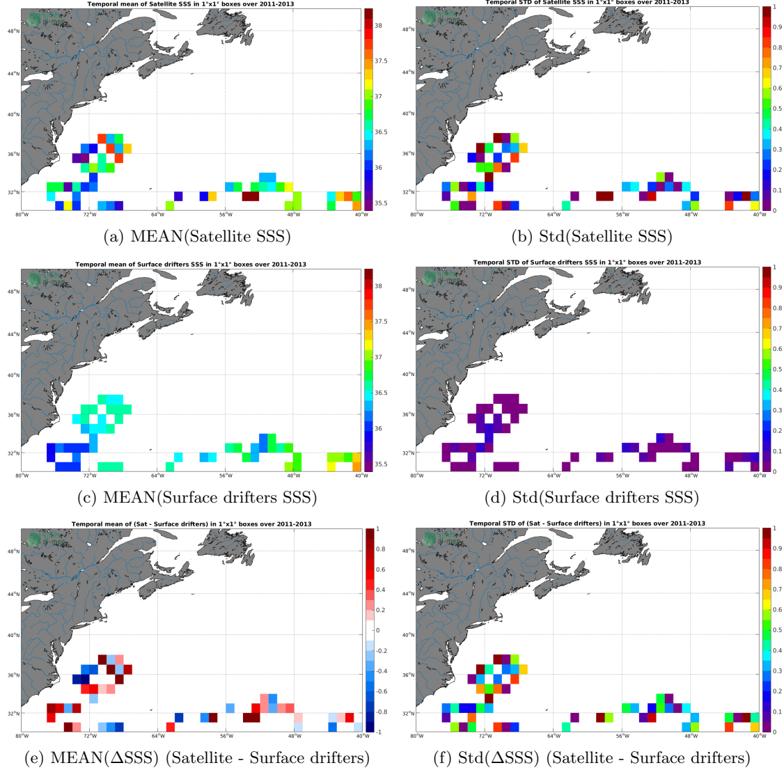
Figure 5: Temporal mean (left) and Std (right) of SSS from SMOS SSS L2Q v321 - 0.25 Deg (CATDS-CPDC) (top), Surface drifters (middle), and of \Delta\text{SSS} (Satellite - Surface drifters). Only match-up pairs are used to generate these maps.
