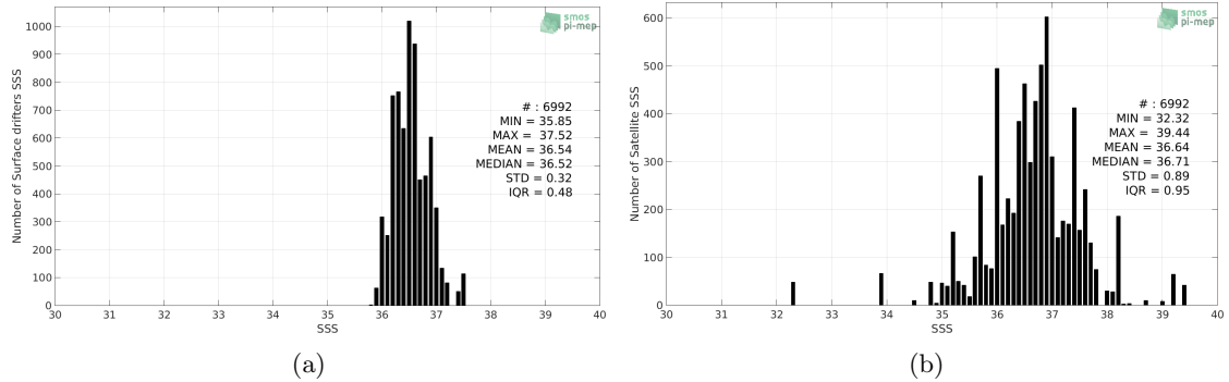
Figure 2: Histograms of SSS from Surface drifters (a) and SMOS L2Q v321 - 0.25 Deg (CATDS-CPDC) (b) considering all match-up pairs per bins of 0.1 over the Gulf Stream Pi-MEP region and for the full satellite product period.
