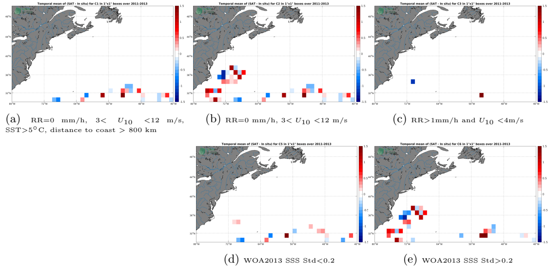
Figure 11: Temporal mean gridded over spatial boxes of size 1^{\circ}\times 1^{\circ} of \Delta\text{SSS} (SMOS L2Q v321 - 0.25 Deg (CATDS-CPDC) - Surface drifters) for 5 different subdatasets corresponding to:RR=0 mm/h, 3 < U_{10} < 12 m/s, SST >5^{\circ}\text{C} , distance to coast > 800 km (a), RR=0 mm/h, 3 < U_{10} < 12 m/s (b), RR >1 mm/h and U_{10} < 4 m/s (c), WOA2013 SSS Std <0.2 (d), WOA2013 SSS Std >0.2 (e).
