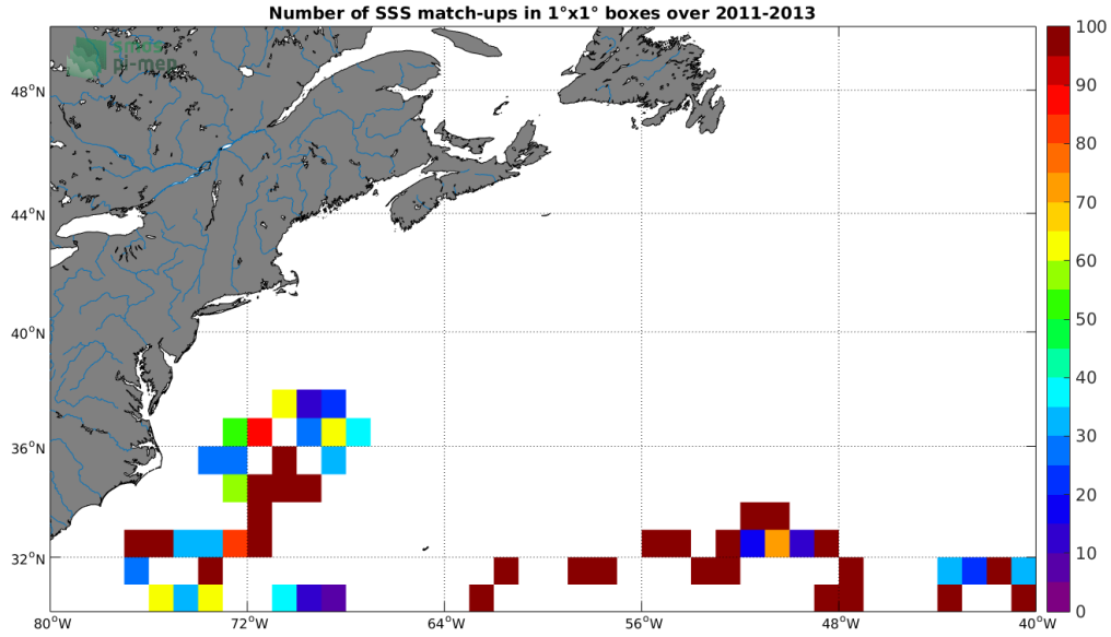
Figure 3: Number of SSS match-ups between Surface drifters SSS and the SMOS L2Q v321 - 0.25 Deg (CATDS-CPDC) SSS product for the Gulf Stream Pi-MEP region over 1^\circ \times 1^\circ boxes and for the full satellite product period.
