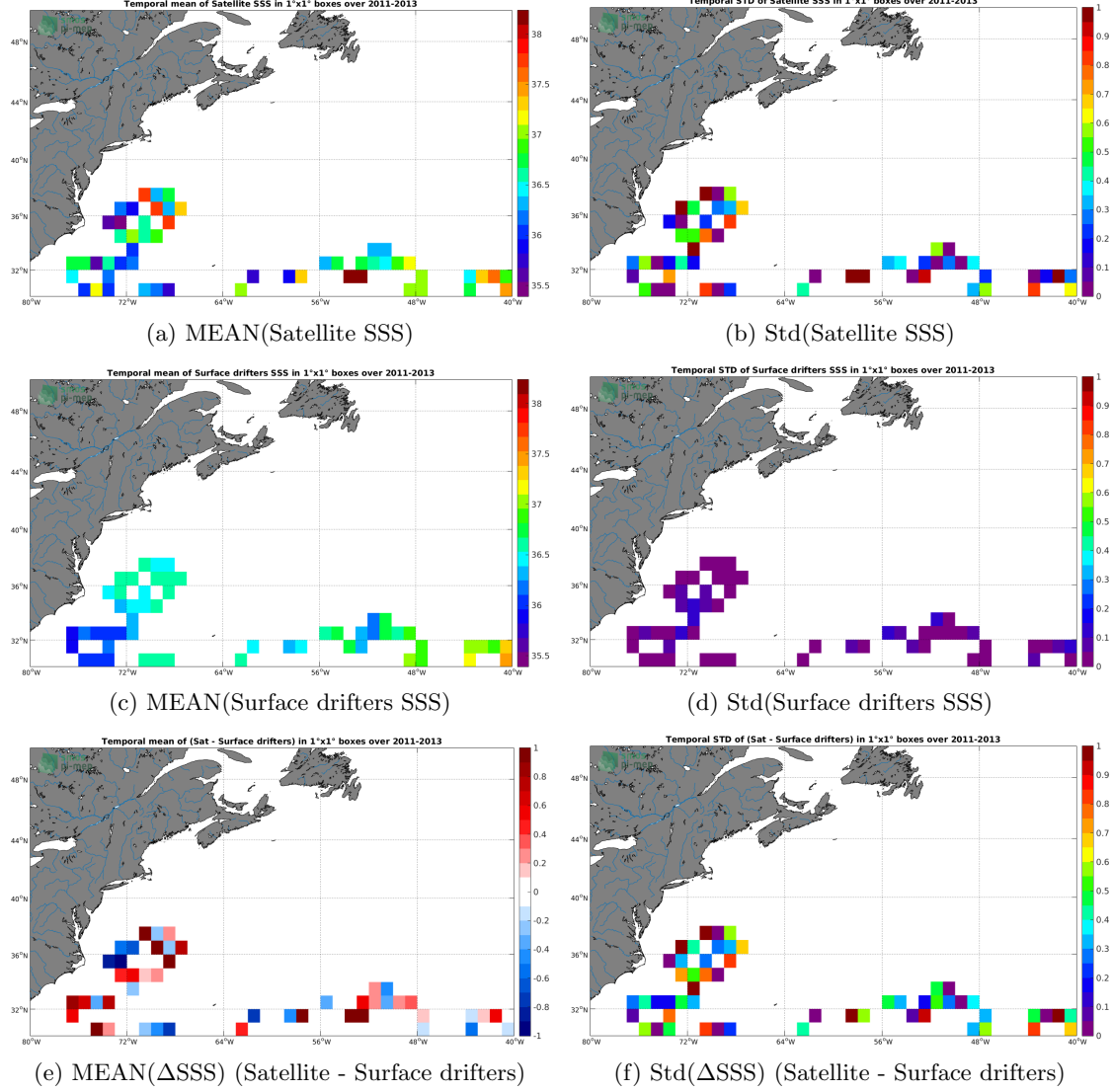
Figure 5: Temporal mean (left) and Std (right) of SSS from SMOS L2Q v321 - 0.25 Deg (CATDS-CPDC) (top), Surface drifters (middle), and of \Delta\text{SSS} (Satellite - Surface drifters). Only match-up pairs are used to generate these maps.
