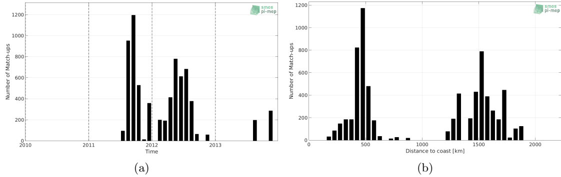
Figure 1: Number of match-ups between Surface drifters and SMOS L2Q v321 - 0.25 Deg (CATDS-CPDC) SSS as a function of time (a) and as function of the distance to coast (b) over the Gulf Stream Pi-MEP region and for the full satellite product period.
