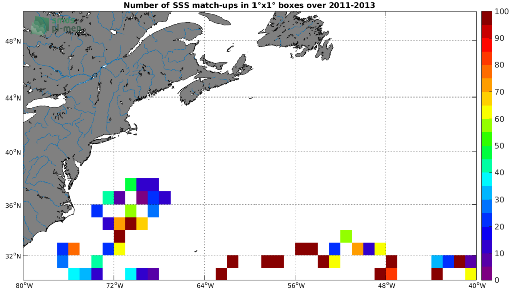
Figure 3: Number of SSS match-ups between Surface drifters SSS and the SMOS-L3-CATDS-CPDC-V321-L2Q SSS product for the Gulf Stream Pi-MEP region over 1°x1° boxes and for the full satellite product period.
