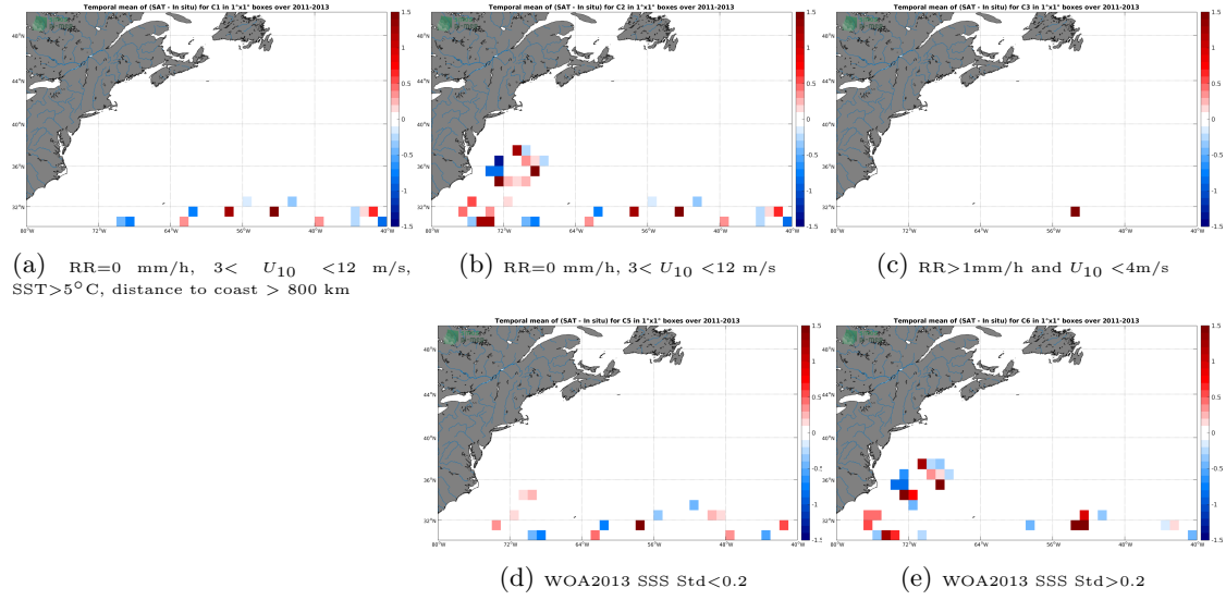
Figure 11: Temporal mean gridded over spatial boxes of size 1^\circ \times 1^\circ of \Delta SSS (SMOS-L3-CATDS-CPDC-V321-L2Q - Surface drifters) for 5 different subdatasets corresponding to: RR=0 mm/h, 3 < U_{10} < 12 m/s, SST > 5^\circ C , distance to coast > 800 km (a), RR=0 mm/h, 3 < U_{10} < 12 m/s (b), RR > 1 mm/h and U_{10} < 4 m/s (c), WOA2013 SSS Std < 0.2 (d), WOA2013 SSS Std > 0.2 (e).
