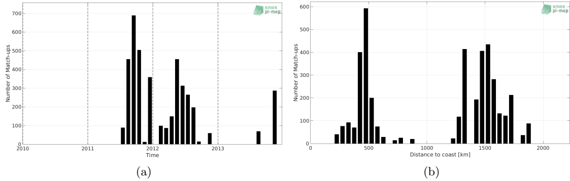
Figure 1: Number of match-ups between Surface drifters and SMOS-L3-CATDS-CPDC-V321-L2Q SSS as a function of time (a) and as function of the distance to coast (b) over the Gulf Stream Pi-MEP region and for the full satellite product period.
