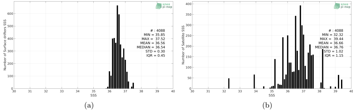
Figure 2: Histograms of SSS from Surface drifters (a) and SMOS-L3-CATDS-CPDC-V321-L2Q (b) considering all match-up pairs per bins of 0.1 over the Gulf Stream Pi-MEP region and for the full satellite product period.
