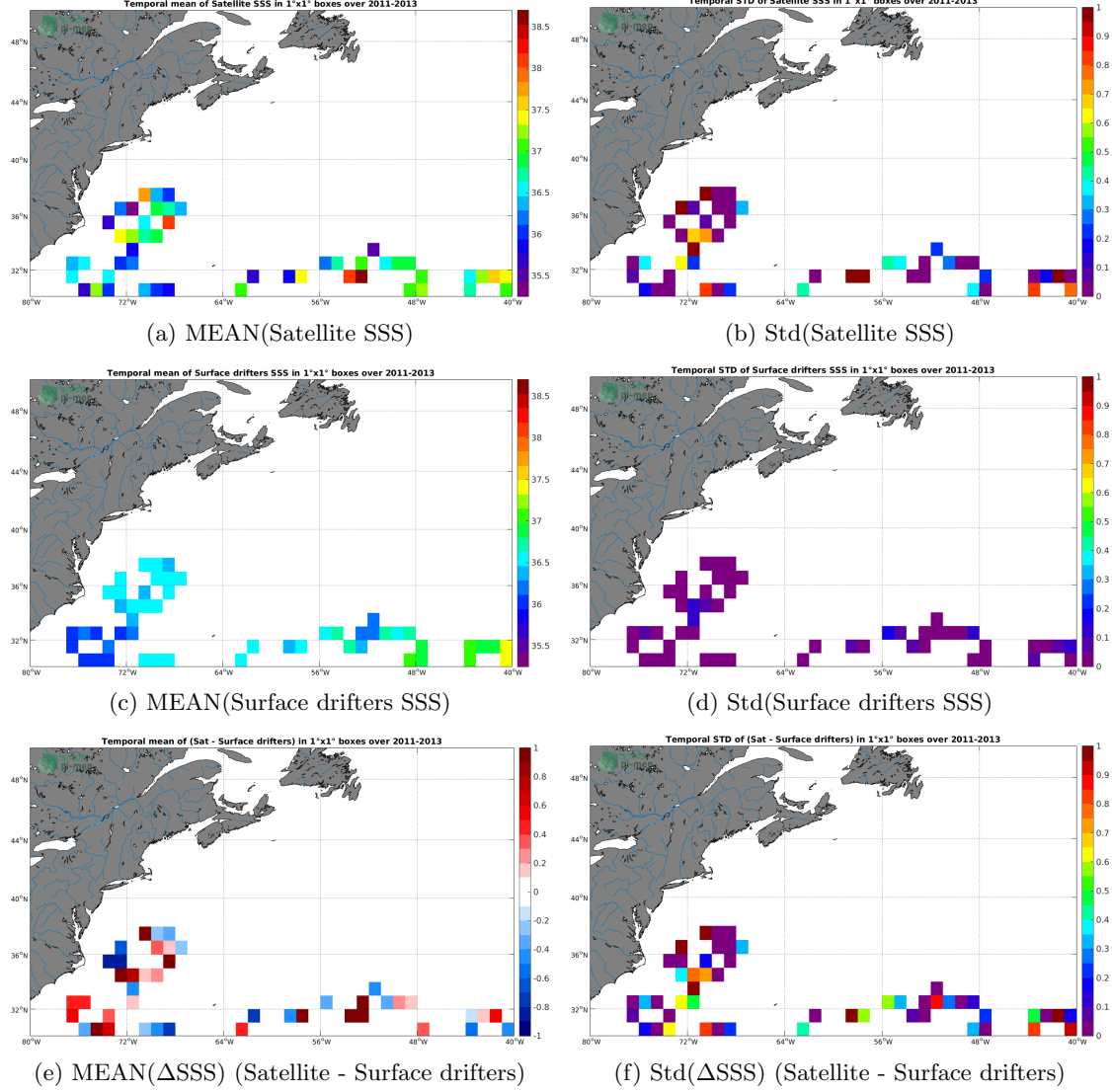
Figure 5: Temporal mean (left) and Std (right) of SSS from SMOS-L3-CATDS-CPDC-V321-L2Q (top), Surface drifters (middle), and of \Delta\text{SSS} (Satellite - Surface drifters). Only match-up pairs are used to generate these maps.
