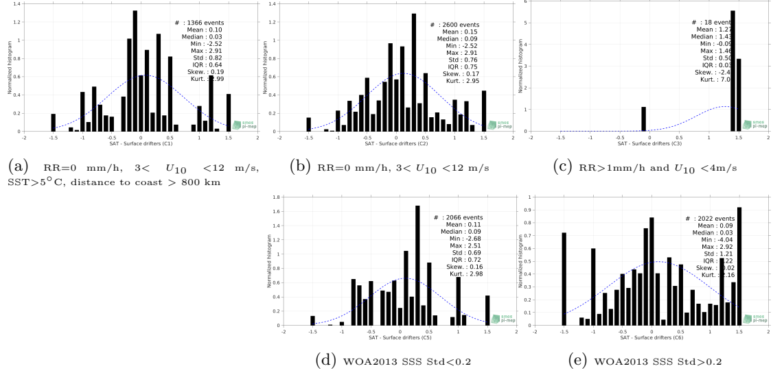
Figure 12: Normalized histogram of \Delta SSS (SMOS-L3-CATDS-CPDC-V321-L2Q - Surface drifters) for 5 different subdatasets corresponding to: RR=0 mm/h, 3 < U_{10} < 12 m/s, SST>5°C, distance to coast > 800 km (a), RR=0 mm/h, 3 < U_{10} < 12 m/s (b), RR>1mm/h and U_{10} < 4 m/s (c), WOA2013 SSS Std<0.2 (d), WOA2013 SSS Std>0.2 (e).
