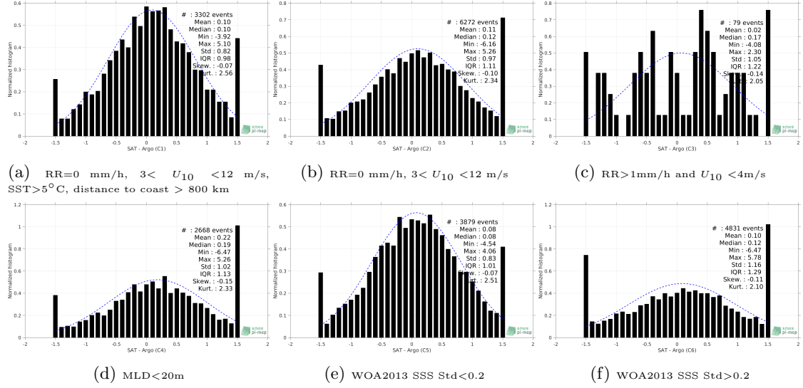
Figure 13: Normalized histogram of \Delta\text{SSS} (SMOS SSS L2Q v321 - 0.25 Deg (CATDS-CPDC) - Argo) for 6 different subdatasets corresponding to: RR=0 mm/h, 3 < U_{10} < 12 m/s, SST>5°C, distance to coast > 800 km (a), RR=0 mm/h, 3 < U_{10} < 12 m/s (b), RR>1mm/h and U_{10} < 4 m/s (c), MLD<20m (d), WOA2013 SSS Std<0.2 (e), WOA2013 SSS Std>0.2 (f).
