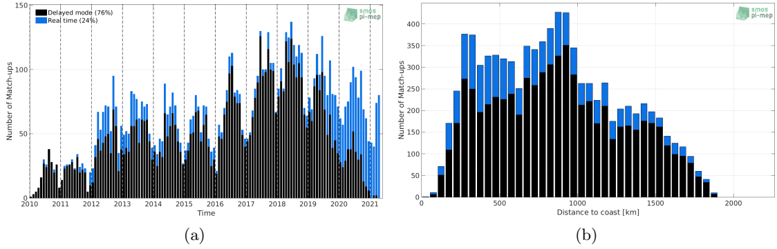
Figure 1: Number of match-ups between Argo and SMOS SSS L2Q v321 - 0.25 Deg (CATDS-CPDC) SSS as a function of time (a) and as function of the distance to coast (b) over the Gulf Stream Pi-MEP region and for the full satellite product period.
