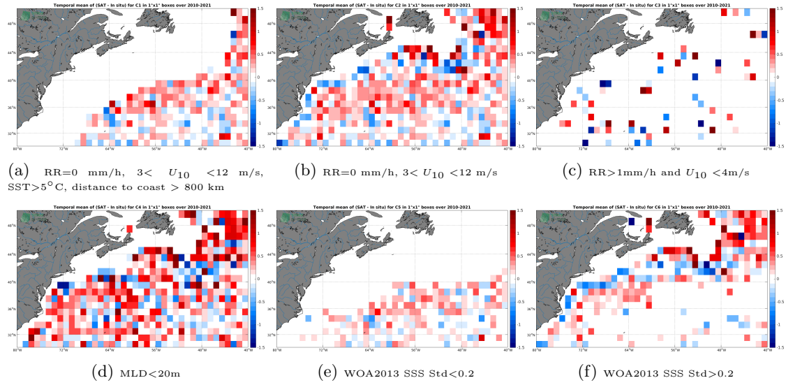
Figure 12: Temporal mean gridded over spatial boxes of size 1^\circ \times 1^\circ of \Delta SSS (SMOS SSS L2Q v321 - 0.25 Deg (CATDS-CPDC) - Argo) for 6 different subdatasets corresponding to: RR=0 mm/h, 3 < U_{10} < 12 m/s, SST > 5^\circ C , distance to coast > 800 km (a), RR=0 mm/h, 3 < U_{10} < 12 m/s (b), RR > 1 mm/h and U_{10} < 4 m/s (c), MLD < 20 m (d), WOA2013 SSS Std < 0.2 (e), WOA2013 SSS Std > 0.2 (f).
