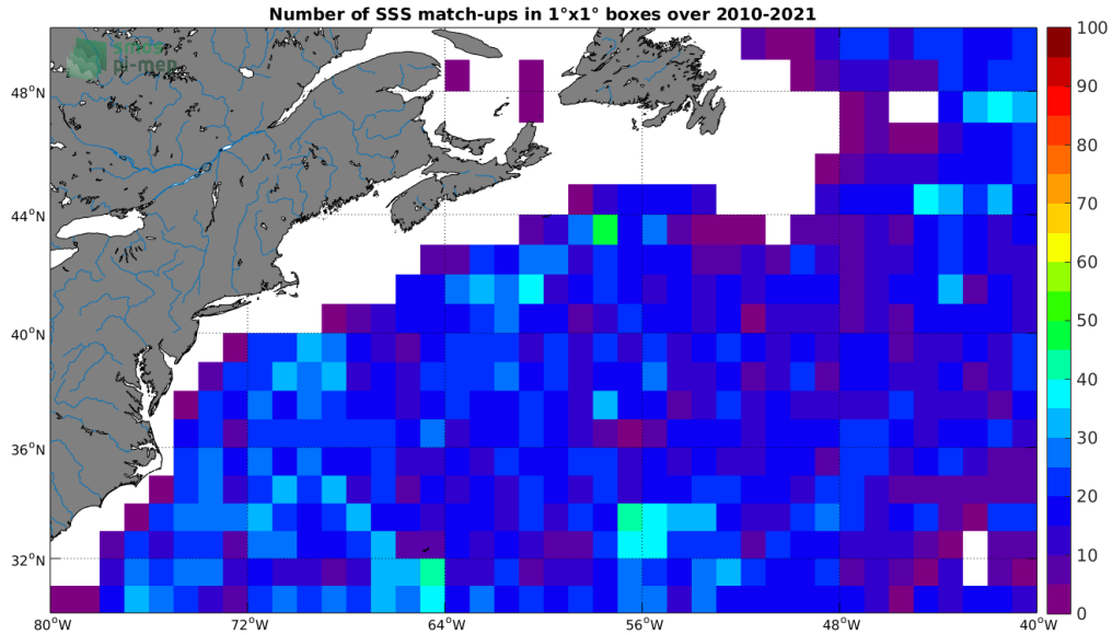
Figure 4: Number of SSS match-ups between Argo SSS and the SMOS SSS L2Q v321 - 0.25 Deg (CATDS-CPDC) SSS product for the Gulf Stream Pi-MEP region over 1^\circ \times 1^\circ boxes and for the full satellite product period.
