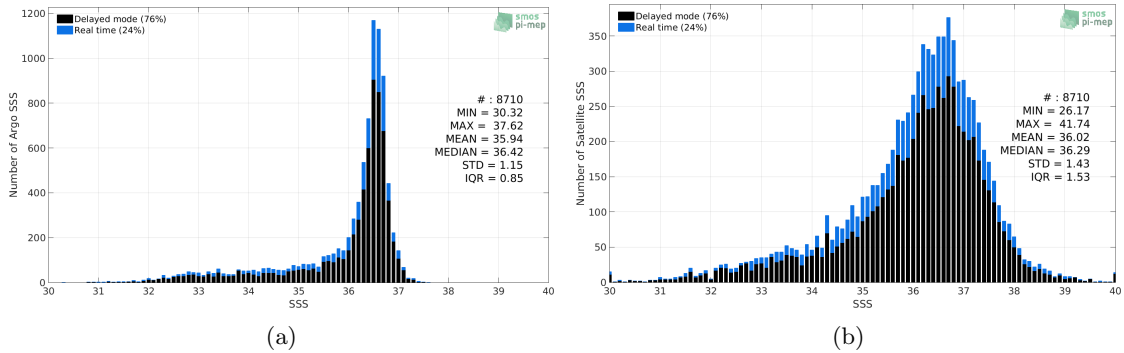
Figure 2: Histograms of SSS from Argo (a) and SMOS SSS L2Q v321 - 0.25 Deg (CATDS-CPDC) (b) considering all match-up pairs per bins of 0.1 over the Gulf Stream Pi-MEP region and for the full satellite product period.
