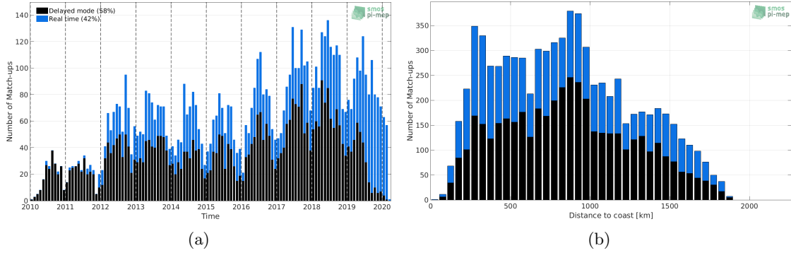
Figure 1: Number of match-ups between Argo and SMOS L2Q v321 - 0.25 Deg (CATDS-CPDC) SSS as a function of time (a) and as function of the distance to coast (b) over the Gulf Stream Pi-MEP region and for the full satellite product period.
