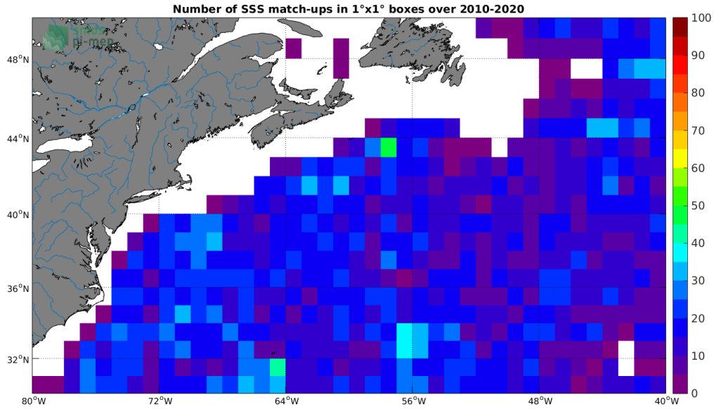
Figure 4: Number of SSS match-ups between Argo SSS and the SMOS L2Q v321 - 0.25 Deg (CATDS-CPDC) SSS product for the Gulf Stream Pi-MEP region over 1°x1° boxes and for the full satellite product period.
