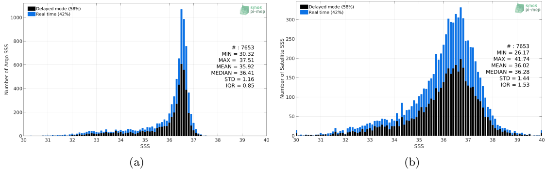
Figure 2: Histograms of SSS from Argo (a) and SMOS L2Q v321 - 0.25 Deg (CATDS-CPDC) (b) considering all match-up pairs per bins of 0.1 over the Gulf Stream Pi-MEP region and for the full satellite product period.
