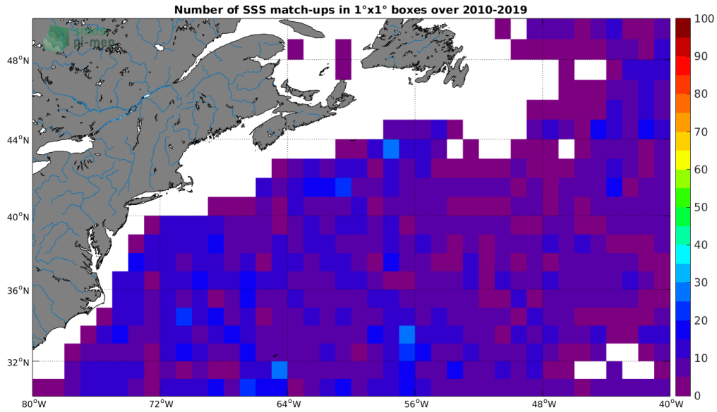
Figure 4: Number of SSS match-ups between Argo SSS and the SMOS-L3-CATDS-CPDC-V321-L2Q SSS product for the Gulf Stream Pi-MEP region over 1°x1° boxes and for the full satellite product period.
