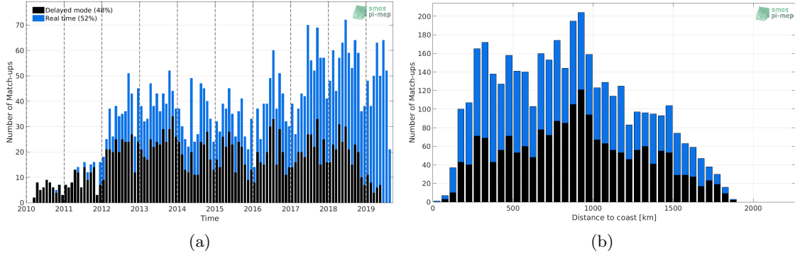
Figure 1: Number of match-ups between Argo and SMOS-L3-CATDS-CPDC-V321-L2Q SSS as a function of time (a) and as function of the distance to coast (b) over the Gulf Stream Pi-MEP region and for the full satellite product period.
