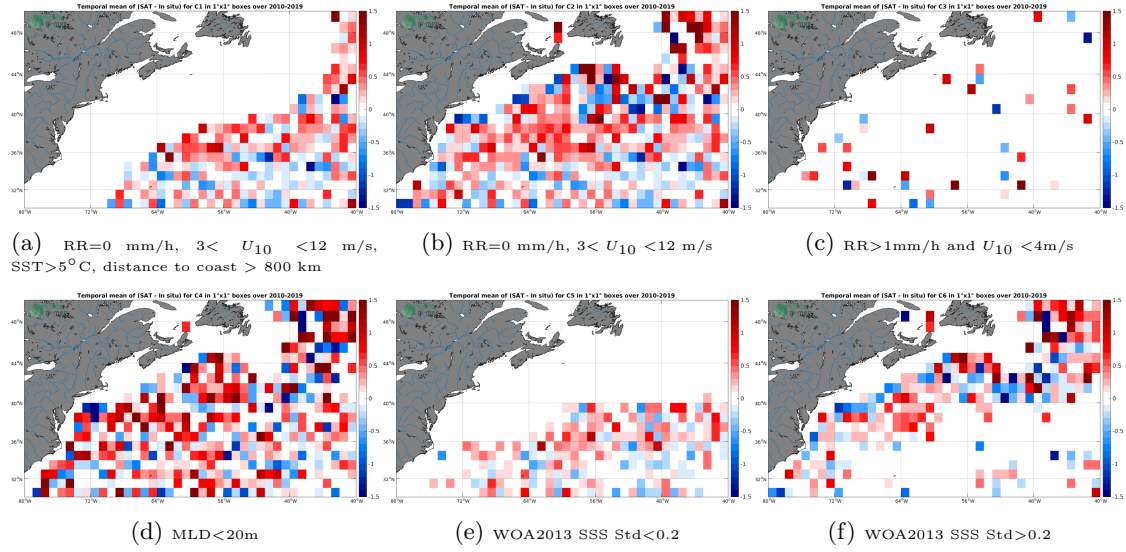
Figure 12: Temporal mean gridded over spatial boxes of size 1^\circ \times 1^\circ of \Delta SSS (SMOS-L3-CATDS-CPDC-V321-L2Q - Argo) for 6 different subdatasets corresponding to: RR=0 mm/h, 3 < U_{10} < 12 m/s, SST > 5^\circ\text{C} , distance to coast > 800 km (a), RR=0 mm/h, 3 < U_{10} < 12 m/s (b), RR > 1 mm/h and U_{10} < 4 m/s (c), MLD < 20 m (d), WOA2013 SSS Std < 0.2 (e), WOA2013 SSS Std > 0.2 (f).
