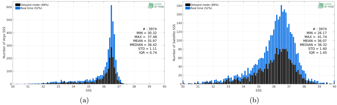
Figure 2: Histograms of SSS from Argo (a) and SMOS-L3-CATDS-CPDC-V321-L2Q (b) considering all match-up pairs per bins of 0.1 over the Gulf Stream Pi-MEP region and for the full satellite product period.
