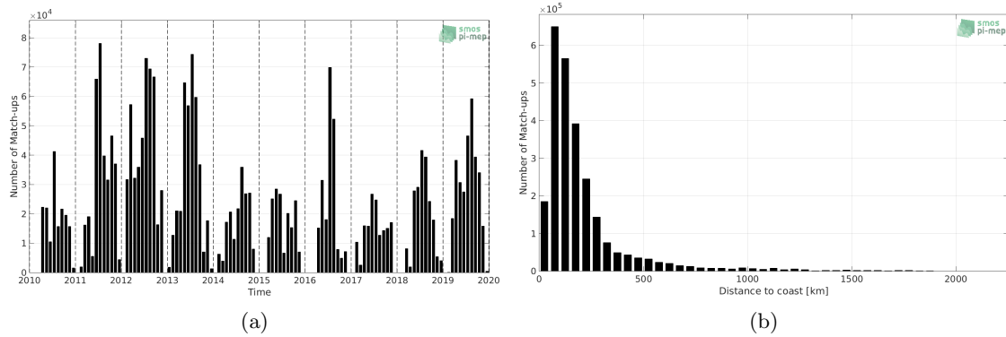
Figure 1: Number of match-ups between TSG-SAMOS and SMOS L3 v317 - Monthly - 25 km (CATDS-CPDC) SSS as a function of time (a) and as function of the distance to coast (b) over the Gulf Stream Pi-MEP region and for the full satellite product period.
