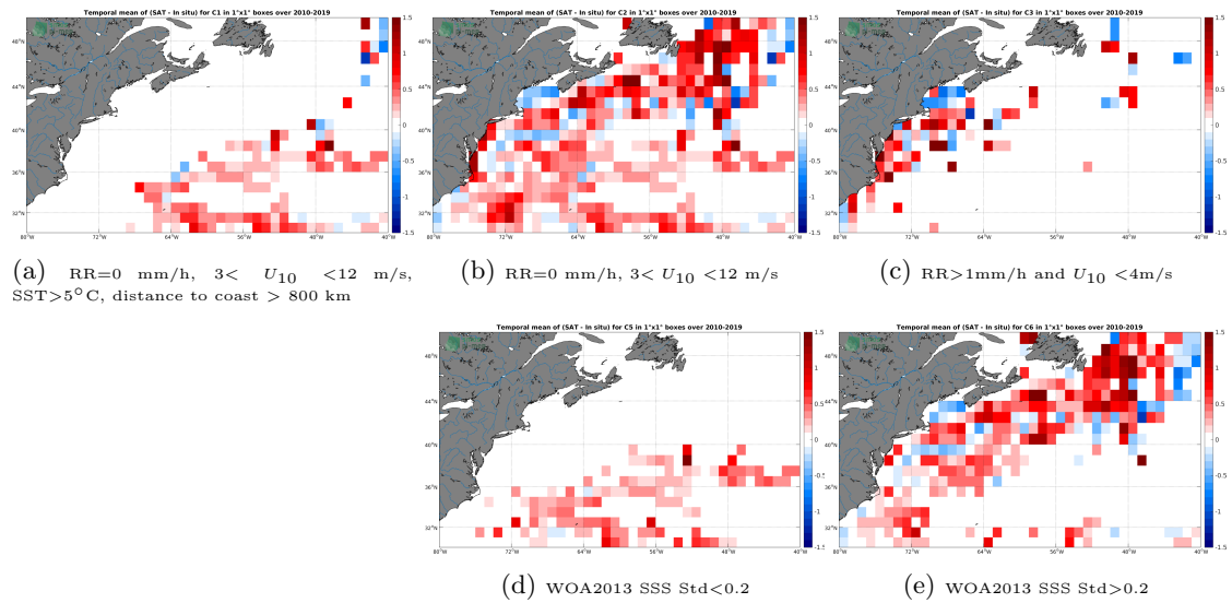
Figure 12: Temporal mean gridded over spatial boxes of size 1^\circ \times 1^\circ of \Delta SSS (SMOS L3 v317 - Monthly - 25 km (CATDS-CPDC) - TSG-SAMOS) for 5 different subdatasets corresponding to: RR=0 mm/h, 3 < U_{10} < 12 m/s, SST > 5^\circ C , distance to coast > 800 km (a), RR=0 mm/h, 3 < U_{10} < 12 m/s (b), RR > 1 mm/h and U_{10} < 4 m/s (c), WOA2013 SSS Std < 0.2 (d), WOA2013 SSS Std > 0.2 (e).
