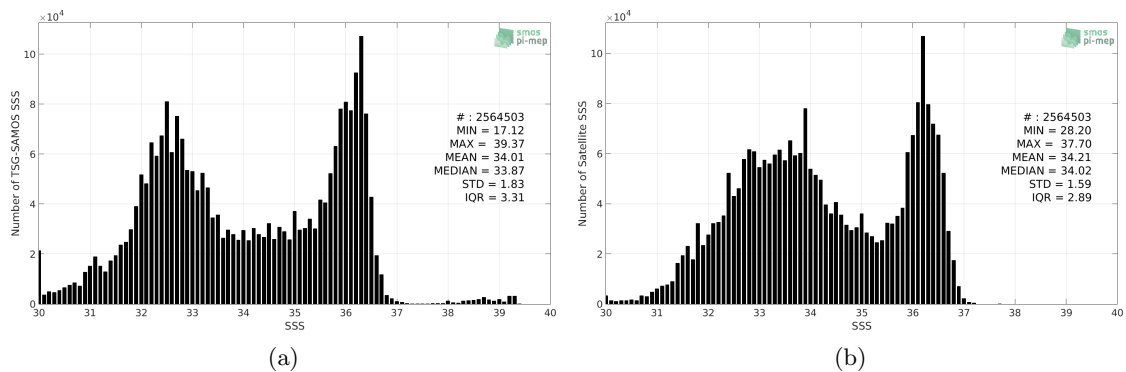
Figure 2: Histograms of SSS from TSG-SAMOS (a) and SMOS L3 v317 - Monthly - 25 km (CATDS-CPDC) (b) considering all match-up pairs per bins of 0.1 over the Gulf Stream Pi-MEP region and for the full satellite product period.
