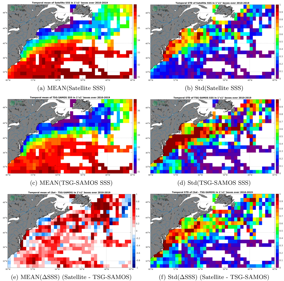
Figure 6: Temporal mean (left) and Std (right) of SSS from SMOS L3 v317 - Monthly - 25 km (CATDS-CPDC) (top), TSG-SAMOS (middle), and of \Delta SSS (Satellite - TSG-SAMOS). Only match-up pairs are used to generate these maps.
