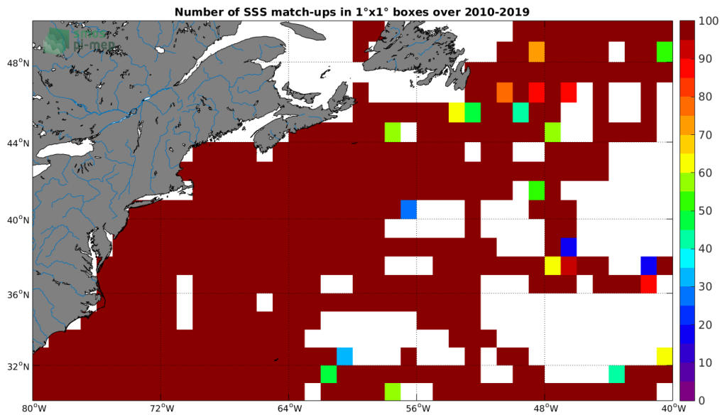
Figure 4: Number of SSS match-ups between TSG-SAMOS SSS and the SMOS L3 v317 - Monthly - 25 km (CATDS-CPDC) SSS product for the Gulf Stream Pi-MEP region over 1°x1° boxes and for the full satellite product period.
