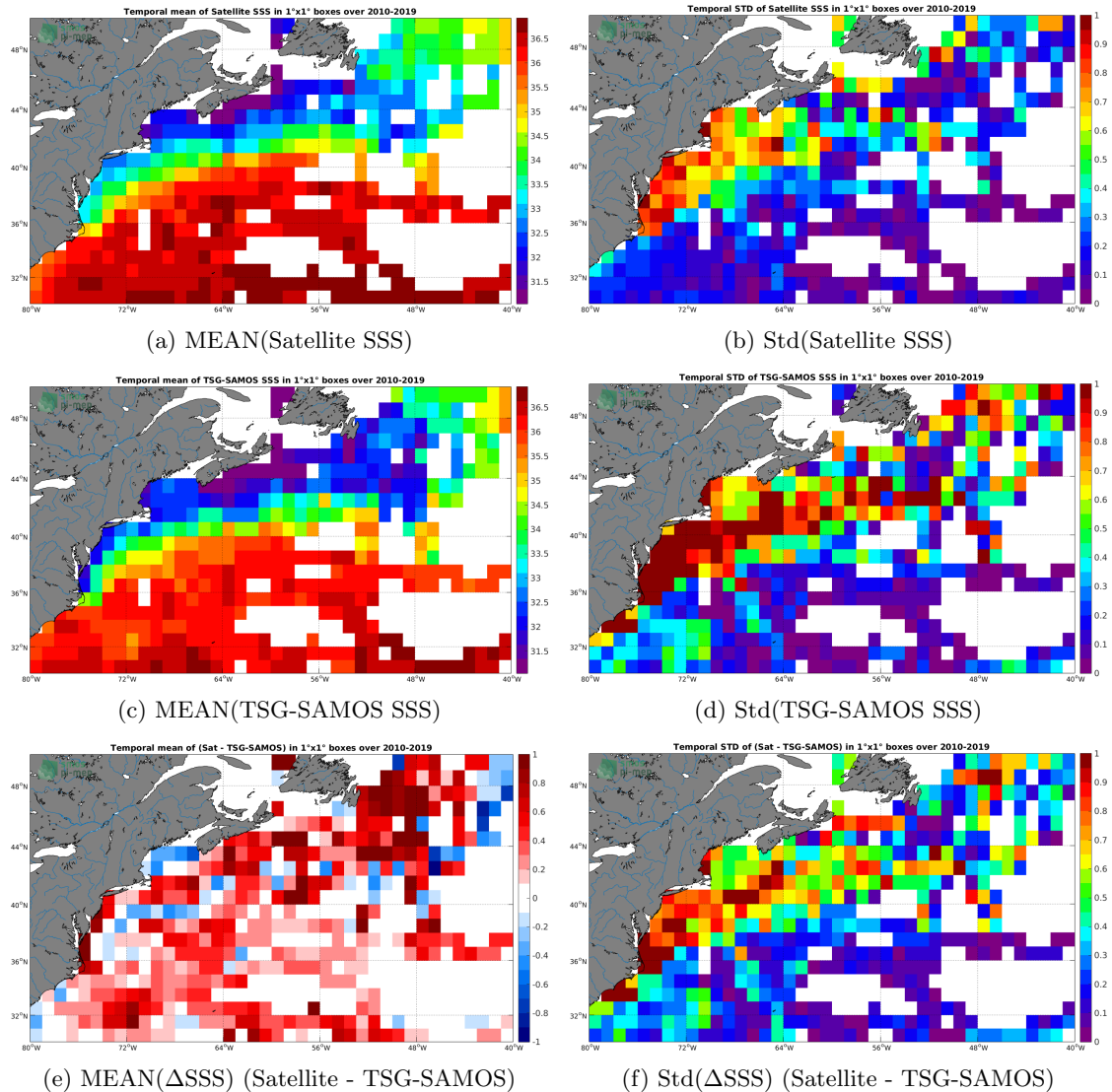
Figure 6: Temporal mean (left) and Std (right) of SSS from SMOS-L3-CATDS-CPDC-V317-MONTHLY-25KM (top), TSG-SAMOS (middle), and of \Delta SSS (Satellite - TSG-SAMOS). Only match-up pairs are used to generate these maps.
