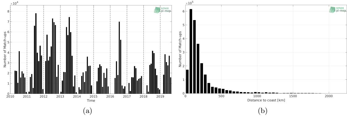
Figure 1: Number of match-ups between TSG-SAMOS and SMOS-L3-CATDS-CPDC-V317-MONTHLY-25KM SSS as a function of time (a) and as function of the distance to coast (b) over the Gulf Stream Pi-MEP region and for the full satellite product period.
