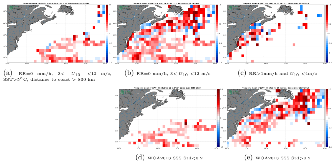
Figure 12: Temporal mean gridded over spatial boxes of size 1^\circ \times 1^\circ of \Delta SSS (SMOS-L3-CATDS-CPDC-V317-MONTHLY-25KM - TSG-SAMOS) for 5 different subdatasets corresponding to:RR=0 mm/h, 3 < U_{10} < 12 m/s, SST >5^\circ C, distance to coast > 800 km (a), RR=0 mm/h, 3 < U_{10} < 12 m/s (b), RR >1 mm/h and U_{10} < 4 m/s (c), WOA2013 SSS Std <0.2 (d), WOA2013 SSS Std >0.2 (e).
