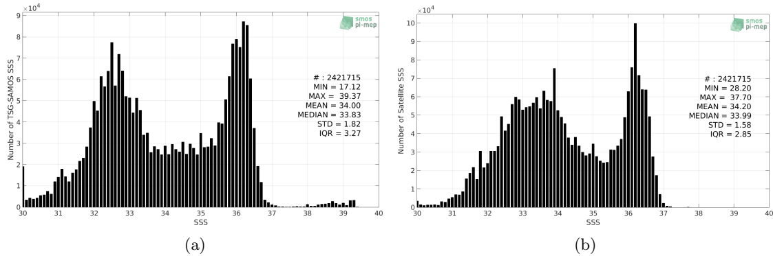
Figure 2: Histograms of SSS from TSG-SAMOS (a) and SMOS-L3-CATDS-CPDC-V317-MONTHLY-25KM (b) considering all match-up pairs per bins of 0.1 over the Gulf Stream Pi-MEP region and for the full satellite product period.
