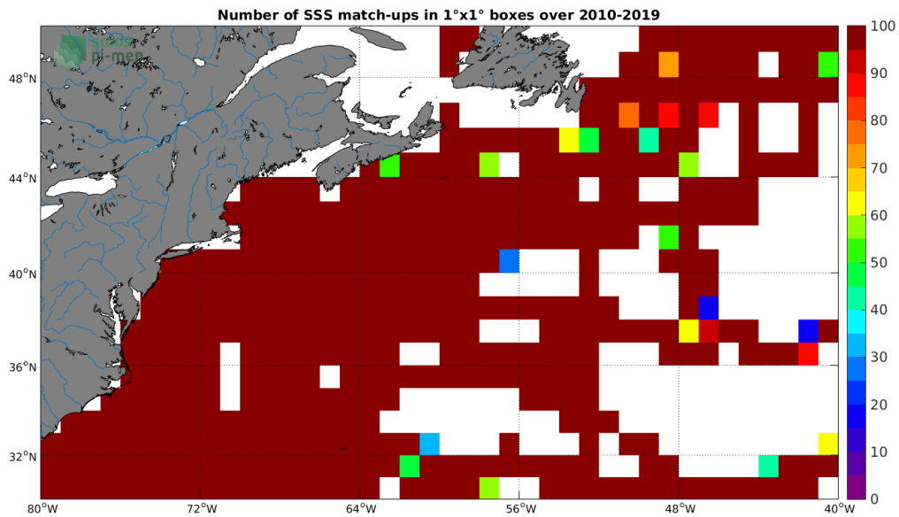
Figure 4: Number of SSS match-ups between TSG-SAMOS SSS and the SMOS-L3-CATDS-CPDC-V317-MONTHLY-25KM SSS product for the Gulf Stream Pi-MEP region over 1^\circ \times 1^\circ boxes and for the full satellite product period.
