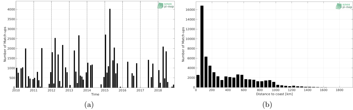
Figure 1: Number of match-ups between TSG-LEGOS-DM and SMOS L3 v317 - Monthly - 25 km (CATDS-CPDC) SSS as a function of time (a) and as function of the distance to coast (b) over the Gulf Stream Pi-MEP region and for the full satellite product period.
