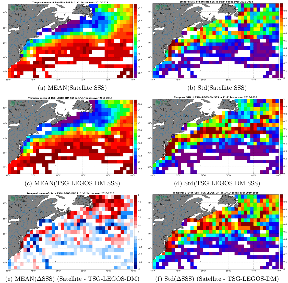
Figure 6: Temporal mean (left) and Std (right) of SSS from SMOS L3 v317 - Monthly - 25 km (CATDS-CPDC) (top), TSG-LEGOS-DM (middle), and of \Delta SSS (Satellite - TSG-LEGOS-DM). Only match-up pairs are used to generate these maps.
