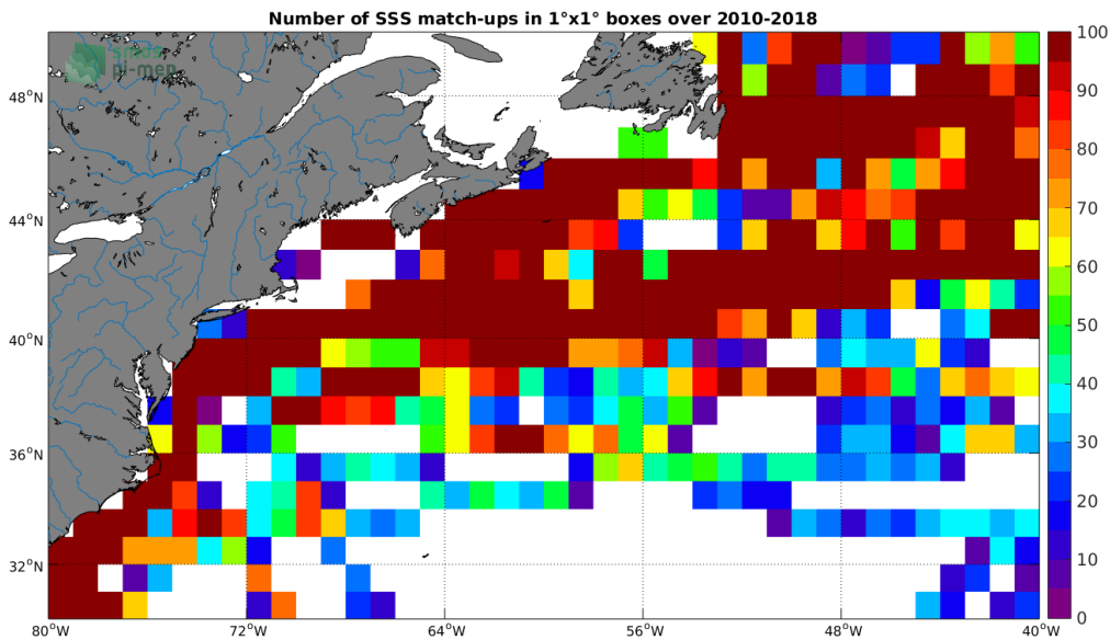
Figure 4: Number of SSS match-ups between TSG-LEGOS-DM SSS and the SMOS L3 v317 - Monthly - 25 km (CATDS-CPDC) SSS product for the Gulf Stream Pi-MEP region over 1^\circ \times 1^\circ boxes and for the full satellite product period.
