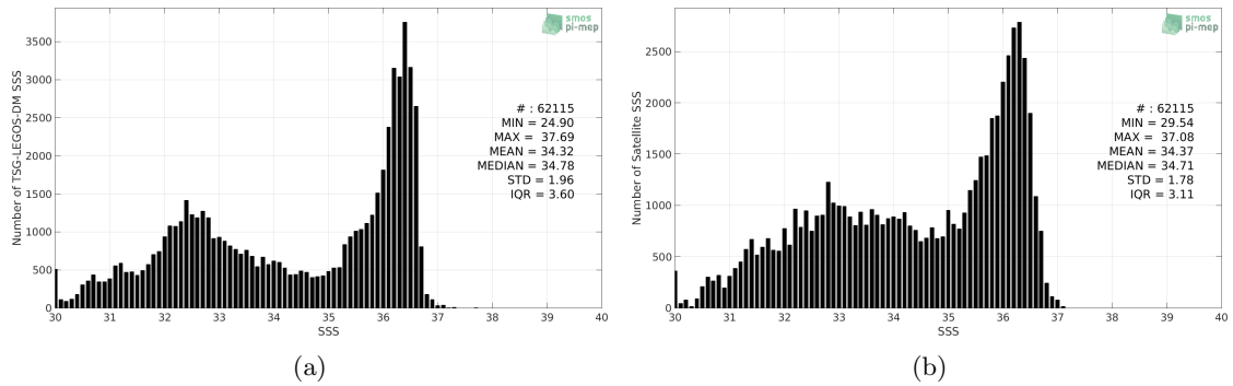
Figure 2: Histograms of SSS from TSG-LEGOS-DM (a) and SMOS L3 v317 - Monthly - 25 km (CATDS-CPDC) (b) considering all match-up pairs per bins of 0.1 over the Gulf Stream Pi-MEP region and for the full satellite product period.
