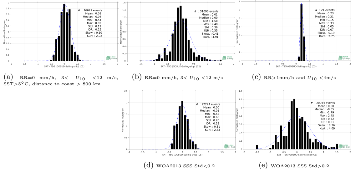
Figure 13: Normalized histogram of \Delta\text{SSS} (SMOS SSS L3 v317 - Monthly - 25 km (CATDS-CPDC) - TSG (GOSUD-Sailing-ship)) for 5 different subdatasets corresponding to: RR=0 mm/h, 3 < U_{10} < 12 m/s, SST>5°C, distance to coast > 800 km (a), RR=0 mm/h, 3 < U_{10} < 12 m/s (b), RR>1mm/h and U_{10} < 4 m/s (c), WOA2013 SSS Std<0.2 (d), WOA2013 SSS Std>0.2 (e).
