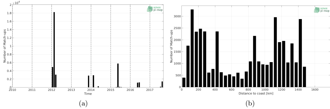
Figure 1: Number of match-ups between TSG-GOSUD-Sailing-ship and SMOS L3 v317 - Monthly - 25 km (CATDS-CPDC) SSS as a function of time (a) and as function of the distance to coast (b) over the Gulf Stream Pi-MEP region and for the full satellite product period.
