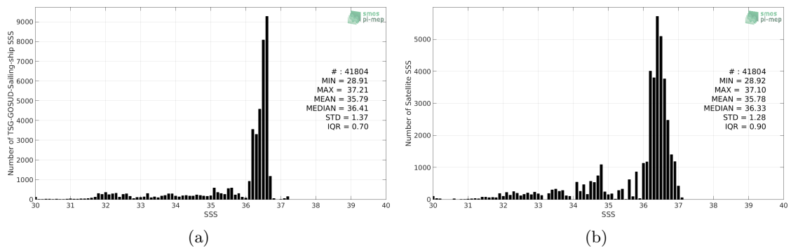
Figure 2: Histograms of SSS from TSG-GOSUD-Sailing-ship (a) and SMOS L3 v317 - Monthly - 25 km (CATDS-CPDC) (b) considering all match-up pairs per bins of 0.1 over the Gulf Stream Pi-MEP region and for the full satellite product period.
