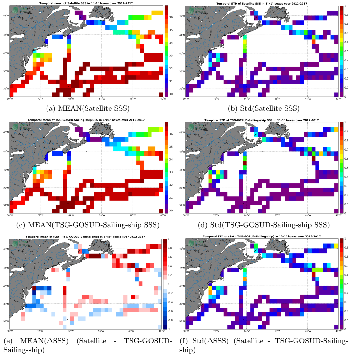
Figure 6: Temporal mean (left) and Std (right) of SSS from SMOS L3 v317 - Monthly - 25 km (CATDS-CPDC) (top), TSG-GOSUD-Sailing-ship (middle), and of \Delta SSS (Satellite - TSG-GOSUD-Sailing-ship). Only match-up pairs are used to generate these maps.
