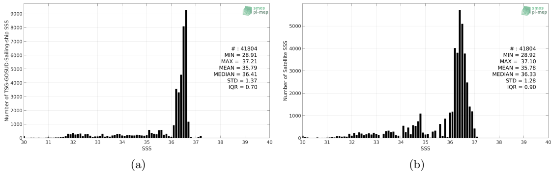
Figure 2: Histograms of SSS from TSG-GOSUD-Sailing-ship (a) and SMOS-L3-CATDS-CPDC-V317-MONTHLY-25KM (b) considering all match-up pairs per bins of 0.1 over the Gulf Stream Pi-MEP region and for the full satellite product period.
