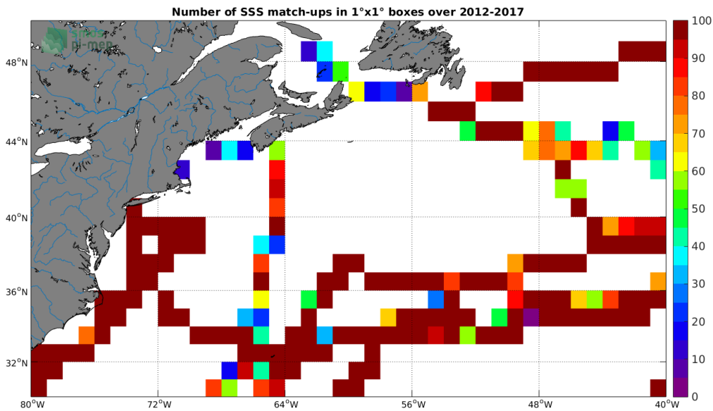
Figure 4: Number of SSS match-ups between TSG-GOSUD-Sailing-ship SSS and the SMOS-L3-CATDS-CPDC-V317-MONTHLY-25KM SSS product for the Gulf Stream Pi-MEP region over 1^\circ \times 1^\circ boxes and for the full satellite product period.
