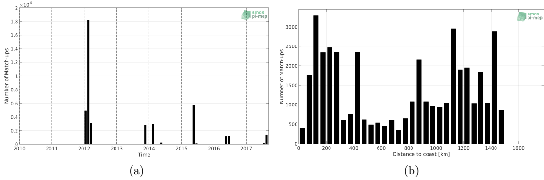
Figure 1: Number of match-ups between TSG-GOSUD-Sailing-ship and SMOS-L3-CATDS-CPDC-V317-MONTHLY-25KM SSS as a function of time (a) and as function of the distance to coast (b) over the Gulf Stream Pi-MEP region and for the full satellite product period.
