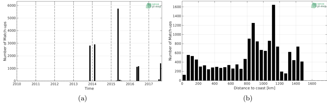
Figure 1: Number of match-ups between TSG-GOSUD-Sailing-ship and SMOS-L3-CATDS-CPDC-V317-MONTHLY-25KM SSS as a function of time (a) and as function of the distance to coast (b) over the Gulf Stream Pi-MEP region and for the full satellite product period.
