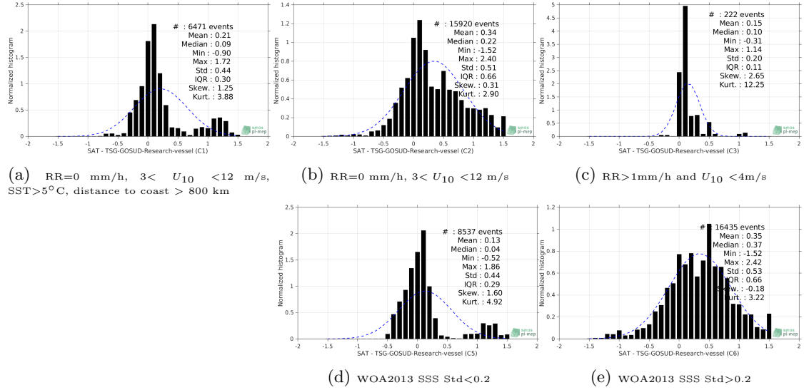
Figure 13: Normalized histogram of \Delta\text{SSS} (SMOS-L3-CATDS-CPDC-V317-MONTHLY-25KM - TSG-GOSUD-Research-vessel) for 5 different subdatasets corresponding to: RR=0 mm/h, 3 < U_{10} < 12 m/s, SST>5°C, distance to coast > 800 km (a), RR=0 mm/h, 3 < U_{10} < 12 m/s (b), RR>1mm/h and U_{10} < 4 m/s (c), WOA2013 SSS Std<0.2 (d), WOA2013 SSS Std>0.2 (e).
