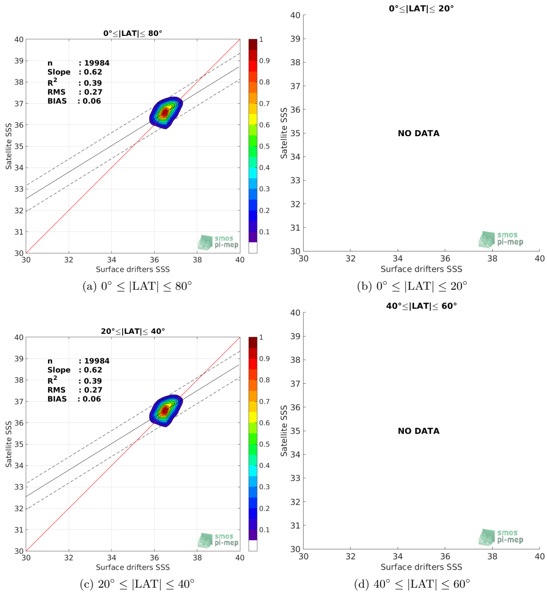
Figure 8: Contour maps of the concentration of SMOS-L3-CATDS-CPDC-V317-MONTHLY-25KM SSS (y-axis) versus Surface drifters SSS (x-axis) at match-up pairs for different latitude bands. For each plot, the red line shows x=y . The black thin and dashed lines indicate a linear fit through the data cloud and the \pm 95\% confidence levels, respectively. The number match-up pairs n , the slope and R^2 coefficient of the linear fit, the root mean square (RMS) and the mean bias between satellite and in situ data are indicated for each latitude band in each plots.
