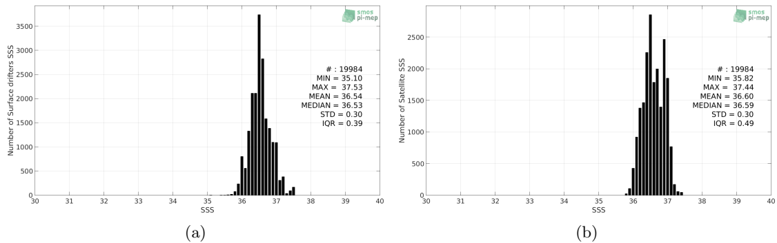
Figure 2: Histograms of SSS from Surface drifters (a) and SMOS-L3-CATDS-CPDC-V317-MONTHLY-25KM (b) considering all match-up pairs per bins of 0.1 over the Gulf Stream Pi-MEP region and for the full satellite product period.
