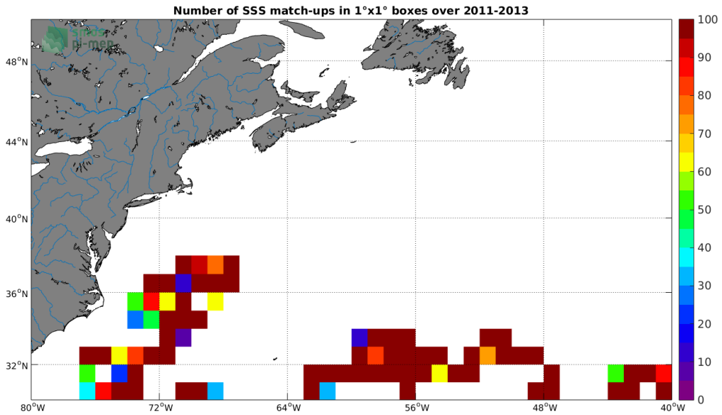
Figure 3: Number of SSS match-ups between Surface drifters SSS and the SMOS-L3-CATDS-CPDC-V317-MONTHLY-25KM SSS product for the Gulf Stream Pi-MEP region over 1°x1° boxes and for the full satellite product period.
