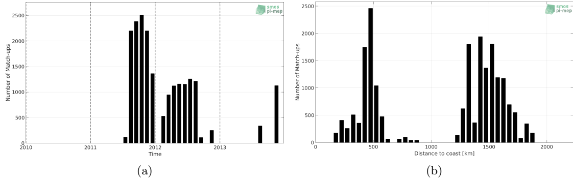
Figure 1: Number of match-ups between Surface drifters and SMOS-L3-CATDS-CPDC-V317-MONTHLY-25KM SSS as a function of time (a) and as function of the distance to coast (b) over the Gulf Stream Pi-MEP region and for the full satellite product period.
