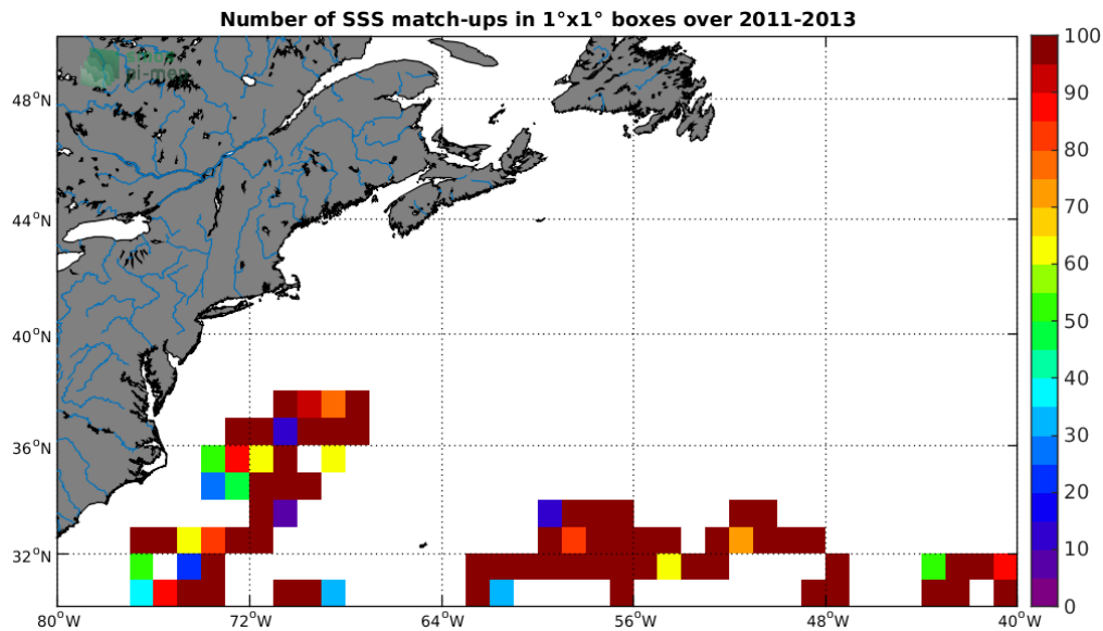
Figure 3: Number of SSS match-ups between Surface drifters SSS and the SMOS-L3-CATDS-CPDC-V317-MONTHLY-25KM SSS product for the Gulf Stream Pi-MEP region over 1^\circ \times 1^\circ boxes and for the full satellite product period.
