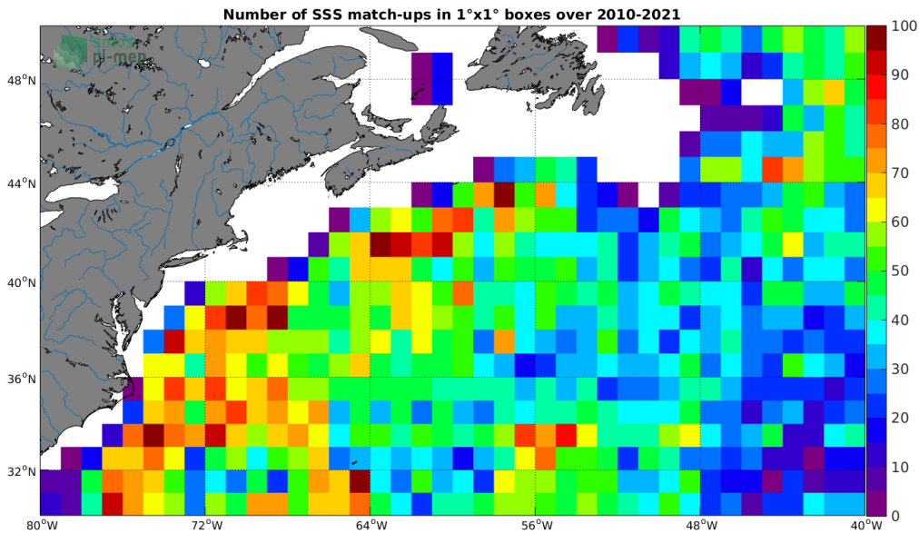
Figure 4: Number of SSS match-ups between Argo SSS and the SMOS SSS L3 v317 - Monthly - 25 km (CATDS-CPDC) SSS product for the Gulf Stream Pi-MEP region over 1^\circ \times 1^\circ boxes and for the full satellite product period.
