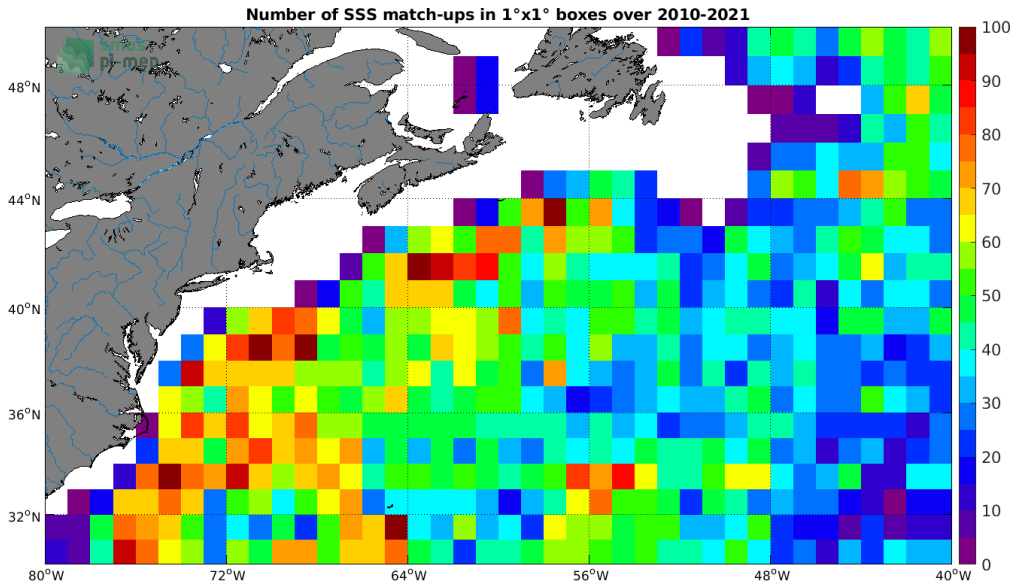
Figure 4: Number of SSS match-ups between Argo SSS and the SMOS SSS L3 v317 - Monthly - 25 km (CATDS-CPDC) SSS product for the Gulf Stream Pi-MEP region over 1^{\circ} \times 1^{\circ} boxes and for the full satellite product period.
