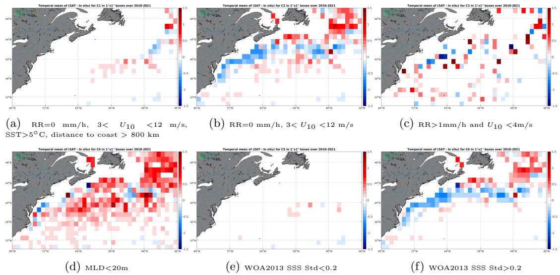
Figure 12: Temporal mean gridded over spatial boxes of size 1°x1° of \Delta SSS (SMOS SSS L3 v317 - Monthly - 25 km (CATDS-CPDC) - Argo) for 6 different subdatasets corresponding to:RR=0 mm/h, 3 < U_{10} < 12 m/s, SST > 5°C, distance to coast > 800 km (a), RR=0 mm/h, 3 < U_{10} < 12 m/s (b), RR > 1mm/h and U_{10} < 4m/s (c),MLD < 20m (d),WOA2013 SSS Std < 0.2 (e),WOA2013 SSS Std > 0.2 (f).
