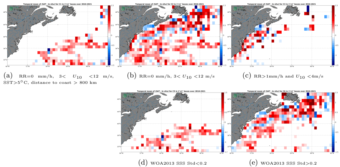
Figure 12: Temporal mean gridded over spatial boxes of size 1^\circ \times 1^\circ of \Delta SSS (SMOS SSS L3 v317 - 10 Days - 25 km (CATDS-CPDC) - TSG (SAMOS)) for 5 different subdatasets corresponding to:RR=0 mm/h, 3 < U_{10} < 12 m/s, SST >5^\circ C, distance to coast > 800 km (a), RR=0 mm/h, 3 < U_{10} < 12 m/s (b), RR >1 mm/h and U_{10} < 4 m/s (c), WOA2013 SSS Std <0.2 (d), WOA2013 SSS Std >0.2 (e).
