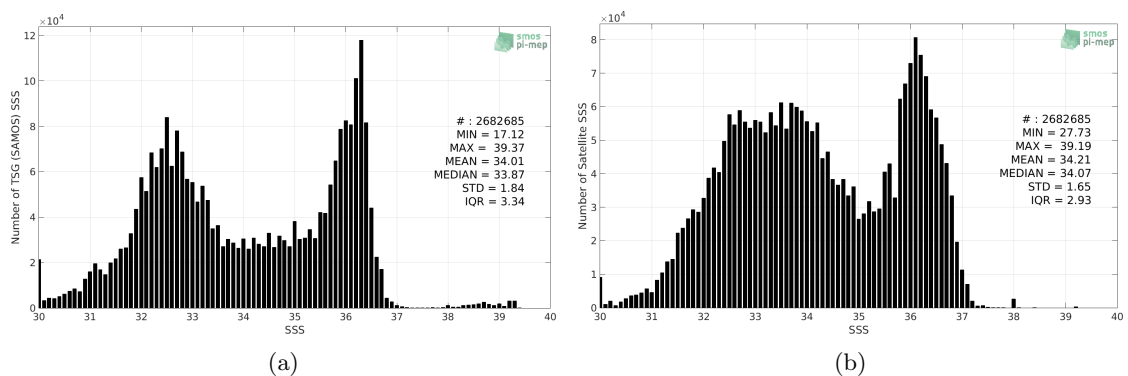
Figure 2: Histograms of SSS from TSG (SAMOS) (a) and SMOS SSS L3 v317 - 10 Days - 25 km (CATDS-CPDC) (b) considering all match-up pairs per bins of 0.1 over the Gulf Stream Pi-MEP region and for the full satellite product period.
