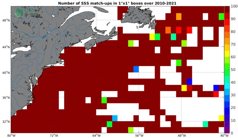
Figure 4: Number of SSS match-ups between TSG (SAMOS) SSS and the SMOS SSS L3 v317 - 10 Days - 25 km (CATDS-CPDC) SSS product for the Gulf Stream Pi-MEP region over 1^\circ \times 1^\circ boxes and for the full satellite product period.
