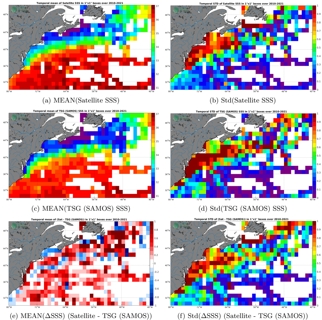
Figure 6: Temporal mean (left) and Std (right) of SSS from SMOS SSS L3 v317 - 10 Days - 25 km (CATDS-CPDC) (top), TSG (SAMOS) (middle), and of \Delta SSS (Satellite - TSG (SAMOS)). Only match-up pairs are used to generate these maps.
