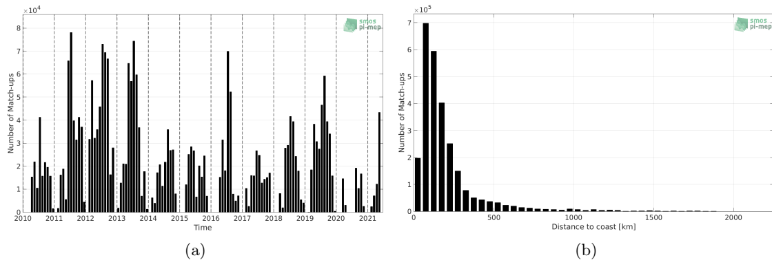
Figure 1: Number of match-ups between TSG (SAMOS) and SMOS SSS L3 v317 - 10 Days - 25 km (CATDS-CPDC) SSS as a function of time (a) and as function of the distance to coast (b) over the Gulf Stream Pi-MEP region and for the full satellite product period.
