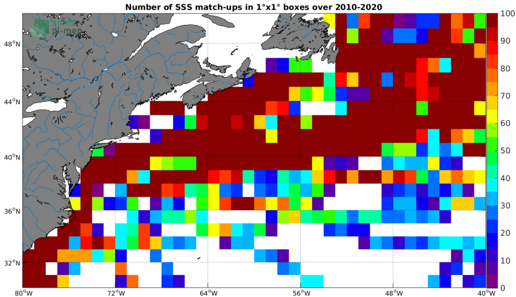
Figure 4: Number of SSS match-ups between TSG (LEGOS-DM) SSS and the SMOS SSS L3 v317 - 10 Days - 25 km (CATDS-CPDC) SSS product for the Gulf Stream Pi-MEP region over 1^\circ \times 1^\circ boxes and for the full satellite product period.
