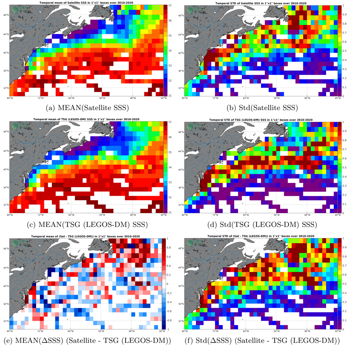
Figure 6: Temporal mean (left) and Std (right) of SSS from SMOS SSS L3 v317 - 10 Days - 25 km (CATDS-CPDC) (top), TSG (LEGOS-DM) (middle), and of \Delta SSS (Satellite - TSG (LEGOS-DM)). Only match-up pairs are used to generate these maps.
