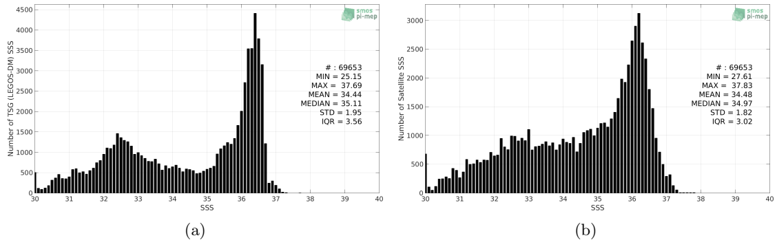
Figure 2: Histograms of SSS from TSG (LEGOS-DM) (a) and SMOS SSS L3 v317 - 10 Days - 25 km (CATDS-CPDC) (b) considering all match-up pairs per bins of 0.1 over the Gulf Stream Pi-MEP region and for the full satellite product period.
