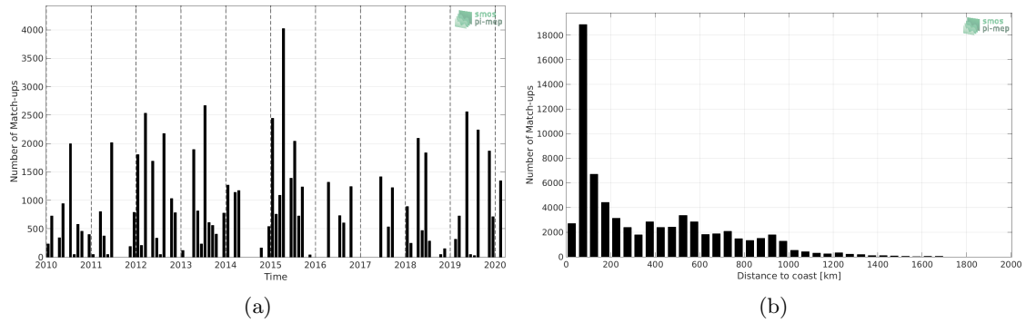
Figure 1: Number of match-ups between TSG (LEGOS-DM) and SMOS SSS L3 v317 - 10 Days - 25 km (CATDS-CPDC) SSS as a function of time (a) and as function of the distance to coast (b) over the Gulf Stream Pi-MEP region and for the full satellite product period.
