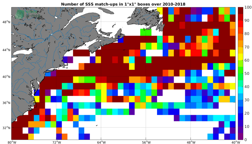
Figure 4: Number of SSS match-ups between TSG-LEGOS-DM SSS and the SMOS L3 v317 - 10 Days - 25 km (CATDS-CPDC) SSS product for the Gulf Stream Pi-MEP region over 1^\circ \times 1^\circ boxes and for the full satellite product period.
