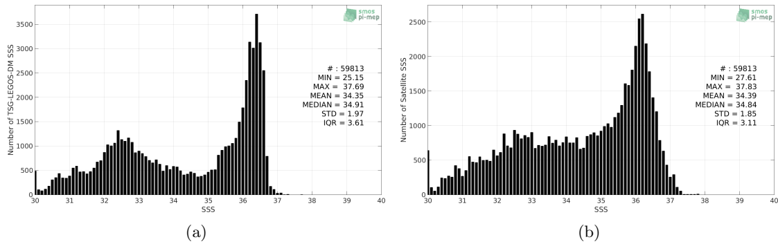
Figure 2: Histograms of SSS from TSG-LEGOS-DM (a) and SMOS L3 v317 - 10 Days - 25 km (CATDS-CPDC) (b) considering all match-up pairs per bins of 0.1 over the Gulf Stream Pi-MEP region and for the full satellite product period.
