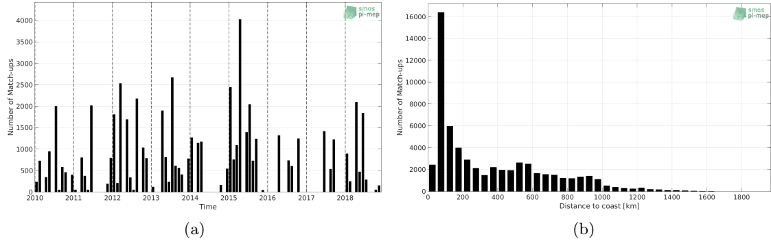
Figure 1: Number of match-ups between TSG-LEGOS-DM and SMOS L3 v317 - 10 Days - 25 km (CATDS-CPDC) SSS as a function of time (a) and as function of the distance to coast (b) over the Gulf Stream Pi-MEP region and for the full satellite product period.
