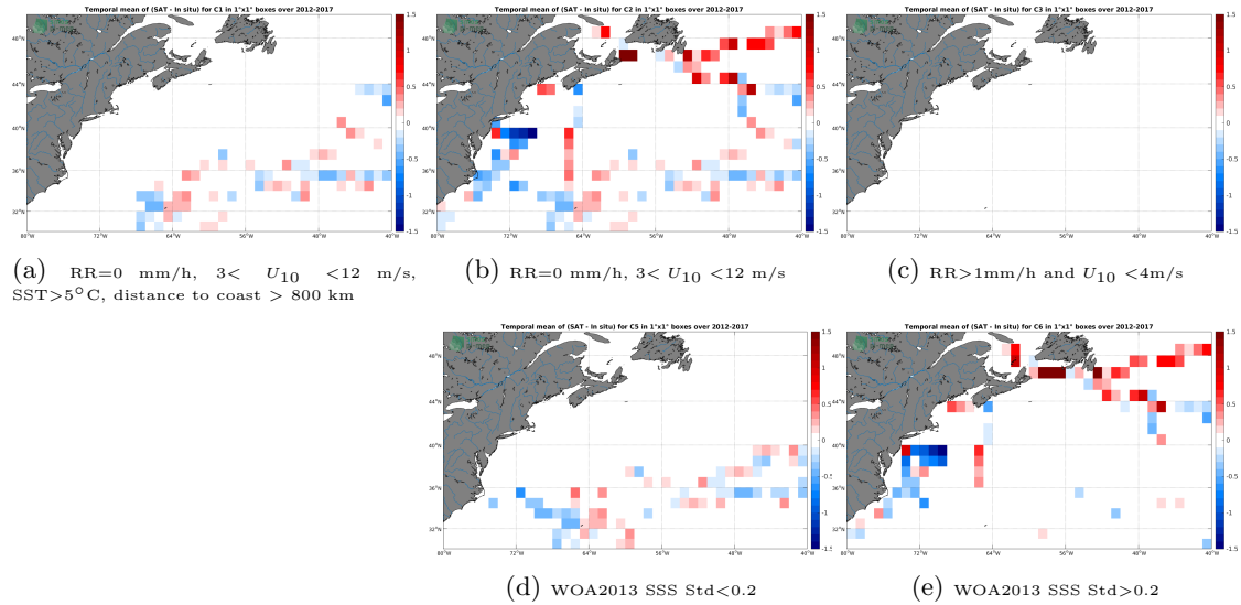
Figure 12: Temporal mean gridded over spatial boxes of size 1^{\circ}\times 1^{\circ} of \Delta SSS (SMOS L3 v317 - 10 Days - 25 km (CATDS-CPDC) - TSG-GOSUD-Sailing-ship) for 5 different subdatasets corresponding to:RR=0 mm/h, 3 < U_{10} < 12 m/s, SST >5^{\circ}\text{C} , distance to coast > 800 km (a), RR=0 mm/h, 3 < U_{10} < 12 m/s (b), RR >1 mm/h and U_{10} < 4 m/s (c), WOA2013 SSS Std <0.2 (d), WOA2013 SSS Std >0.2 (e).
