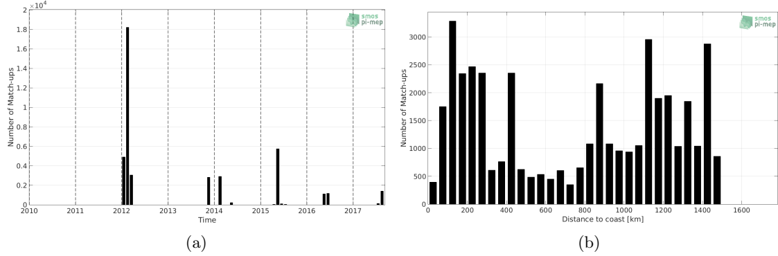
Figure 1: Number of match-ups between TSG-GOSUD-Sailing-ship and SMOS L3 v317 - 10 Days - 25 km (CATDS-CPDC) SSS as a function of time (a) and as function of the distance to coast (b) over the Gulf Stream Pi-MEP region and for the full satellite product period.
