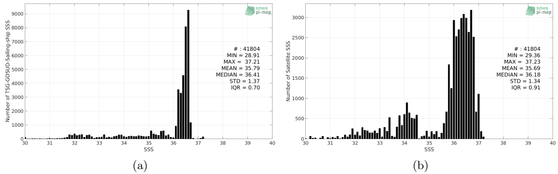
Figure 2: Histograms of SSS from TSG-GOSUD-Sailing-ship (a) and SMOS L3 v317 - 10 Days - 25 km (CATDS-CPDC) (b) considering all match-up pairs per bins of 0.1 over the Gulf Stream Pi-MEP region and for the full satellite product period.
