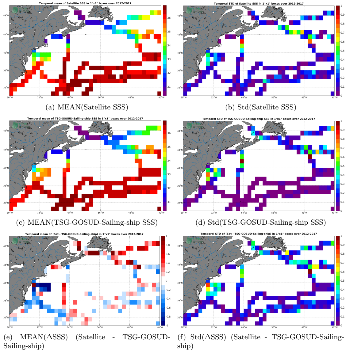
Figure 6: Temporal mean (left) and Std (right) of SSS from SMOS L3 v317 - 10 Days - 25 km (CATDS-CPDC) (top), TSG-GOSUD-Sailing-ship (middle), and of \Delta SSS (Satellite - TSG-GOSUD-Sailing-ship). Only match-up pairs are used to generate these maps.
